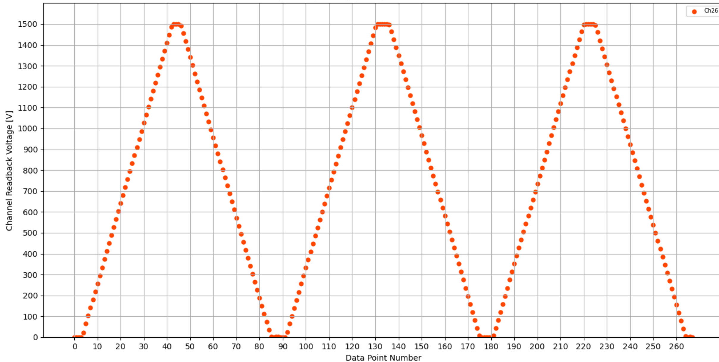
Voltage Ramp Test (Python) Bd #173, Slot #9, Ch #26
