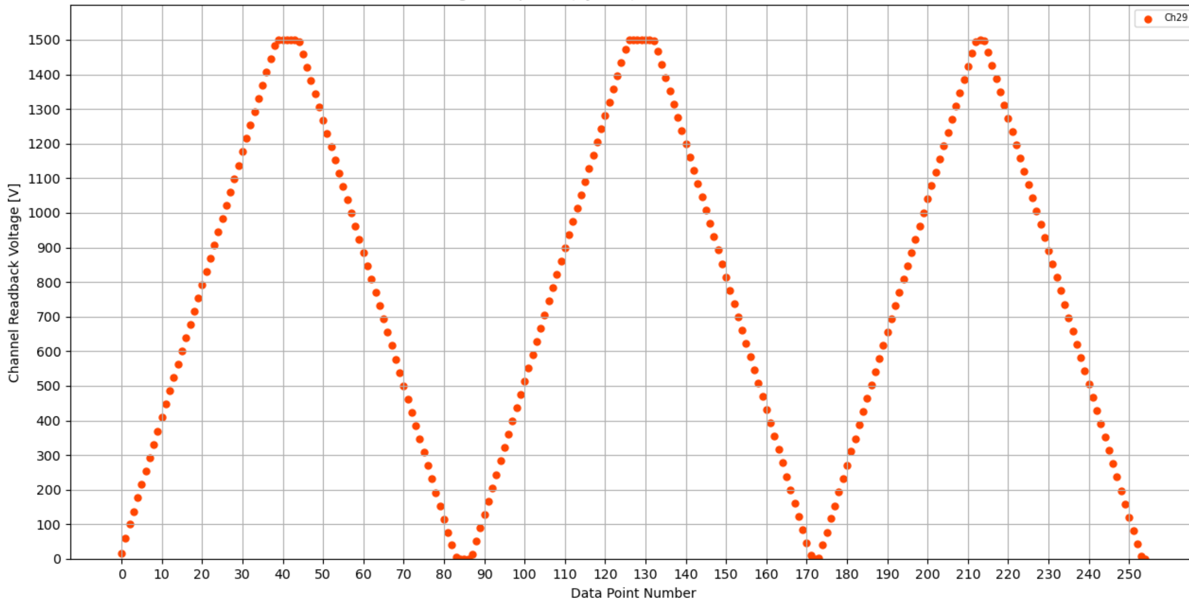
Voltage Ramp Test (Python) Bd #173, Slot #9, Ch #29
