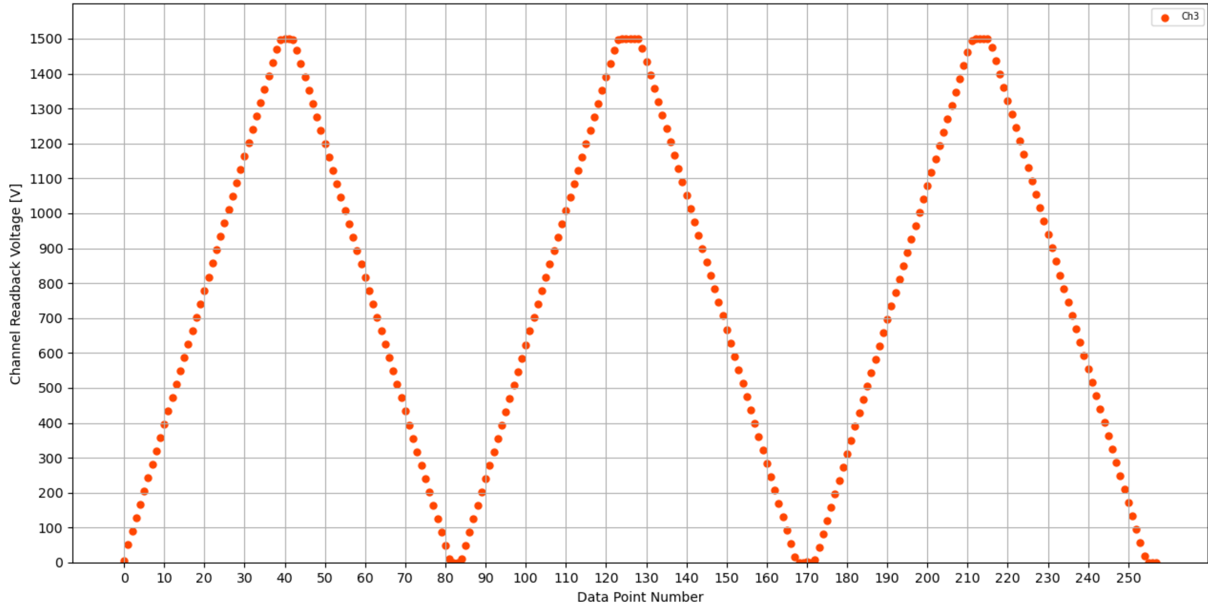
Voltage Ramp Test (Python) Bd #173, Slot #9, Ch #3
