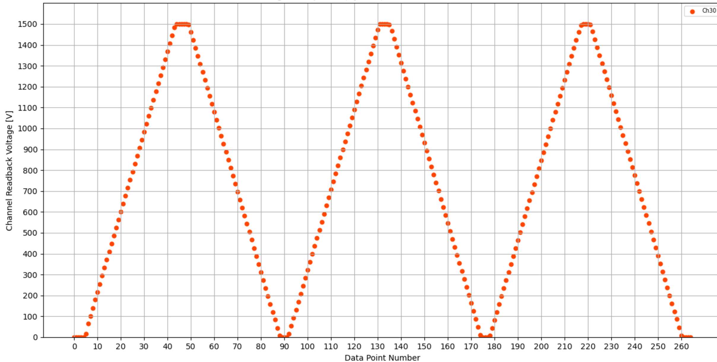
Voltage Ramp Test (Python) Bd #173, Slot #9, Ch #30
