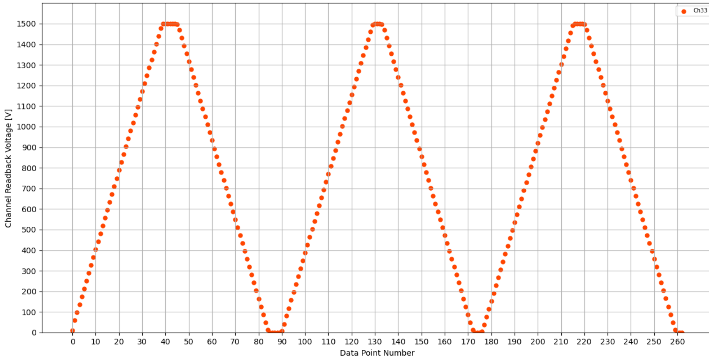
Voltage Ramp Test (Python) Bd #173, Slot #9, Ch #33
