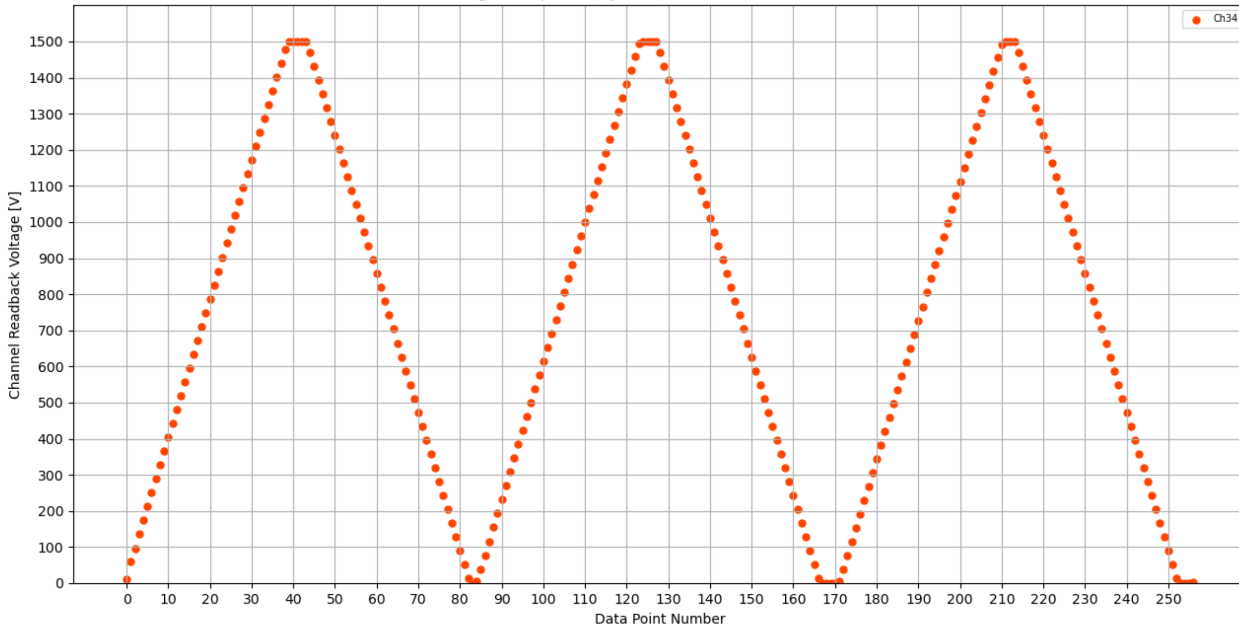
Voltage Ramp Test (Python) Bd #173, Slot #9, Ch #34
