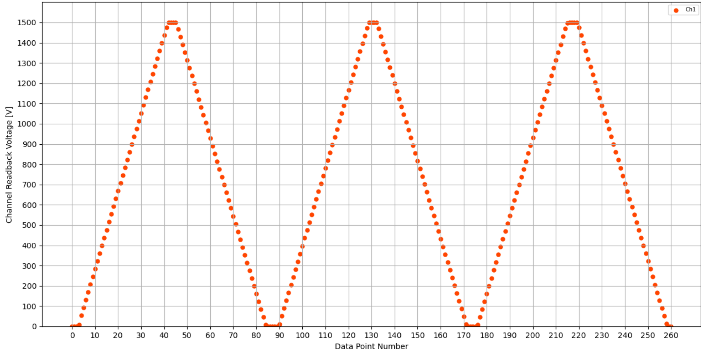
Voltage Ramp Test (Python) Bd #184, Slot #2, Ch #1
