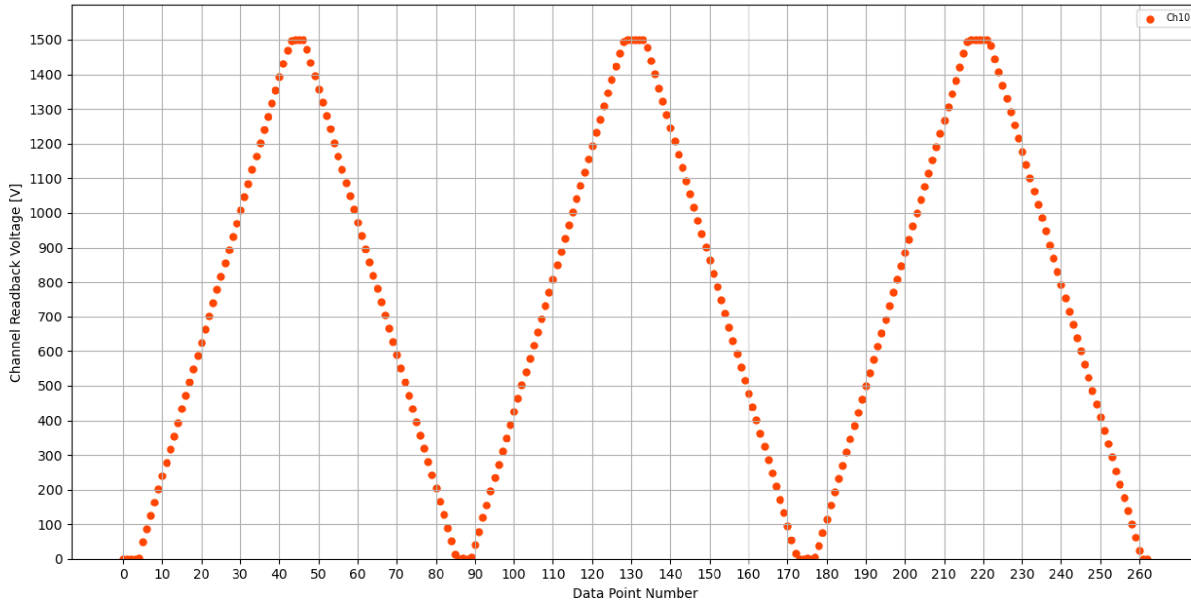
Voltage Ramp Test (Python) Bd #184, Slot #2, Ch #10
