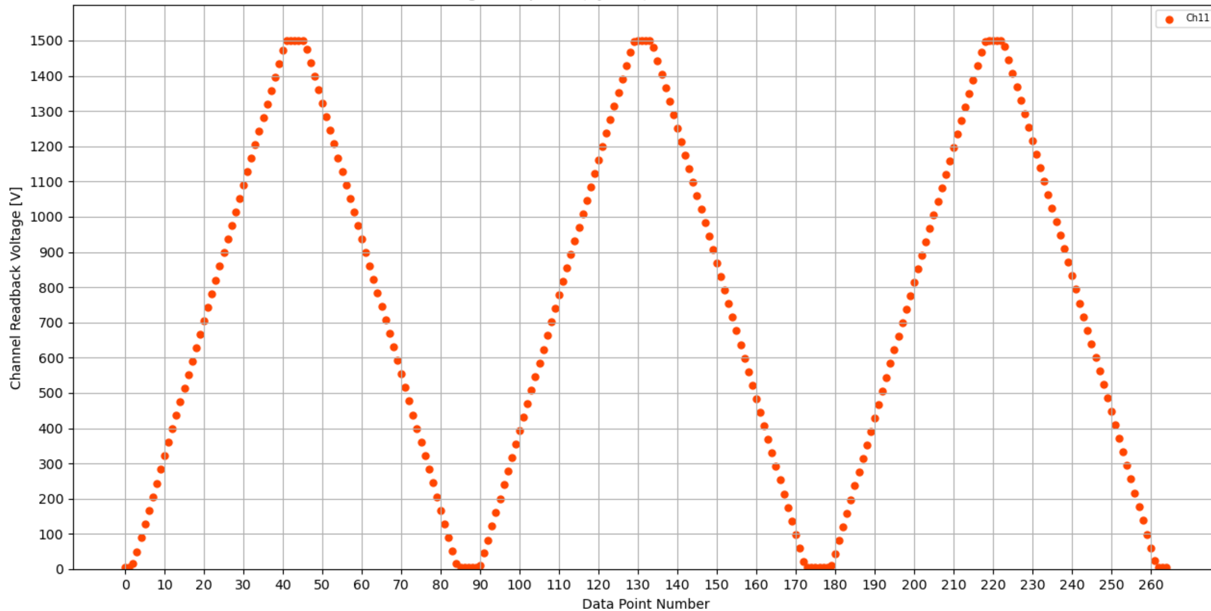
Voltage Ramp Test (Python) Bd #184, Slot #2, Ch #11
