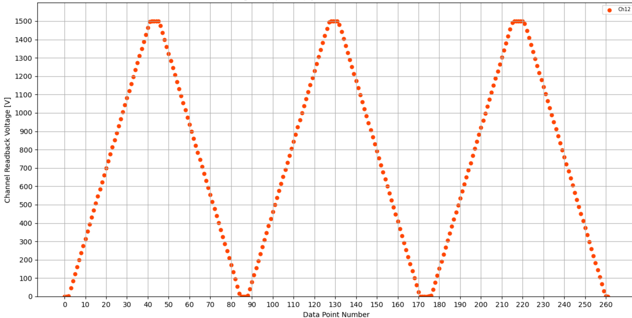
Voltage Ramp Test (Python) Bd #184, Slot #2, Ch #12
