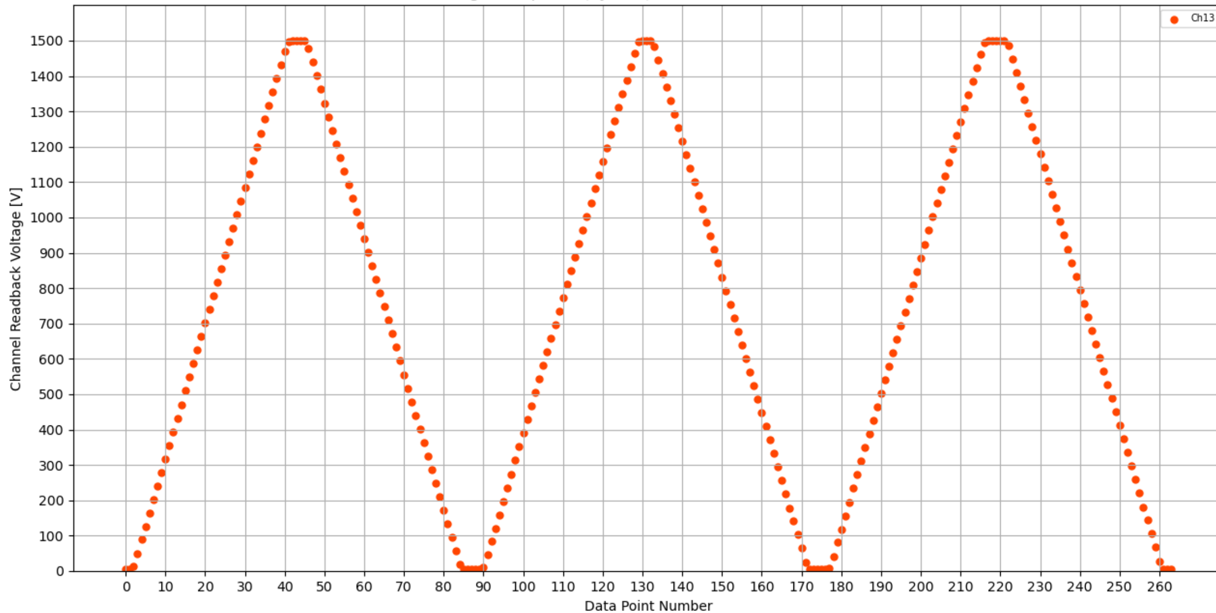
Voltage Ramp Test (Python) Bd #184, Slot #2, Ch #13
