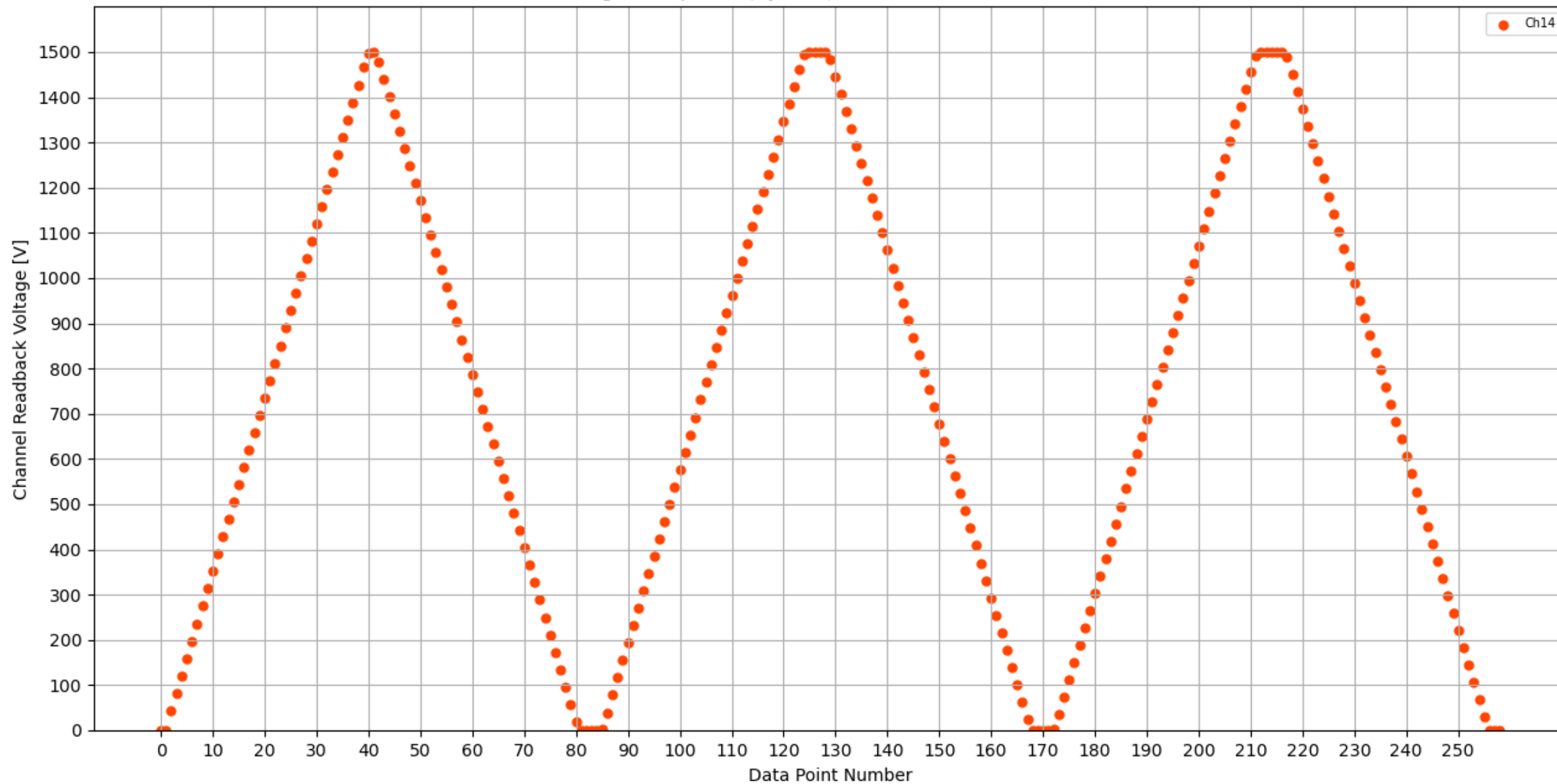
Voltage Ramp Test (Python) Bd #184, Slot #2, Ch #14
