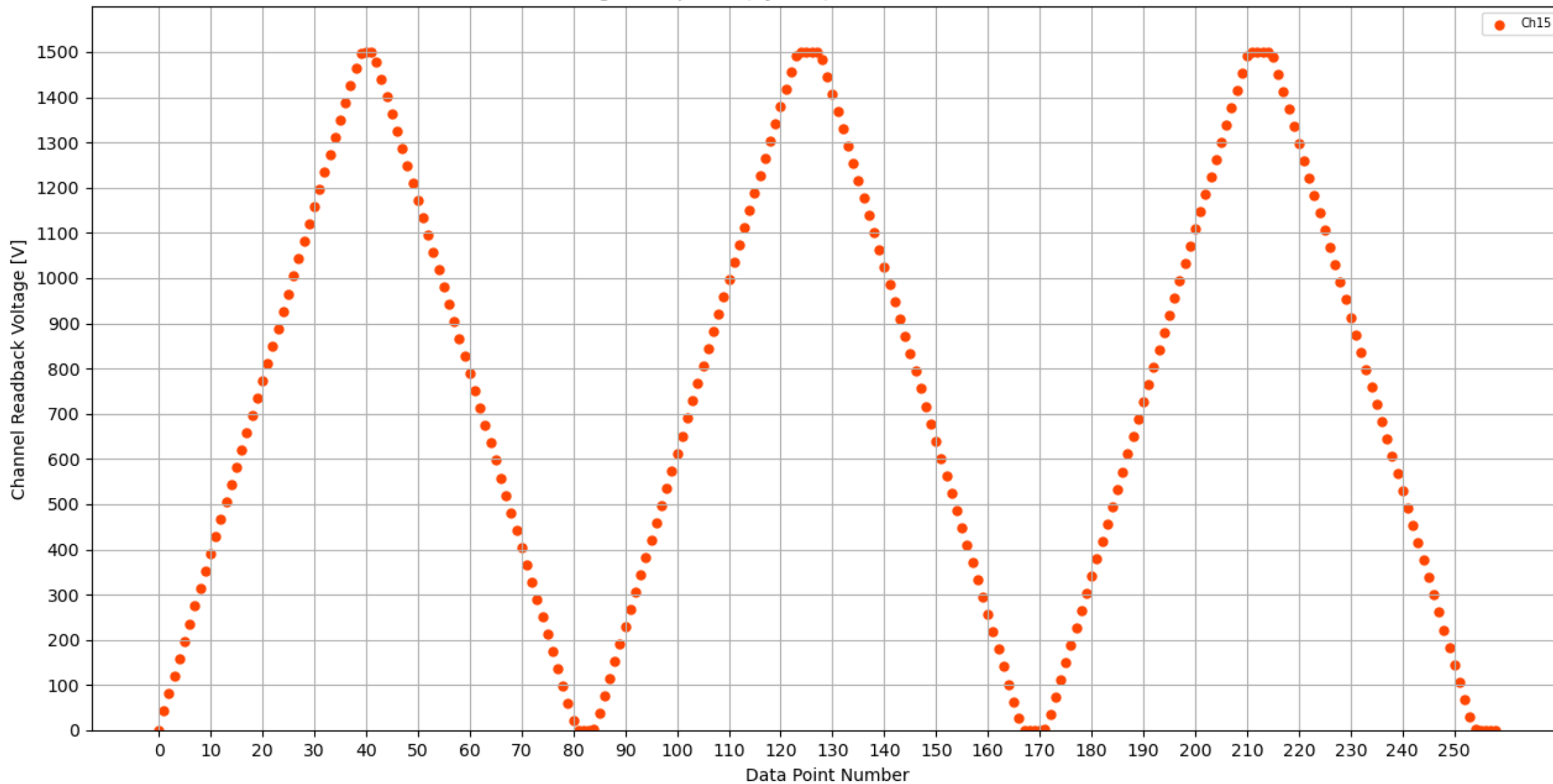
Voltage Ramp Test (Python) Bd #184, Slot #2, Ch #15
