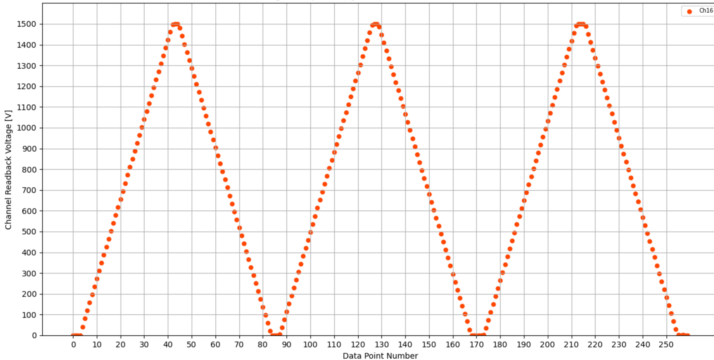
Voltage Ramp Test (Python) Bd #184, Slot #2, Ch #16
