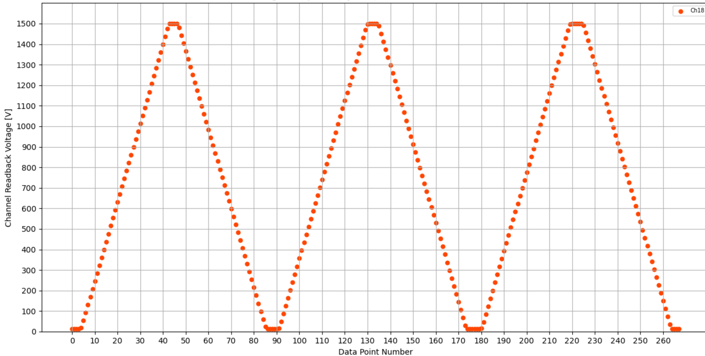
Voltage Ramp Test (Python) Bd #184, Slot #2, Ch #18
