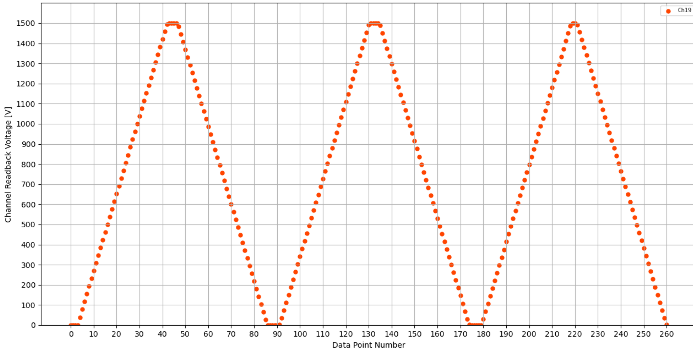
Voltage Ramp Test (Python) Bd #184, Slot #2, Ch #19
