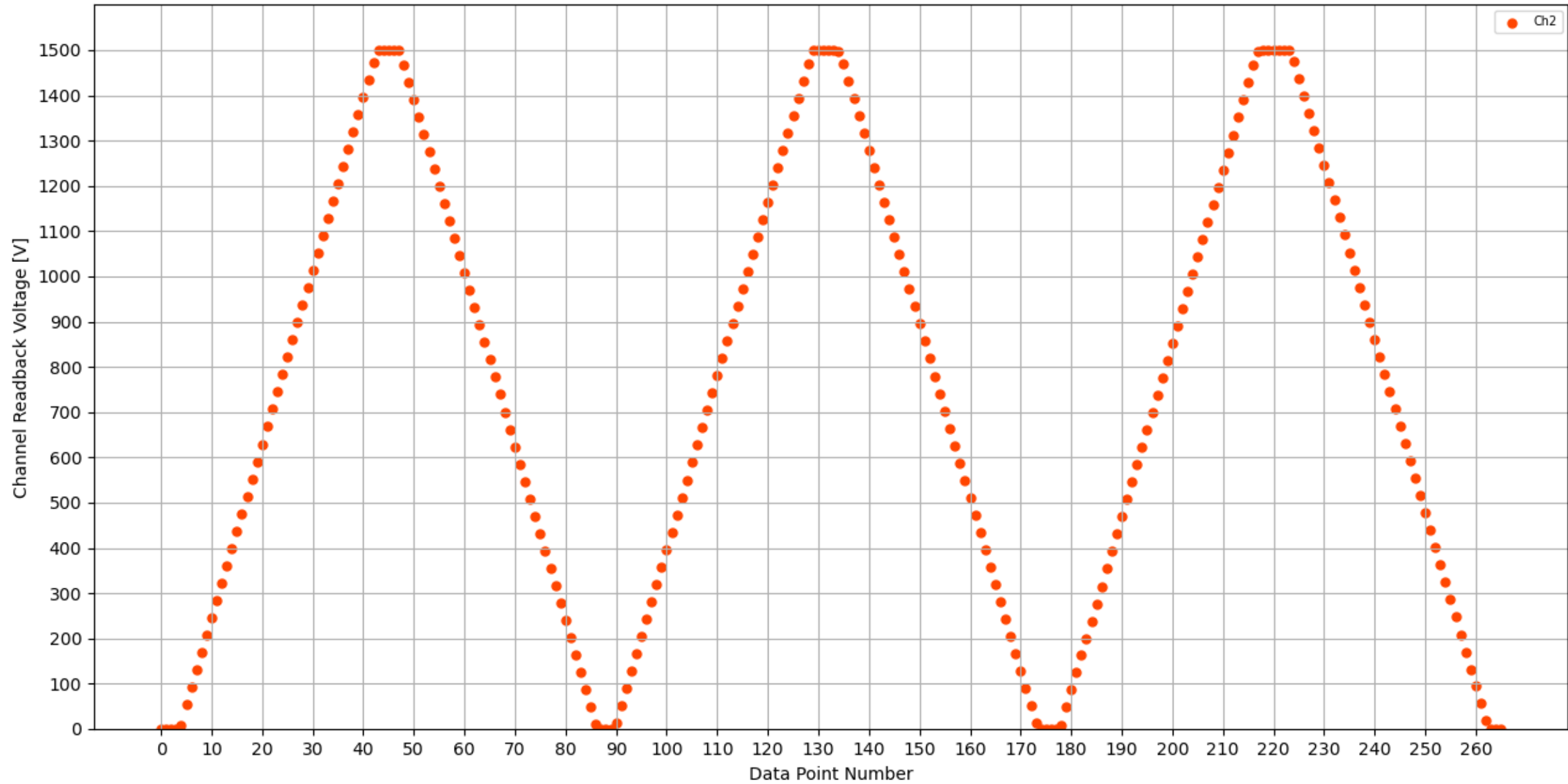
Voltage Ramp Test (Python) Bd #184, Slot #2, Ch #2
