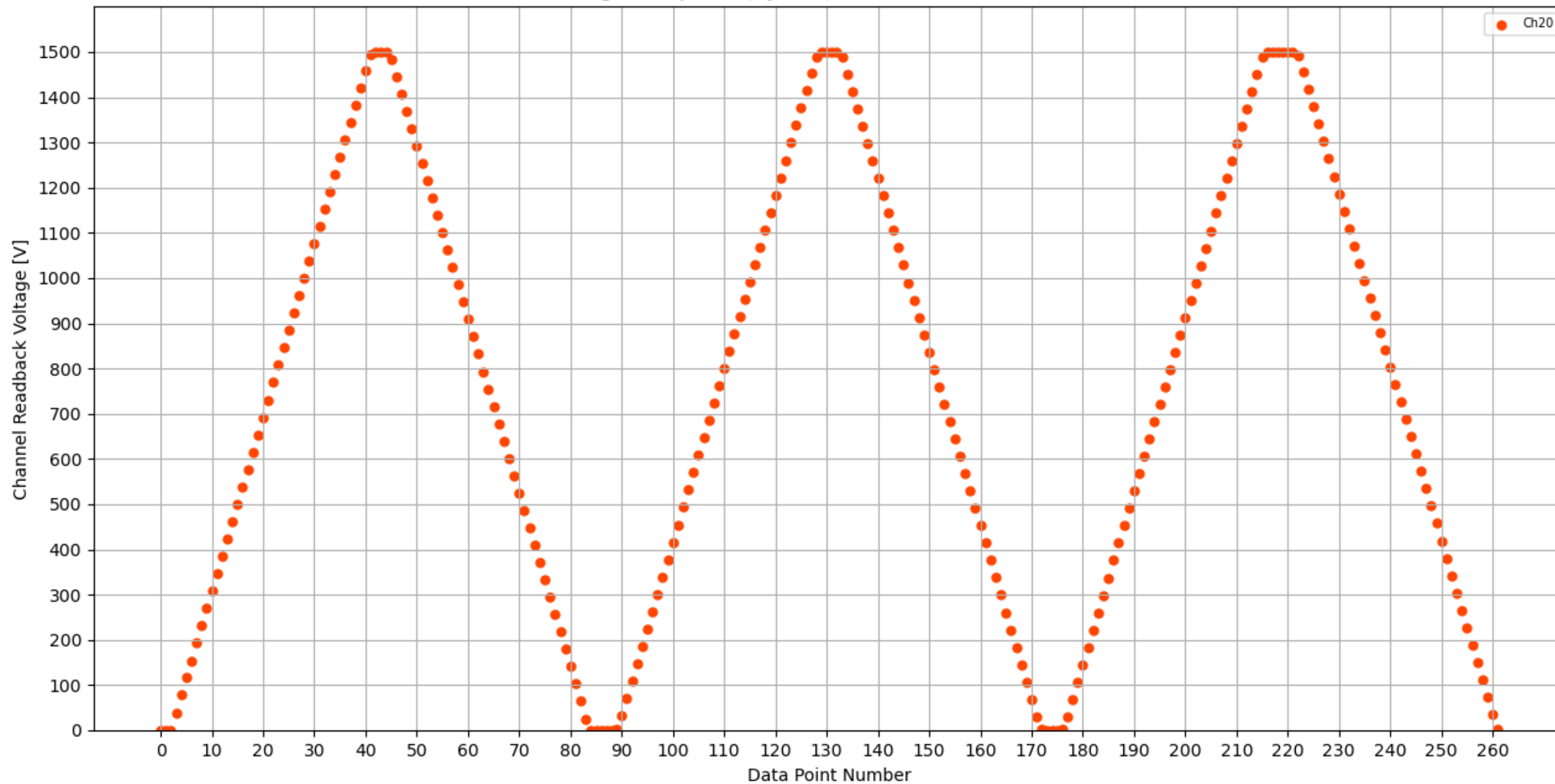
Voltage Ramp Test (Python) Bd #184, Slot #2, Ch #20
