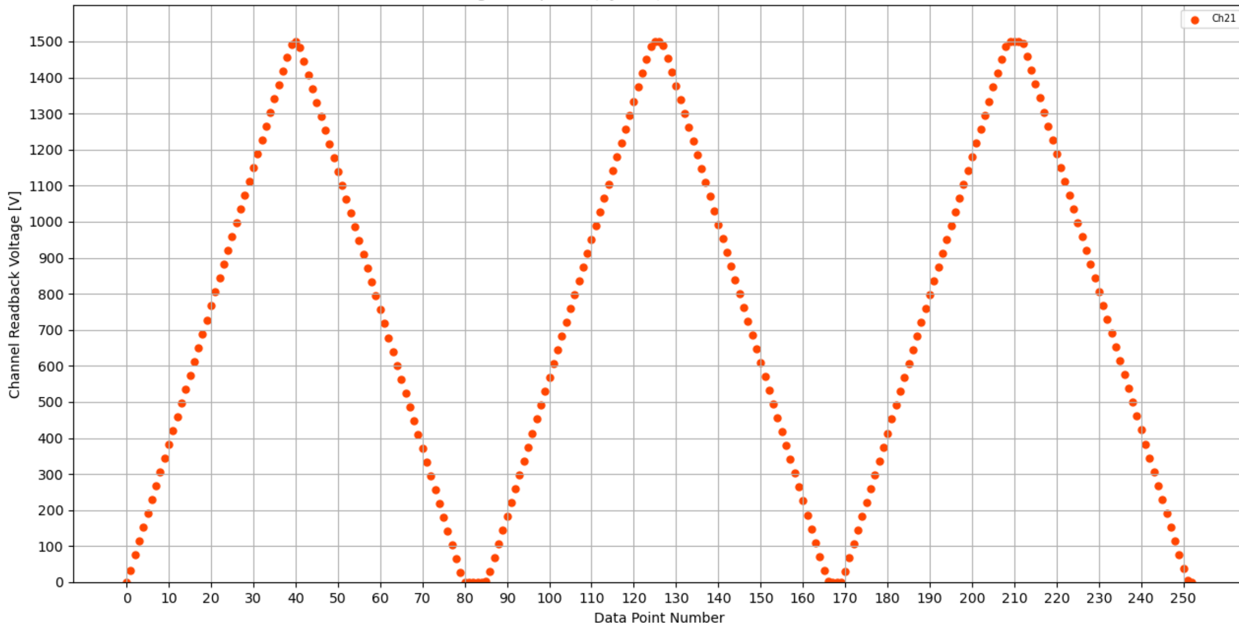
Voltage Ramp Test (Python) Bd #184, Slot #2, Ch #21
