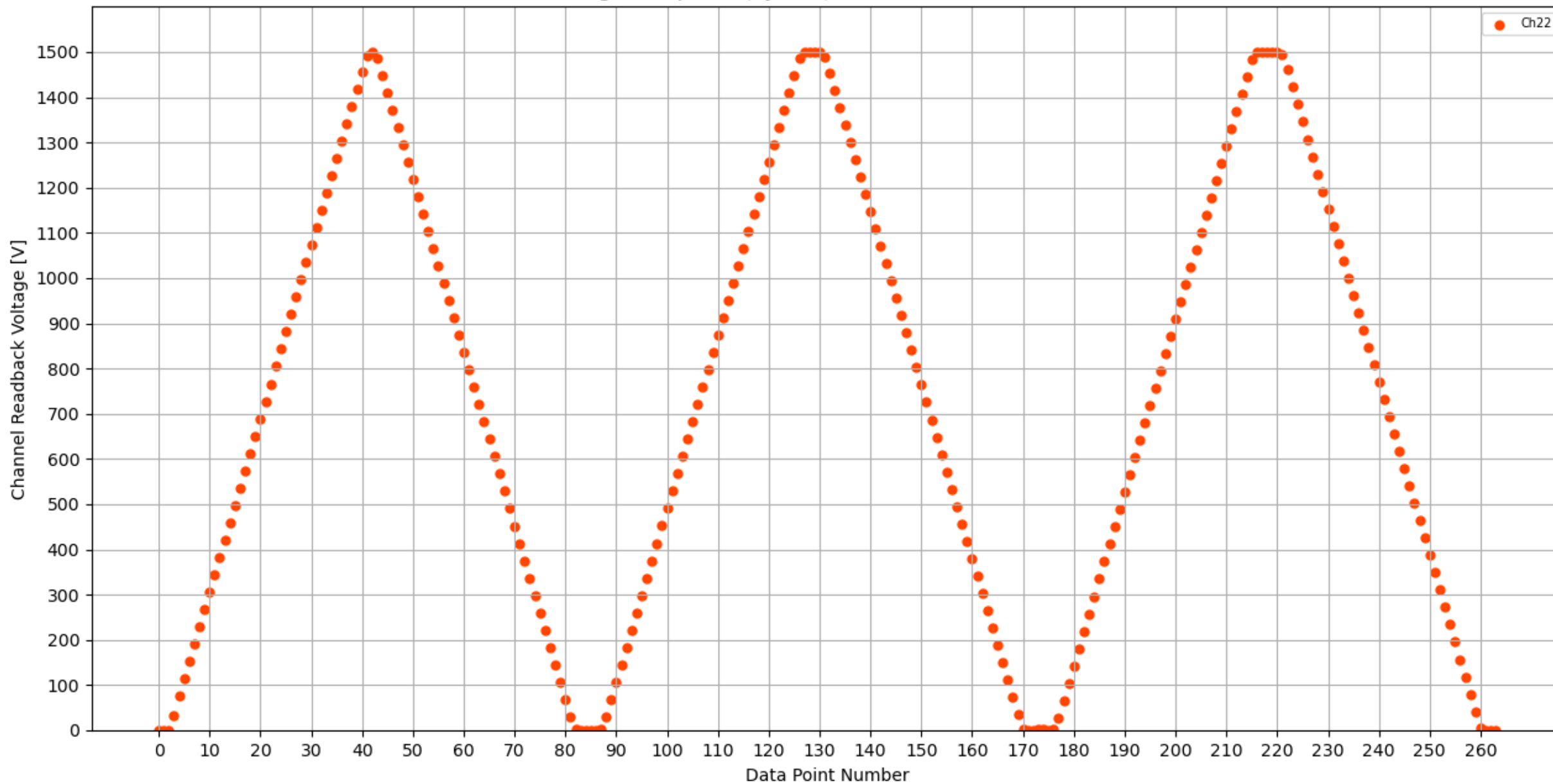
Voltage Ramp Test (Python) Bd #184, Slot #2, Ch #22
