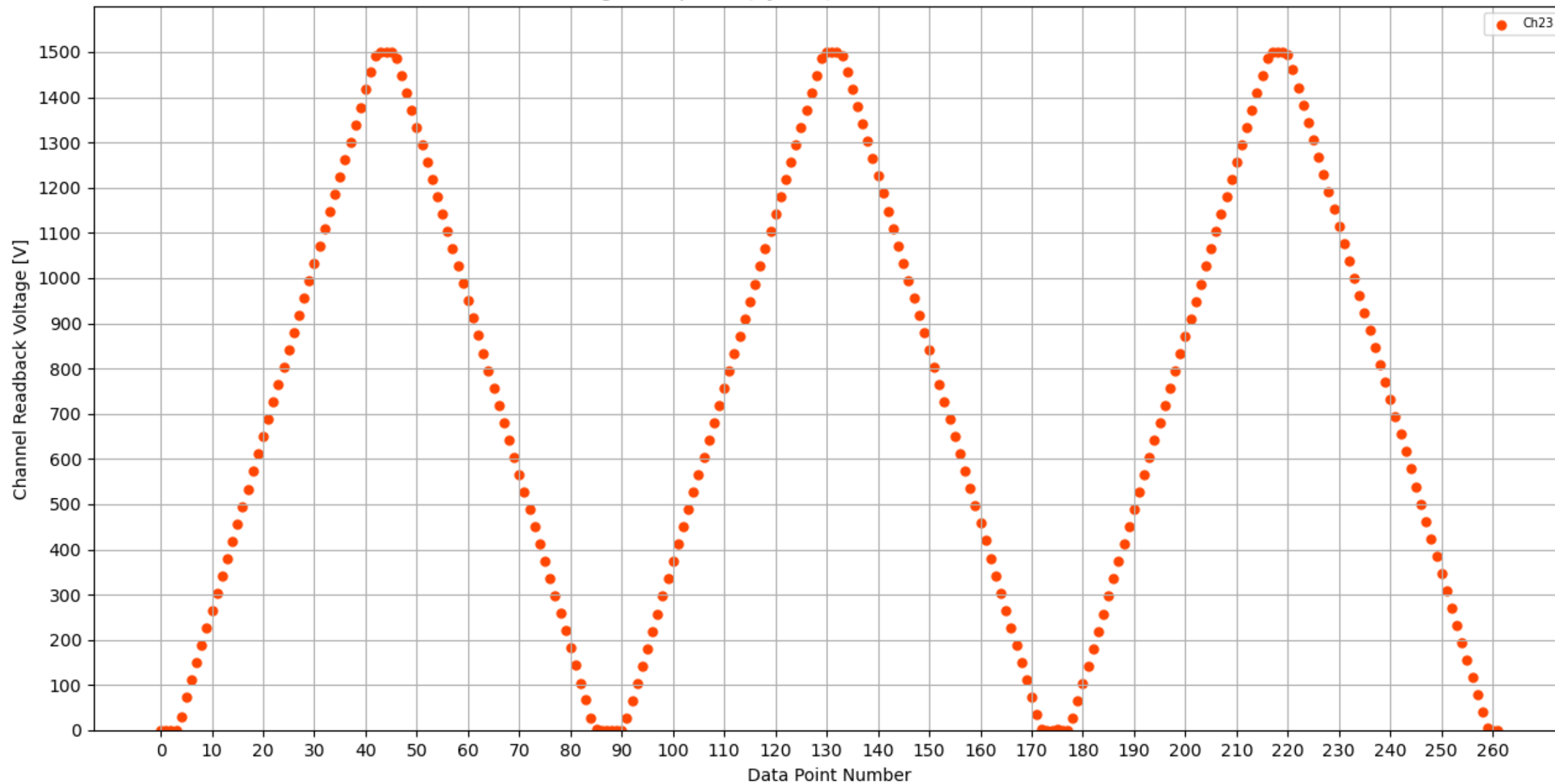
Voltage Ramp Test (Python) Bd #184, Slot #2, Ch #23
