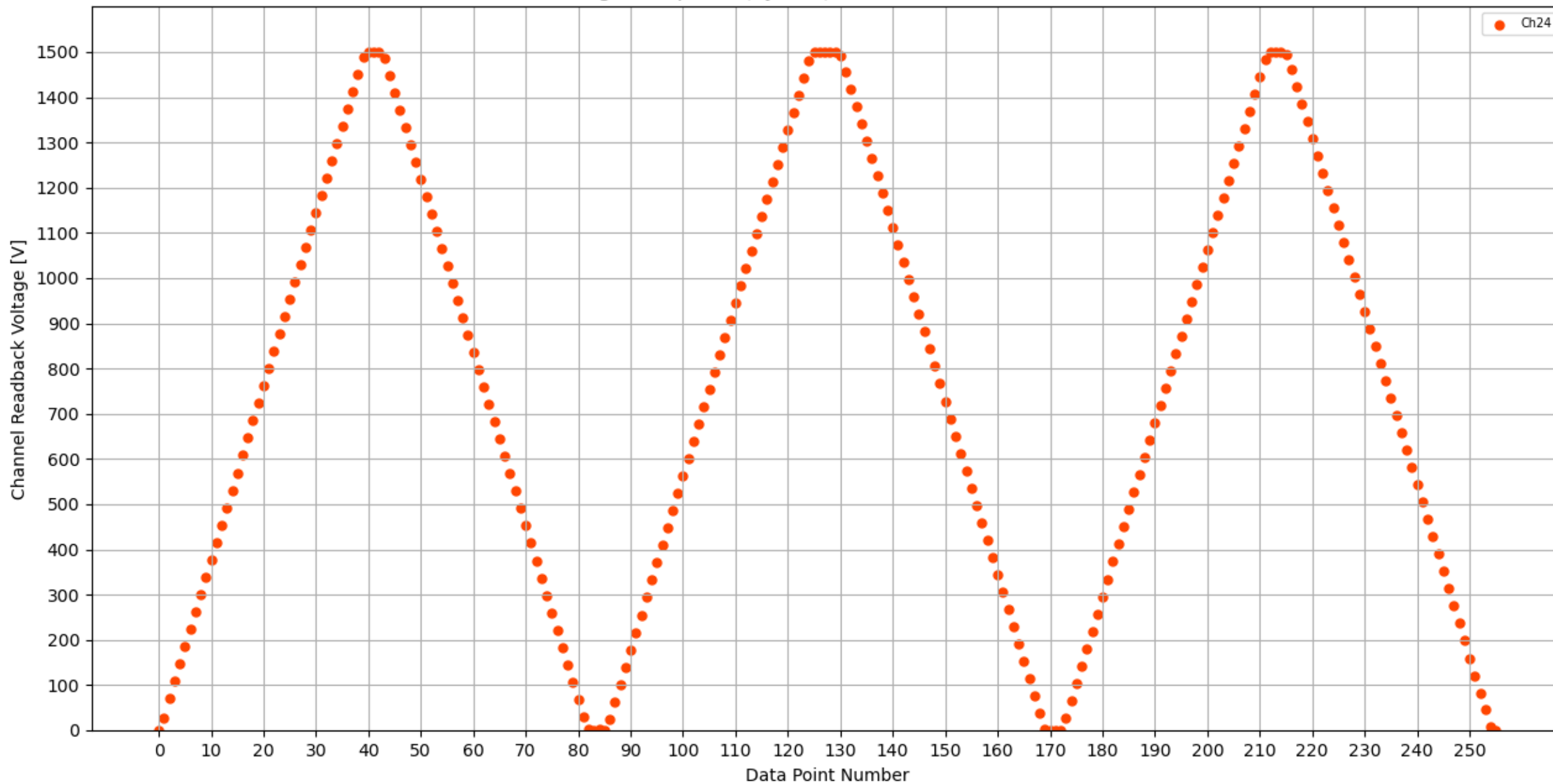
Voltage Ramp Test (Python) Bd #184, Slot #2, Ch #24
