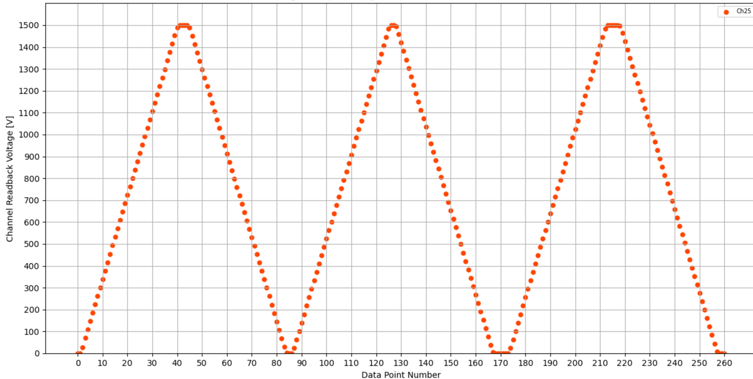
Voltage Ramp Test (Python) Bd #184, Slot #2, Ch #25
