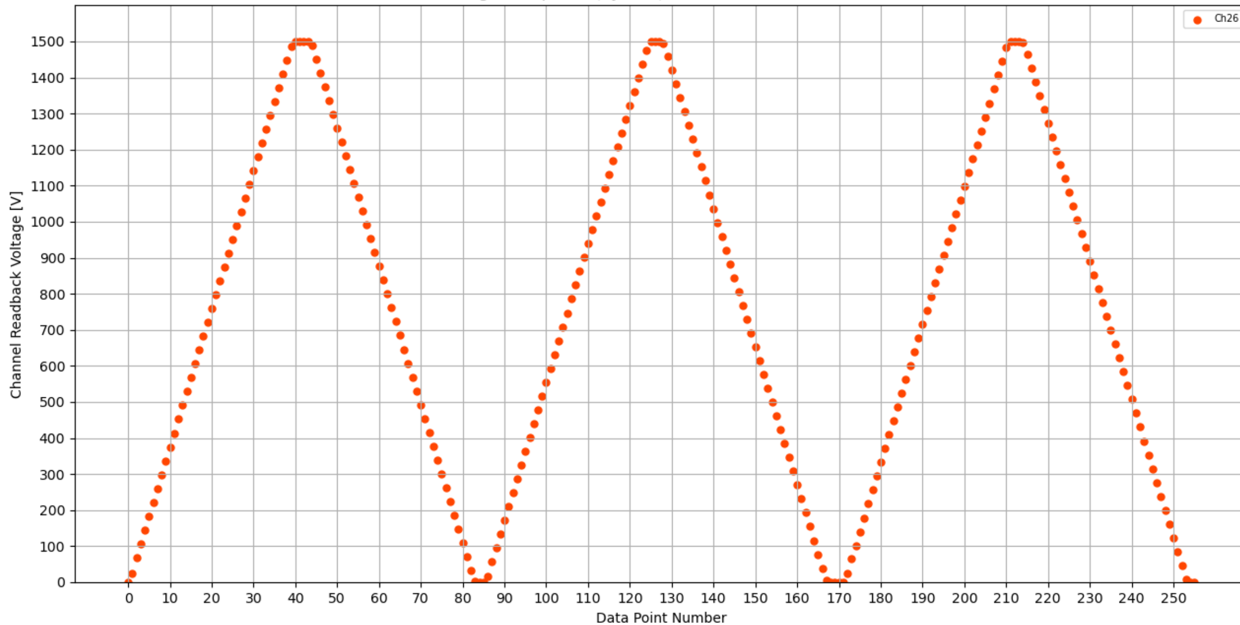
Voltage Ramp Test (Python) Bd #184, Slot #2, Ch #26
