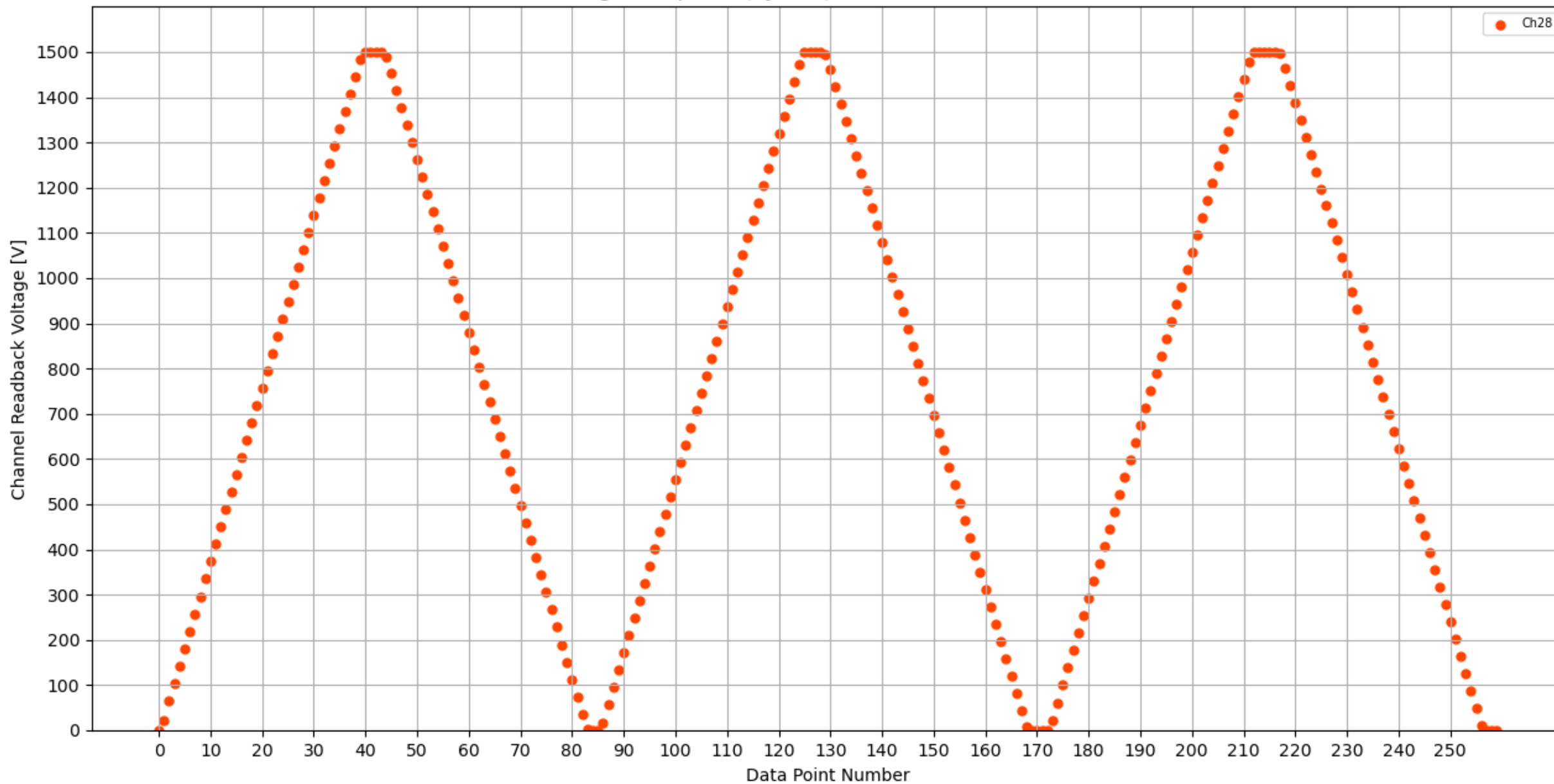
Voltage Ramp Test (Python) Bd #184, Slot #2, Ch #28
