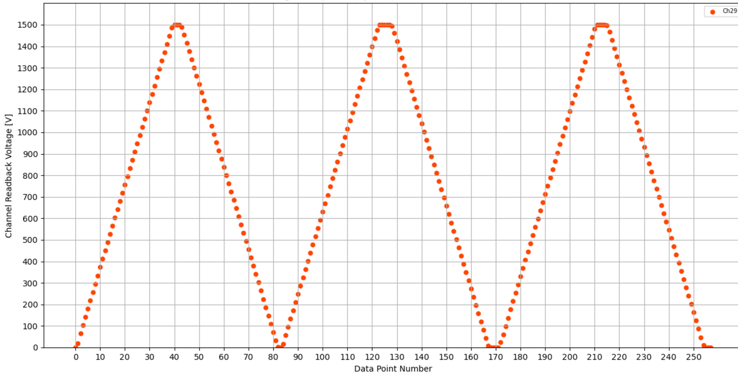
Voltage Ramp Test (Python) Bd #184, Slot #2, Ch #29
