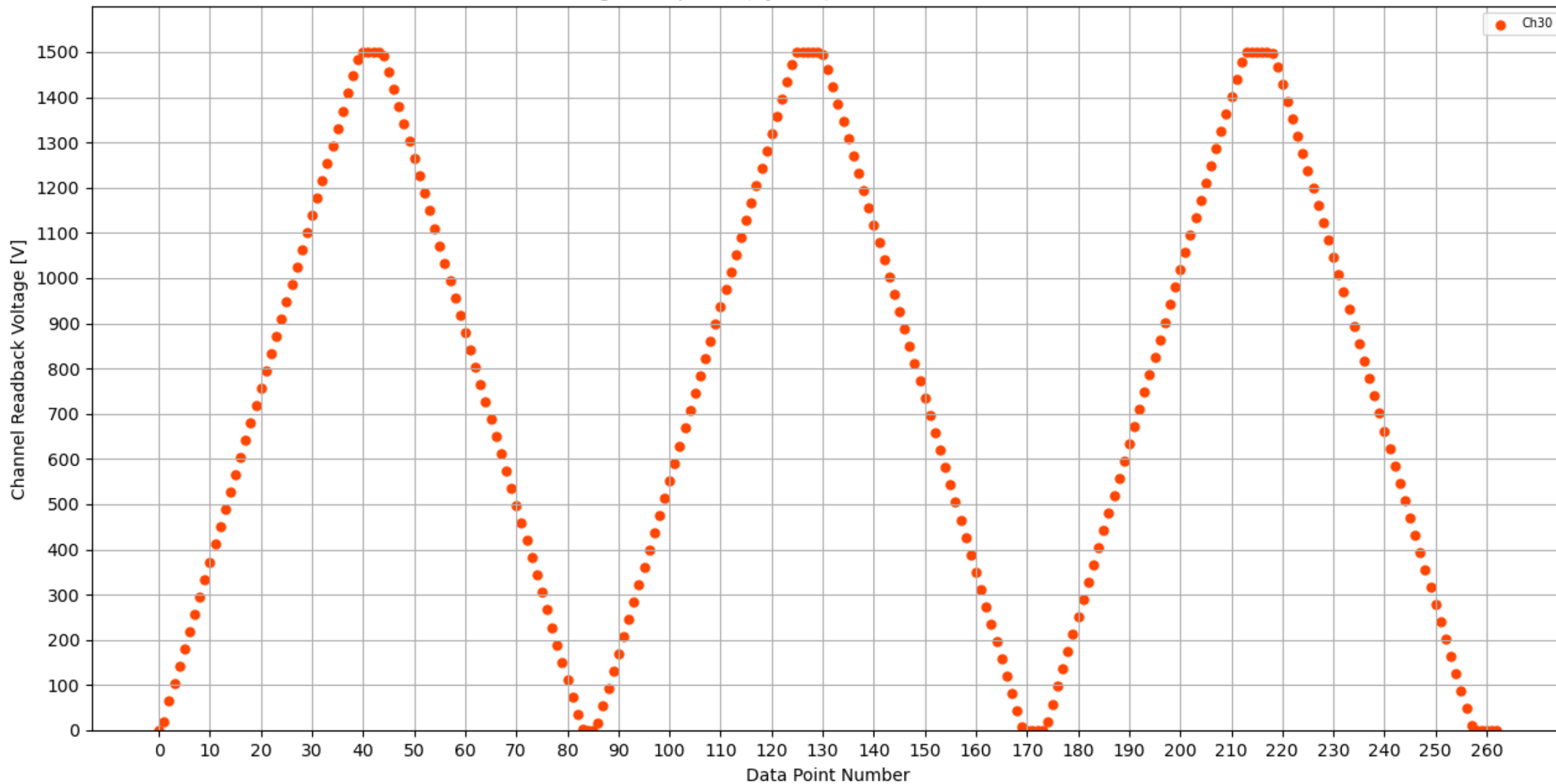
Voltage Ramp Test (Python) Bd #184, Slot #2, Ch #30
