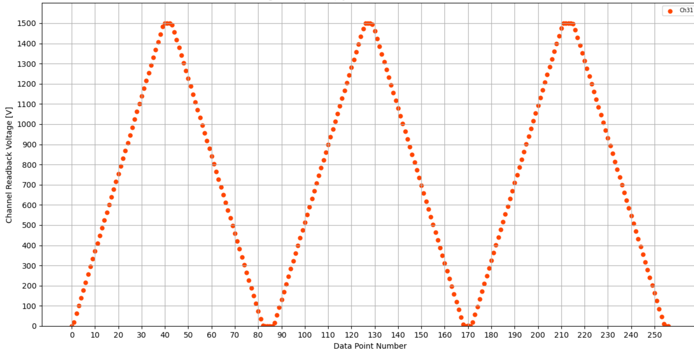
Voltage Ramp Test (Python) Bd #184, Slot #2, Ch #31
