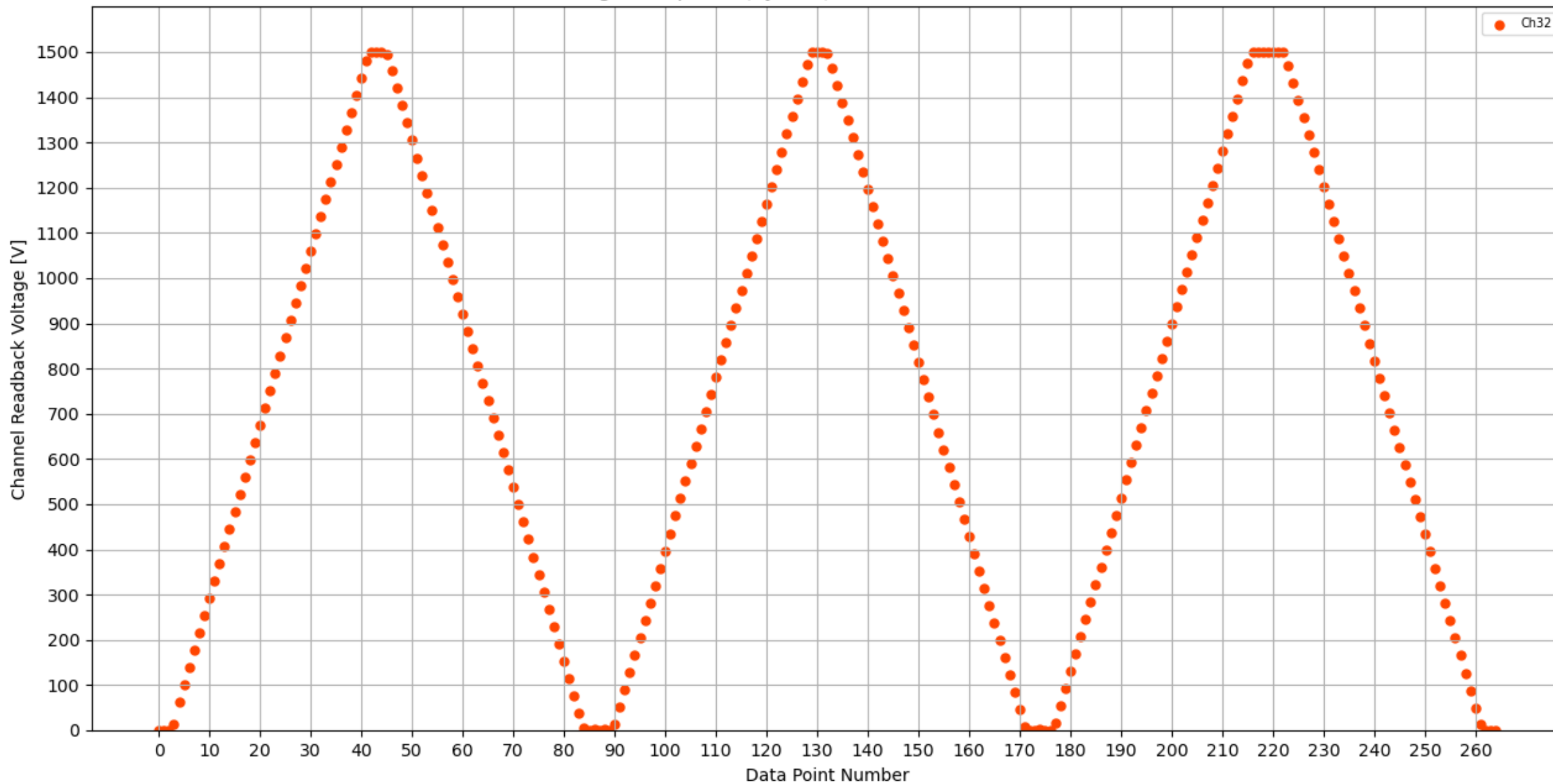
Voltage Ramp Test (Python) Bd #184, Slot #2, Ch #32
