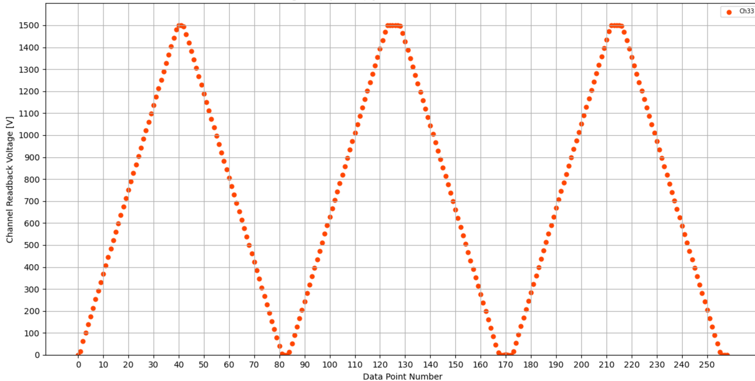
Voltage Ramp Test (Python) Bd #184, Slot #2, Ch #33
