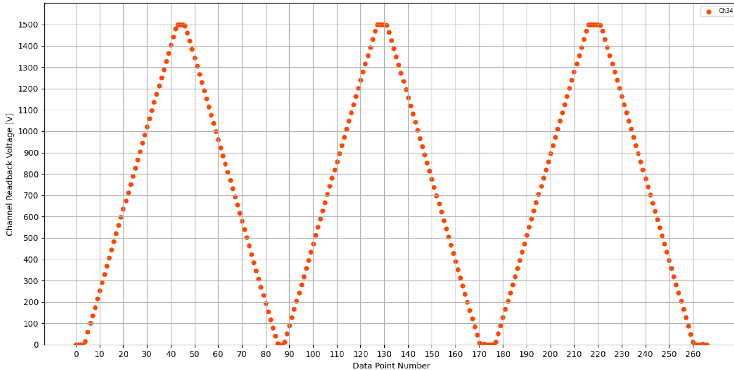
Voltage Ramp Test (Python) Bd #184, Slot #2, Ch #34
