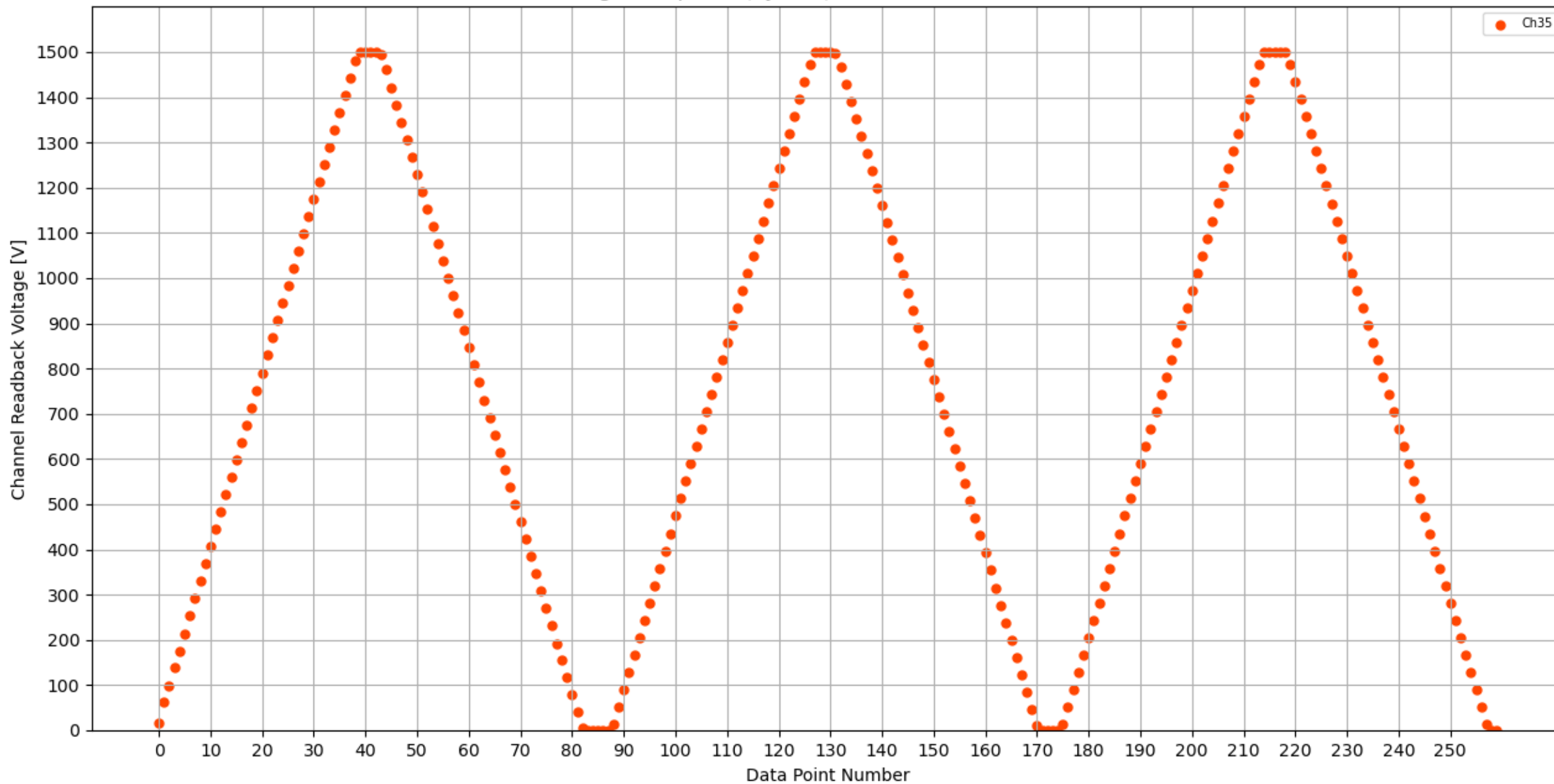
Voltage Ramp Test (Python) Bd #184, Slot #2, Ch #35
