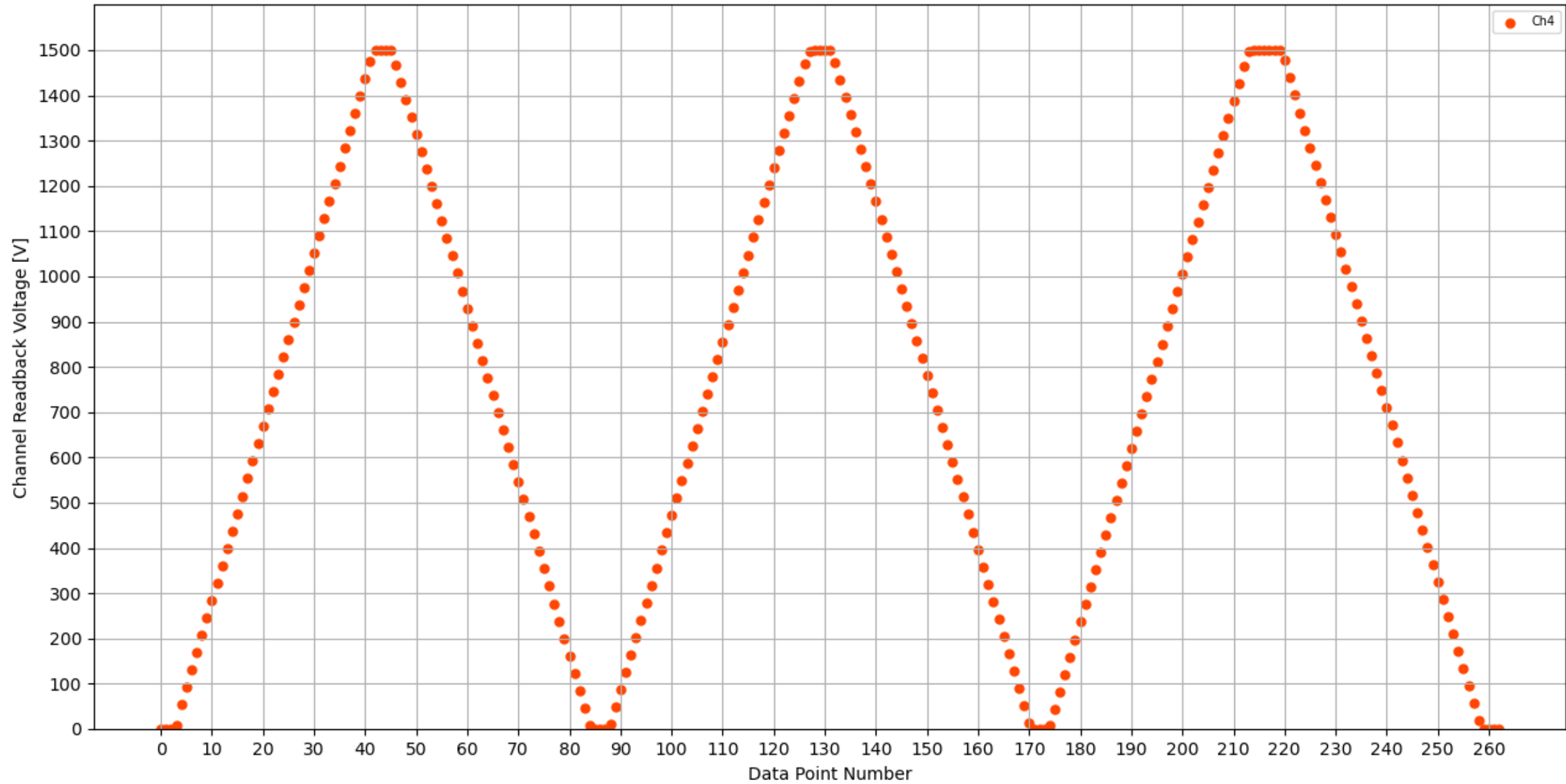
Voltage Ramp Test (Python) Bd #184, Slot #2, Ch #4
