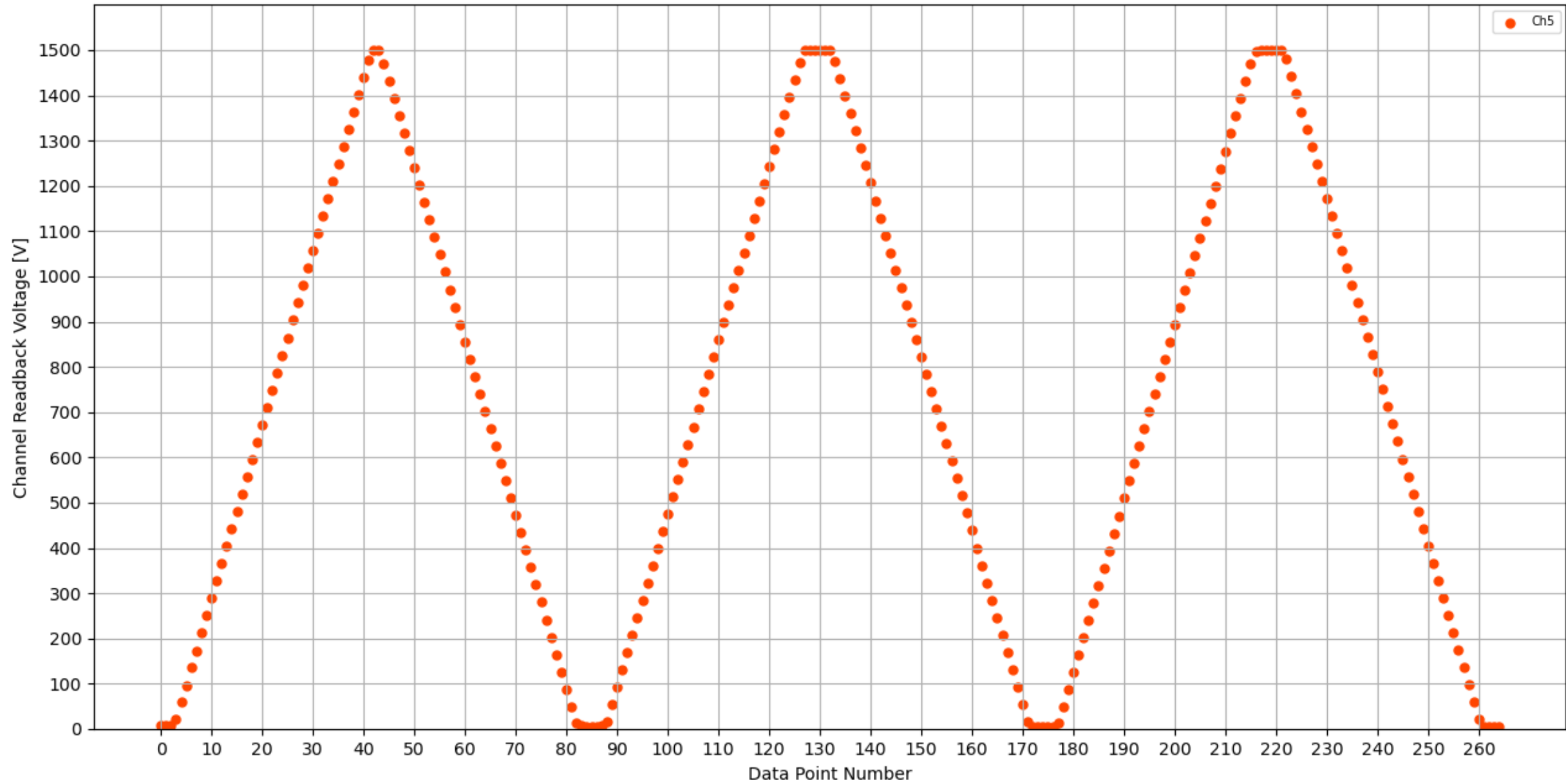
Voltage Ramp Test (Python) Bd #184, Slot #2, Ch #5
