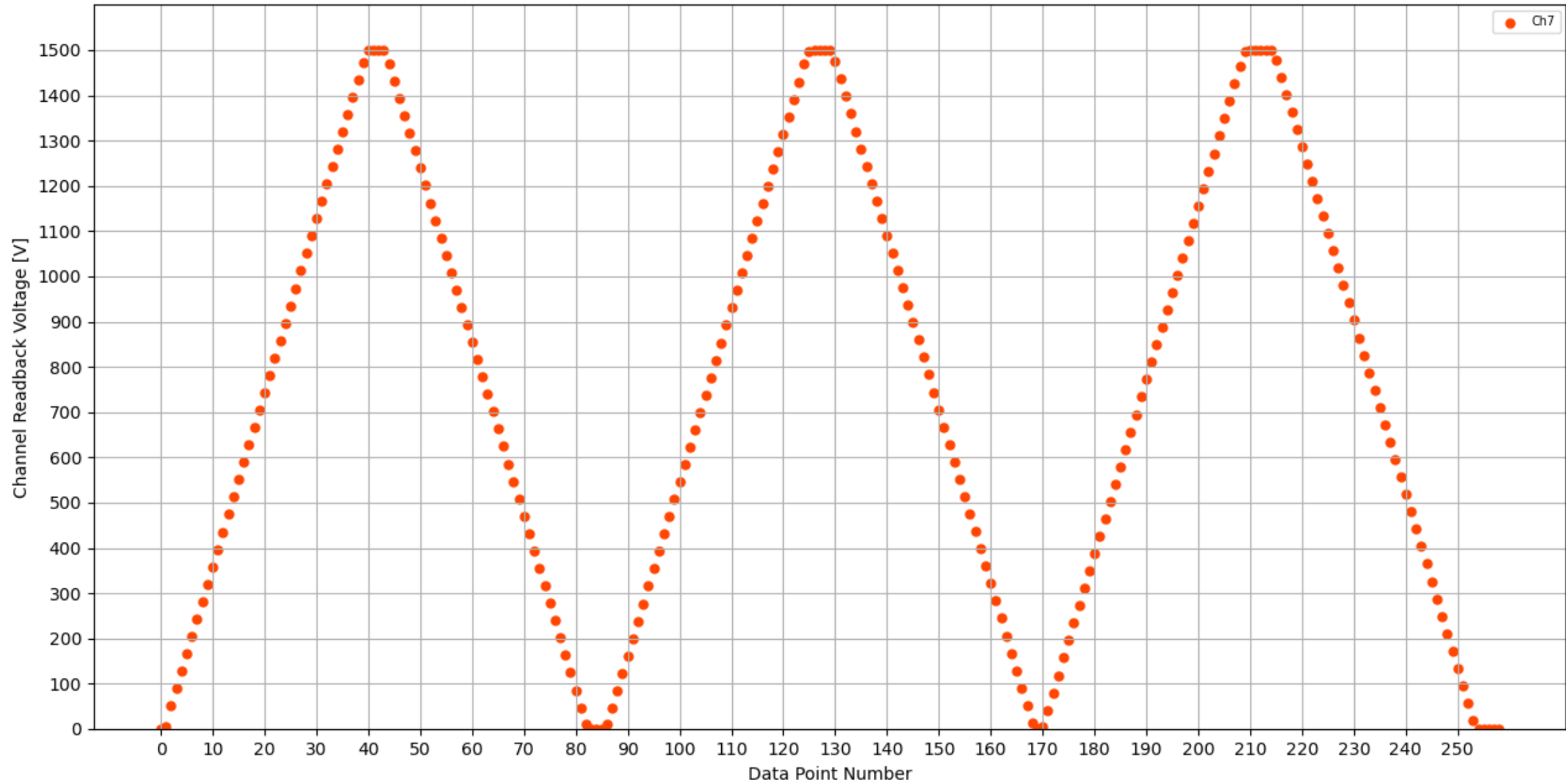
Voltage Ramp Test (Python) Bd #184, Slot #2, Ch #7
