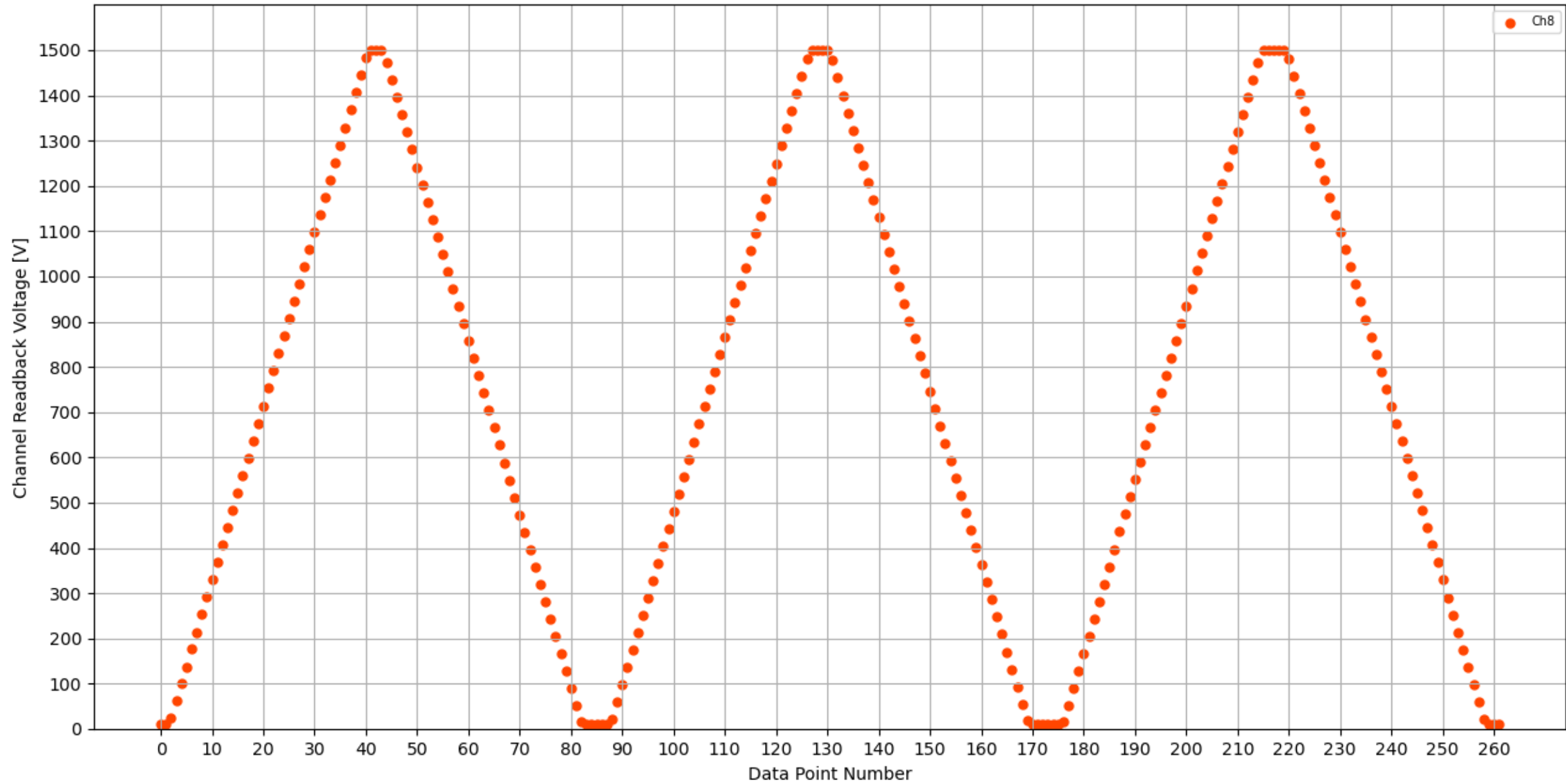
Voltage Ramp Test (Python) Bd #184, Slot #2, Ch #8
