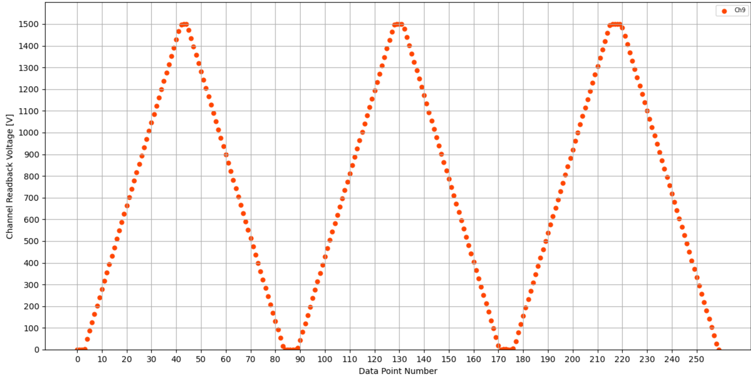
Voltage Ramp Test (Python) Bd #184, Slot #2, Ch #9
