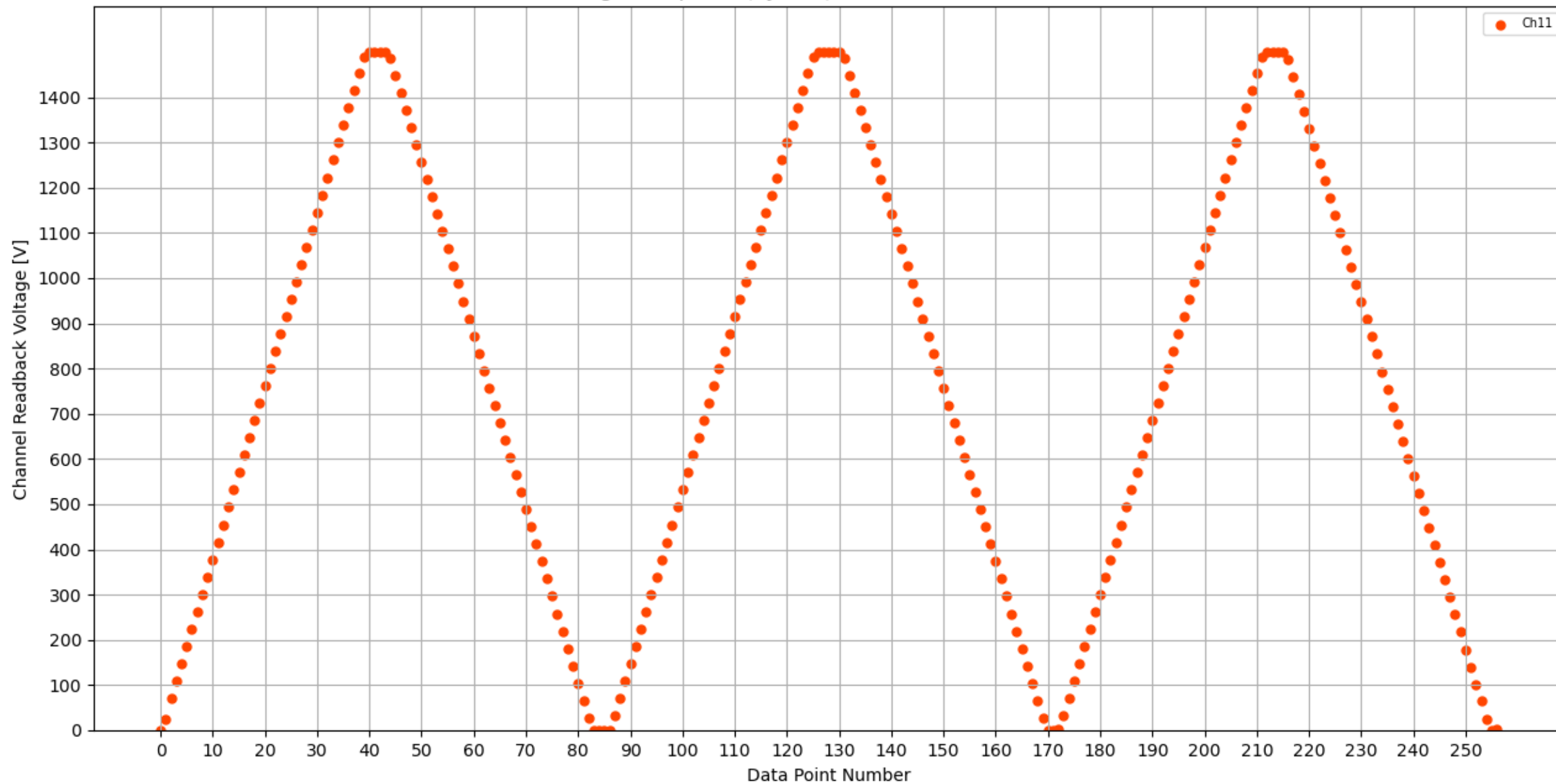
Voltage Ramp Test (Python) Bd #256, Slot #3, Ch #11
