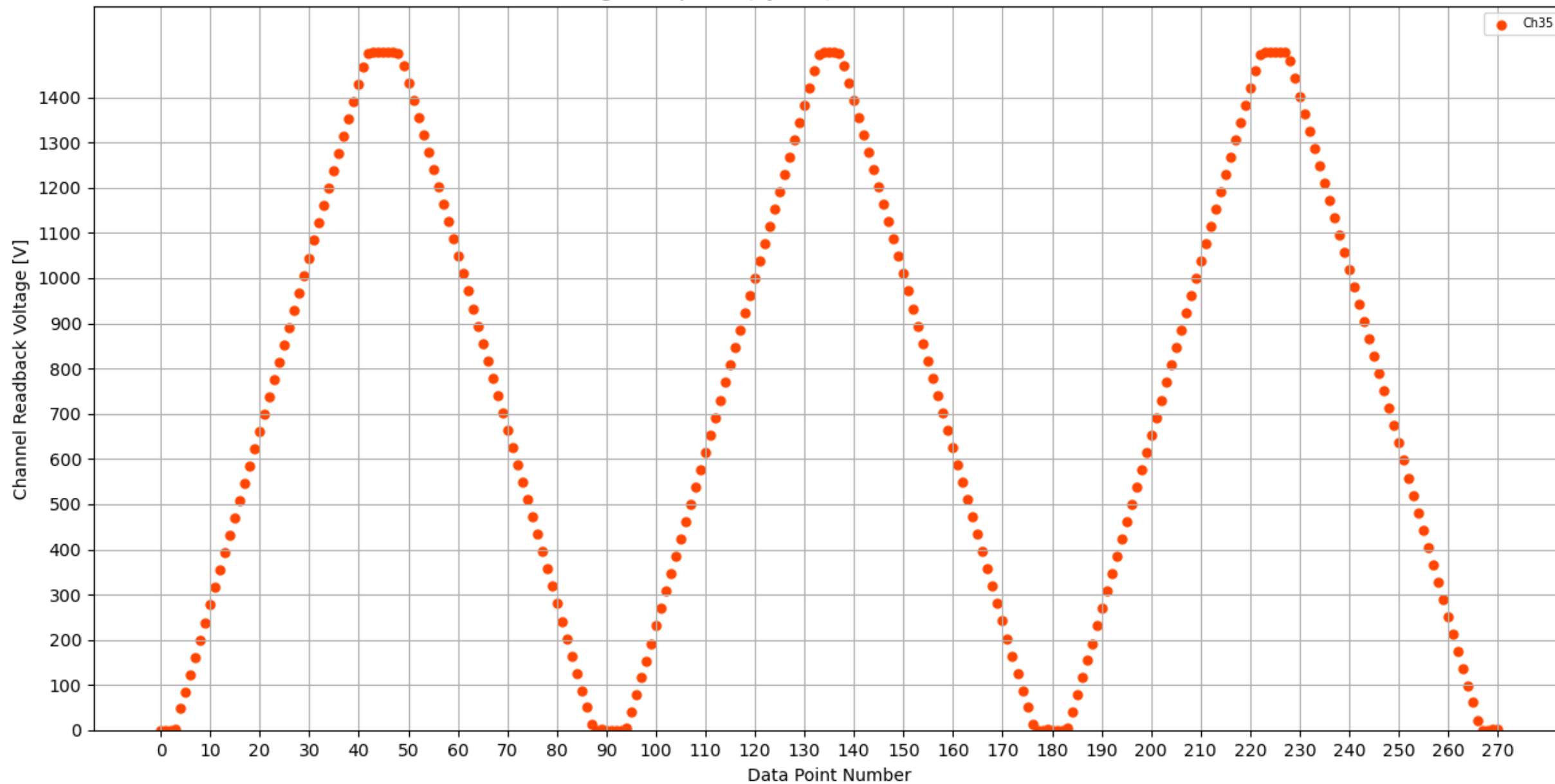
Voltage Ramp Test (Python) Bd #256, Slot #3, Ch #35
