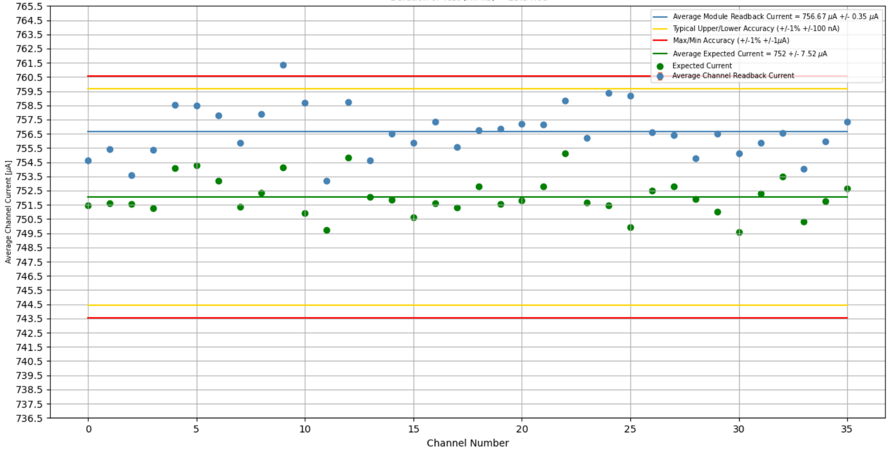
Stability Test 1500 V [With Load]: Trial #1, Crate #2, Slot #8, Board #313 Duration of Test (H:M:S) = 23:54:08
