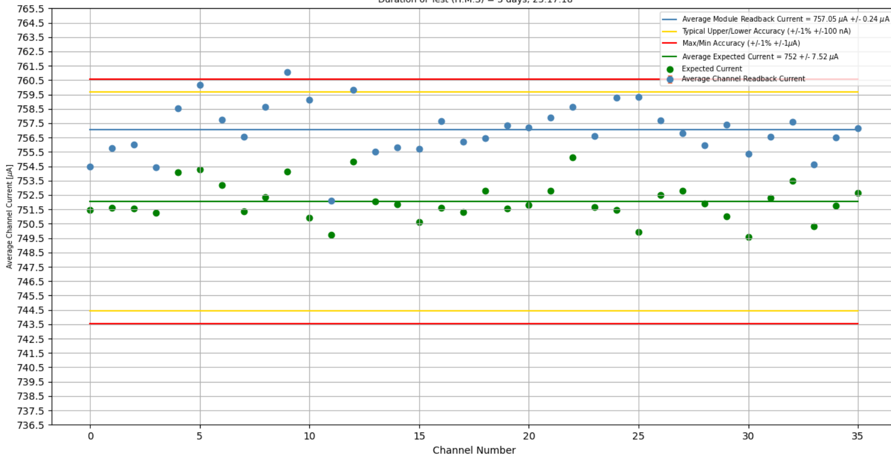
Stability Test 1500 V [With Load]: Trial #1, Crate #2, Slot #13, Board #350 Duration of Test (H:M:S) = 3 days, 23:17:18
