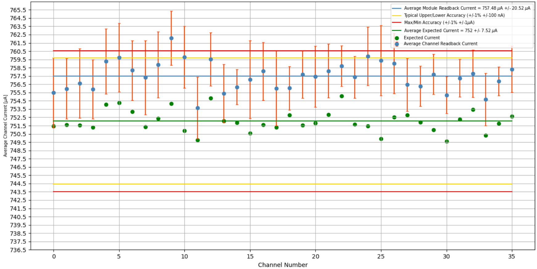
Stability Test 1500 V [With Load]: Trial #1, Crate #2, Slot #5, Board #355 Duration of Test (H:M:S) = 1 day, 0:35:08
