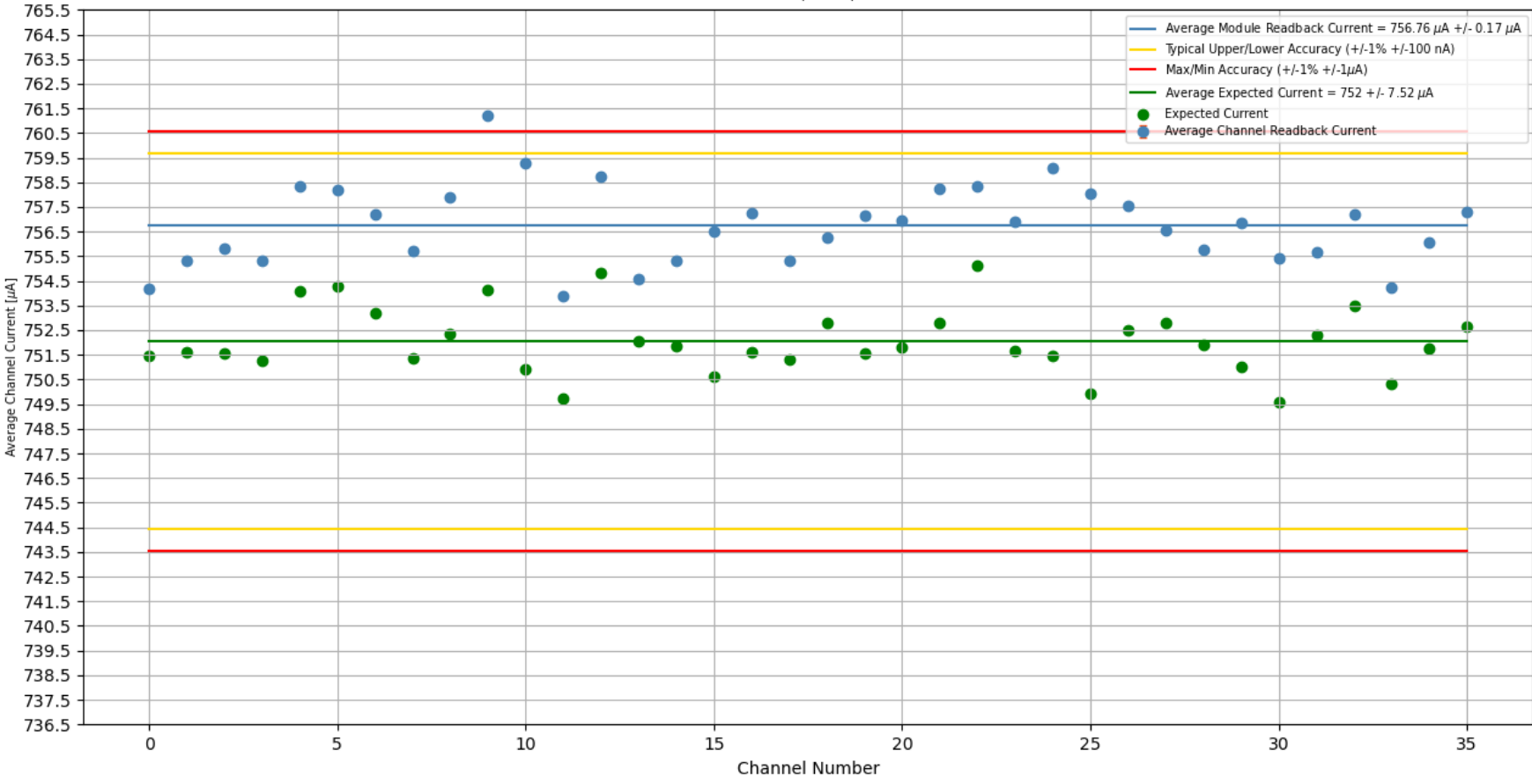
Stability Test 1500 V [With Load]: Trial #1, Crate #2, Slot #10, Board #339 Duration of Test (H:M:S) = 21:56:26
