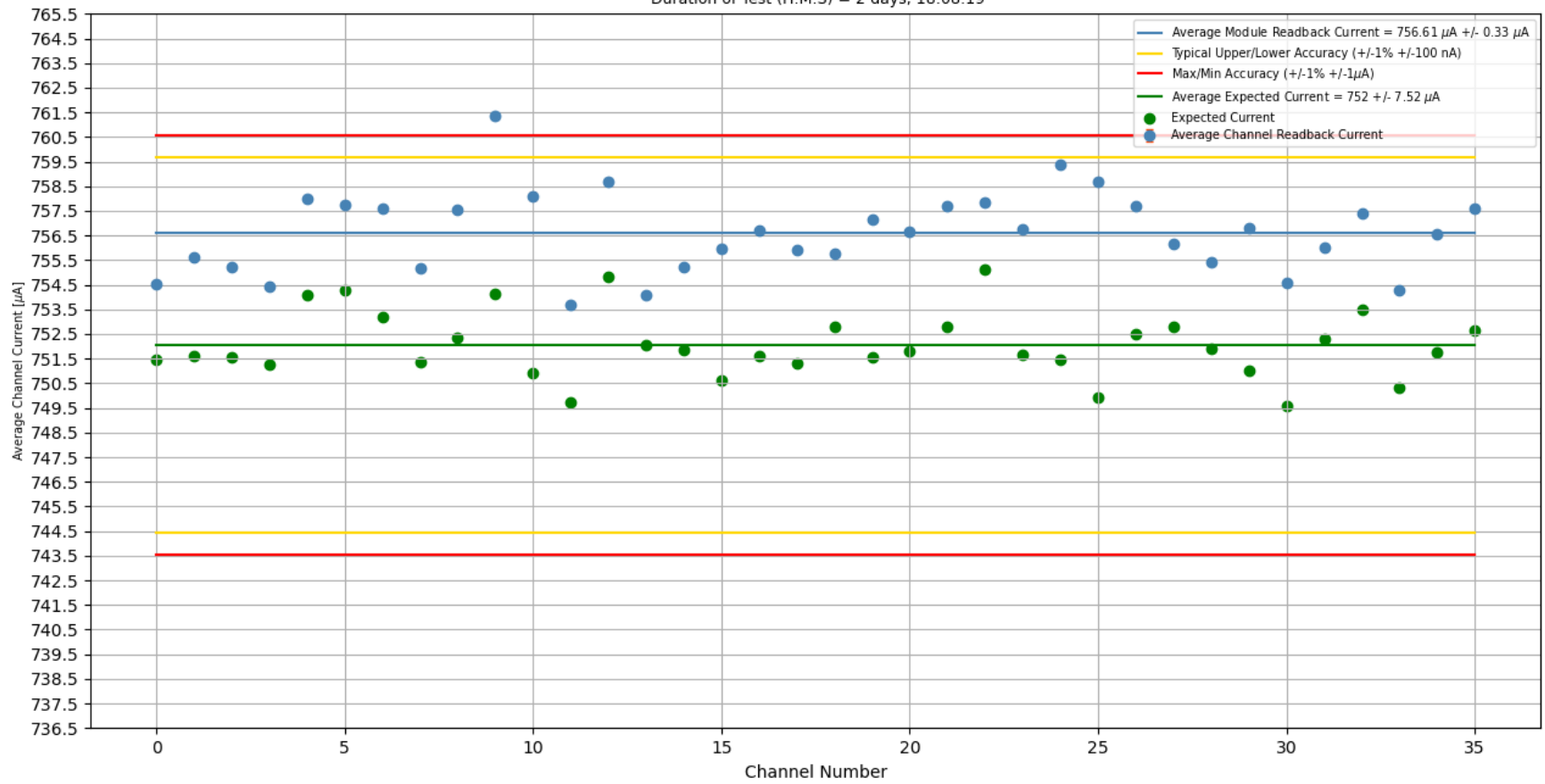
Stability Test 1500 V [With Load]: Trial #1, Crate #3, Slot #9, Board #317 Duration of Test (H:M:S) = 2 days, 18:08:19
