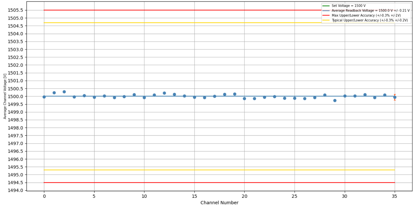
Stability Test 1500 V [With Load]: Trial #1, Crate #3, Slot #12, Board #338 Duration of Test (H:M:S) = 15:27:15
