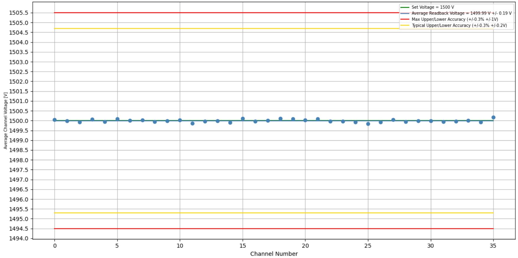
Stability Test 1500 V [With Load]: Trial #1, Crate #3, Slot #6, Board #128 Duration of Test (H:M:S) = 17:50:47
