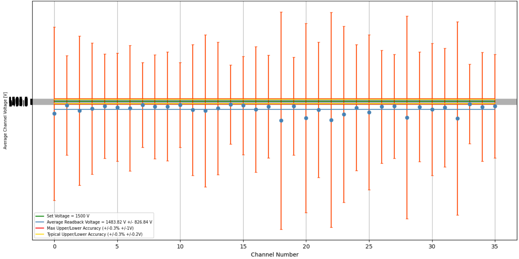
Stability Test 1500 V [With Load]: Trial #1, Crate #2, Slot #0, Board #353 Duration of Test (H:M:S) = 1 day, 0:10:15
