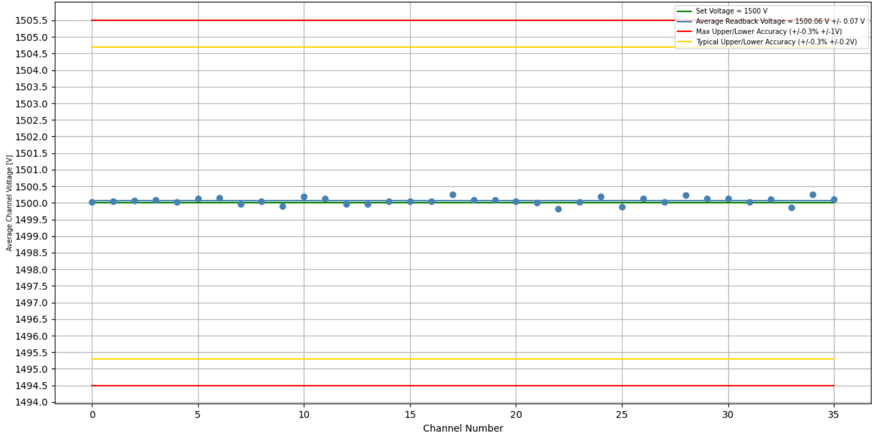
Stability Test 1500 V [With Load]: Trial #1, Crate #2, Slot #3, Board #359 Duration of Test (H:M:S) = 1 day, 0:01:24
