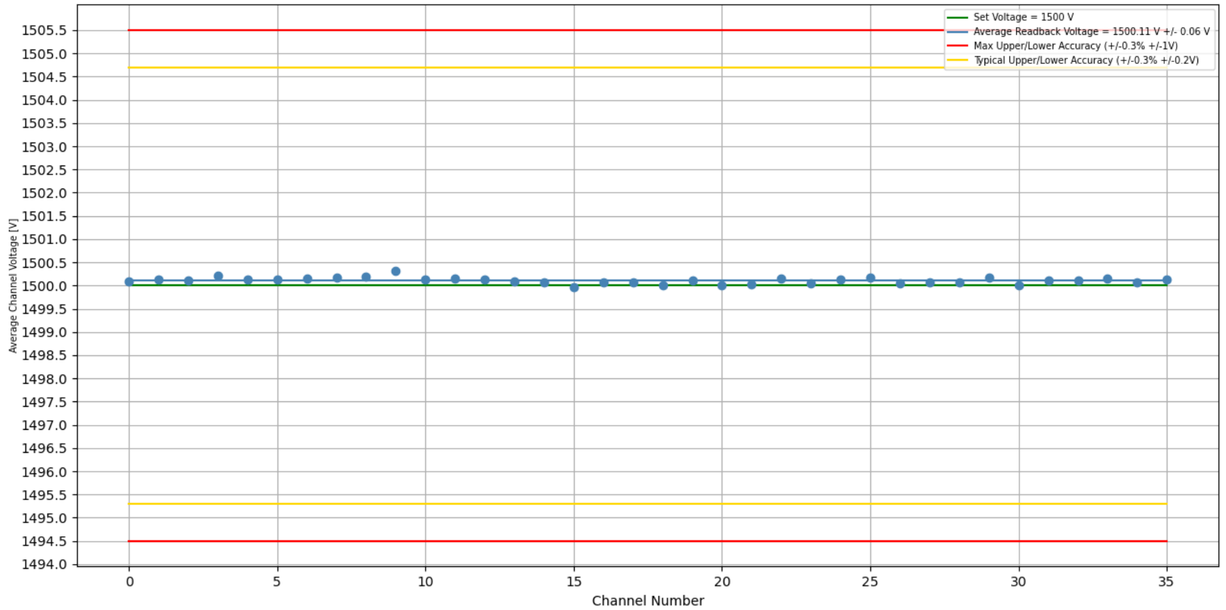
Stability Test 1500 V [With Load]: Trial #1, Crate #2, Slot #12, Board #314 Duration of Test (H:M:S) = 1 day, 0:33:11
