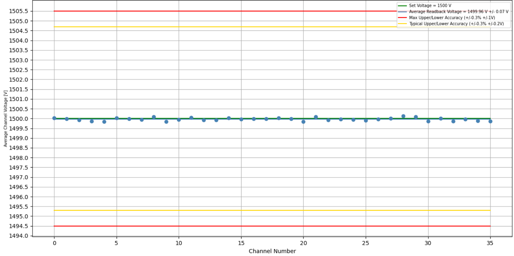
Stability Test 1500 V [With Load]: Trial #1, Crate #3, Slot #10, Board #324 Duration of Test (H:M:S) = 21:07:10
