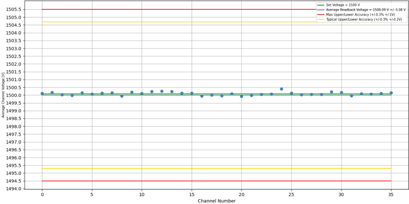
Stability Test 1500 V [With Load]: Trial #1, Crate #2, Slot #6, Board #358 Duration of Test (H:M:S) = 1 day, 0:09:35
