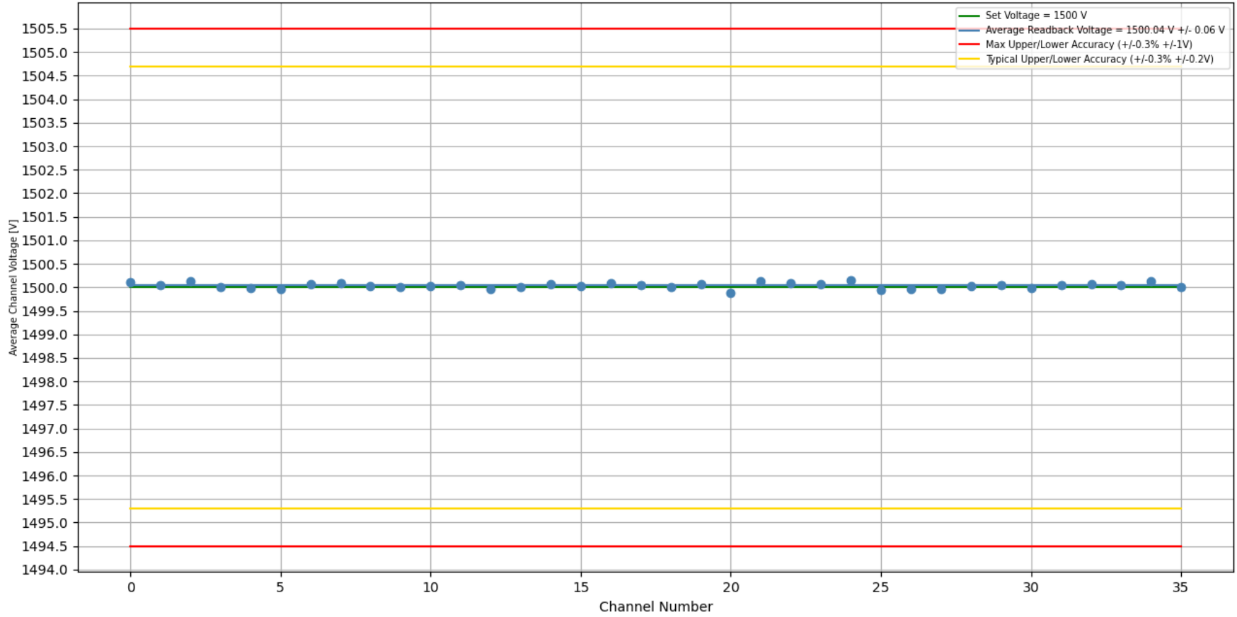
Stability Test 1500 V [With Load]: Trial #1, Crate #3, Slot #5, Board #262 Duration of Test (H:M:S) = 19:37:37
