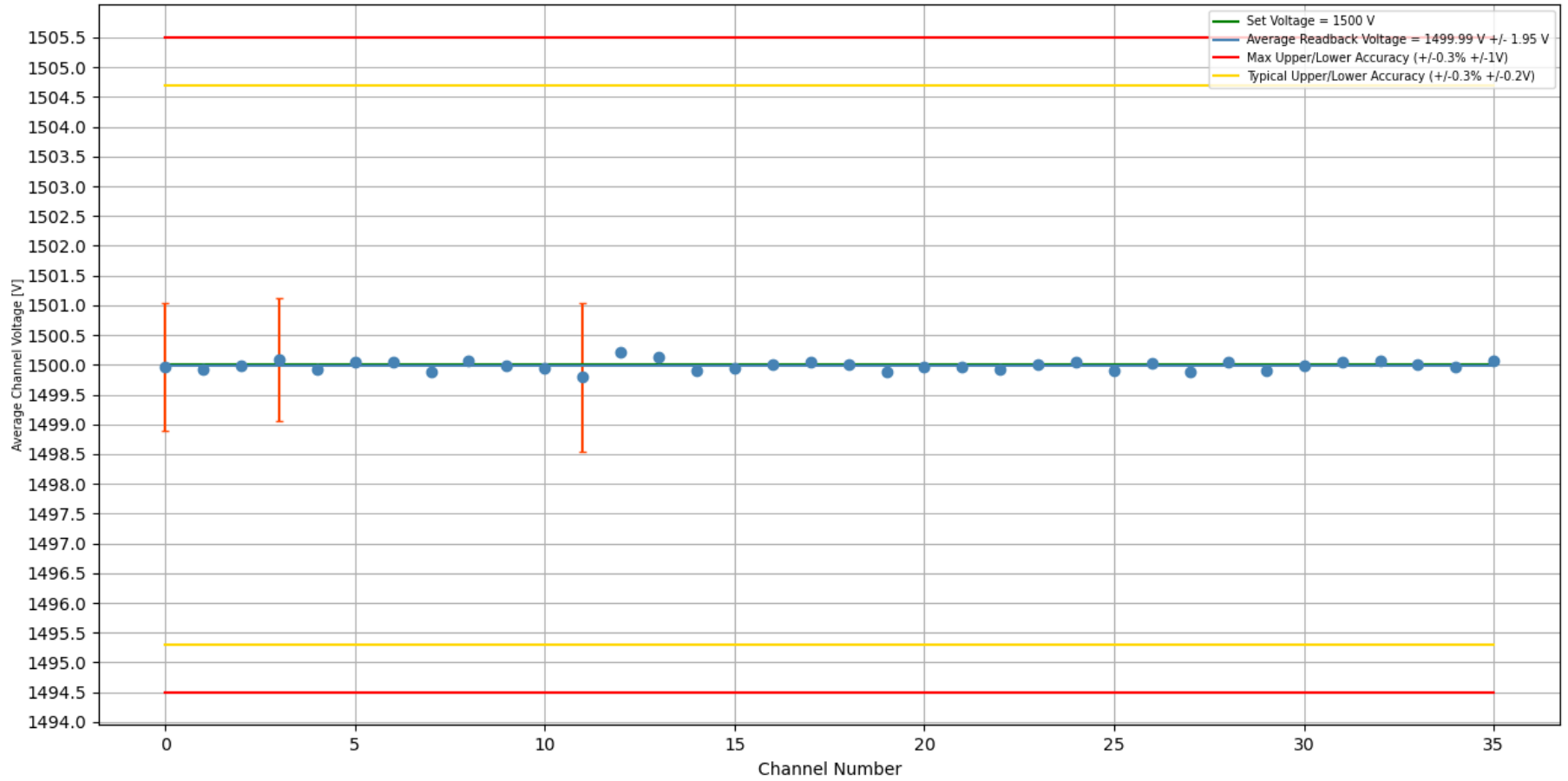
Stability Test 1500 V [With Load]: Trial #1, Crate #2, Slot #4, Board #327 Duration of Test (H:M:S) = 2 days, 22:51:20
