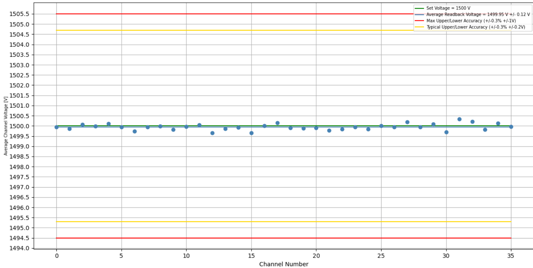
Stability Test 1500 V [With Load]: Trial #1, Crate #3, Slot #13, Board #302 Duration of Test (H:M:S) = 22:20:14
