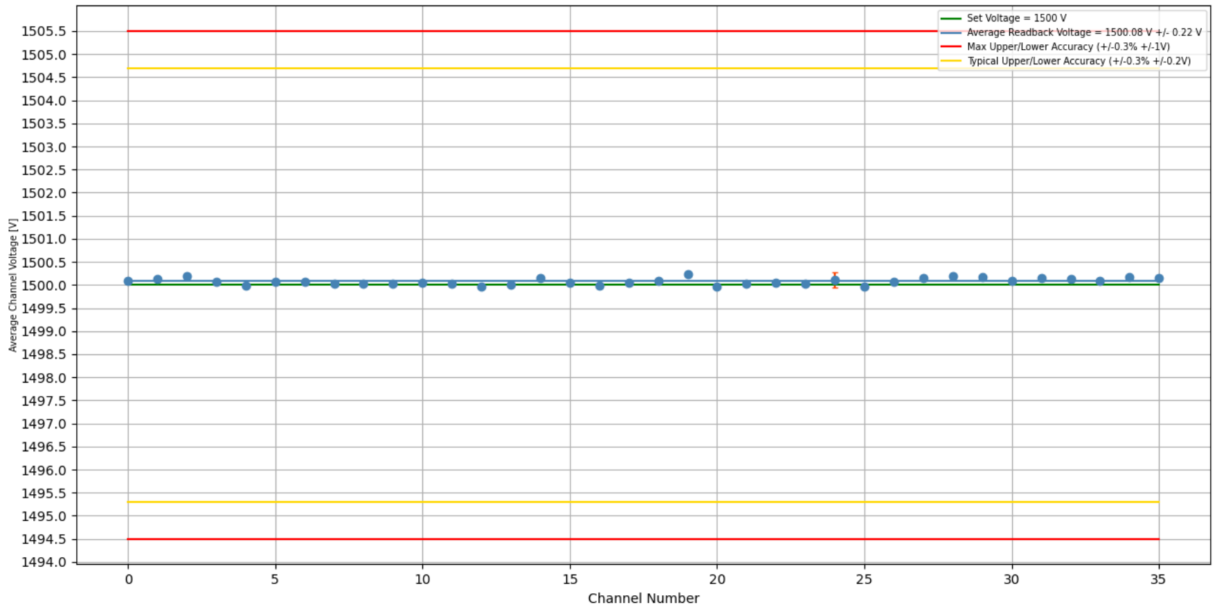
Stability Test 1500 V [With Load]: Trial #1, Crate #3, Slot #15, Board #184 Duration of Test (H:M:S) = 18:09:31
