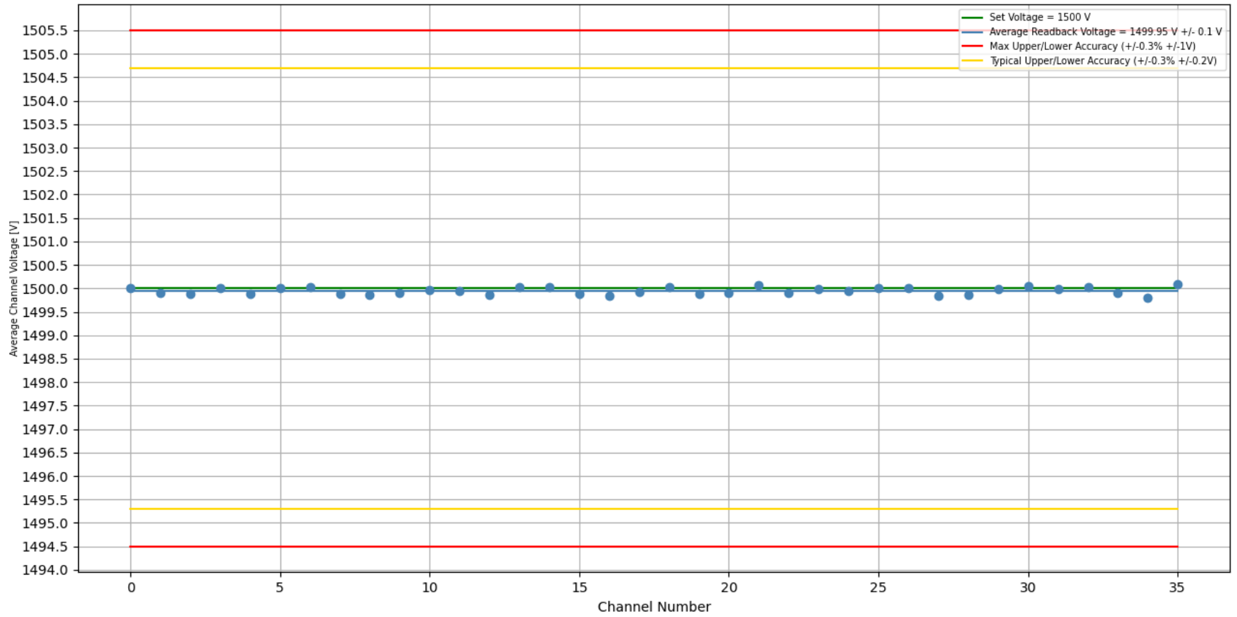
Stability Test 1500 V [With Load]: Trial #1, Crate #2, Slot #1, Board #356 Duration of Test (H:M:S) = 22:05:36
