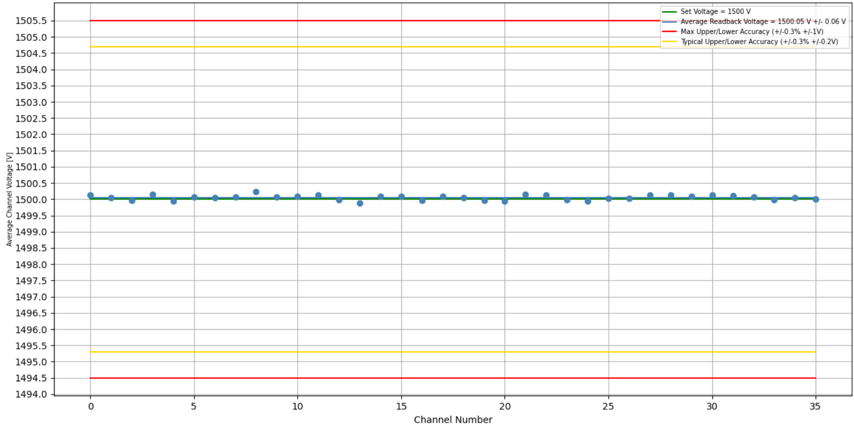
Stability Test 1500 V [With Load]: Trial #1, Crate #2, Slot #2, Board #352 Duration of Test (H:M:S) = 1 day, 0:24:36
