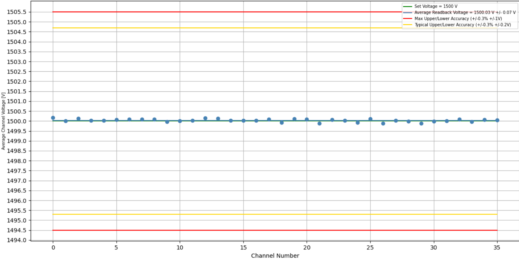
Stability Test 1500 V [With Load]: Trial #1, Crate #3, Slot #14, Board #256 Duration of Test (H:M:S) = 2 days, 17:17:58
