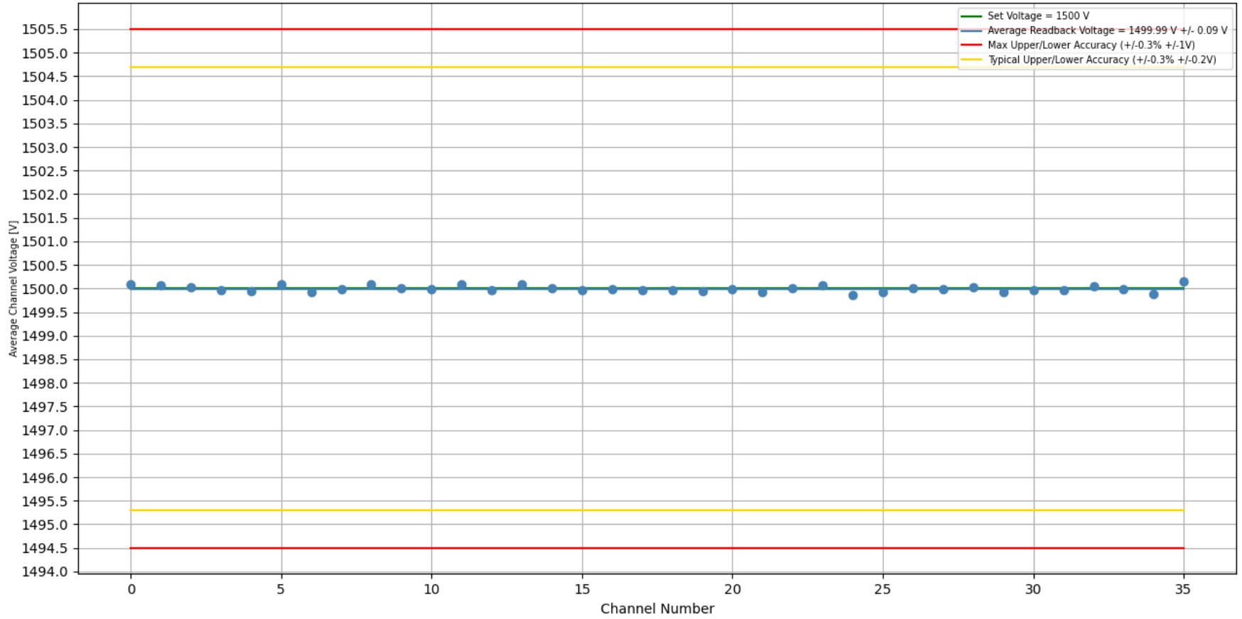
Stability Test 1500 V [With Load]: Trial #1, Crate #3, Slot #1, Board #325 Duration of Test (H:M:S) = 2 days, 23:03:57
