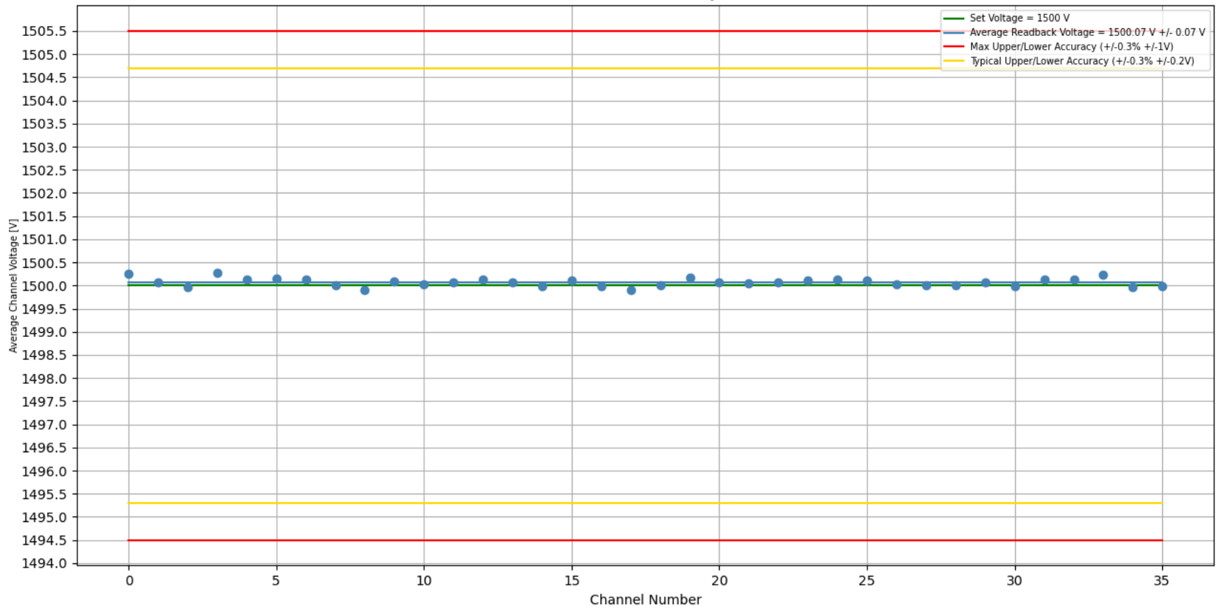
Stability Test 1500 V [With Load]: Trial #1, Crate #2, Slot #15, Board #336 Duration of Test (H:M:S) = 1 day, 0:17:26
