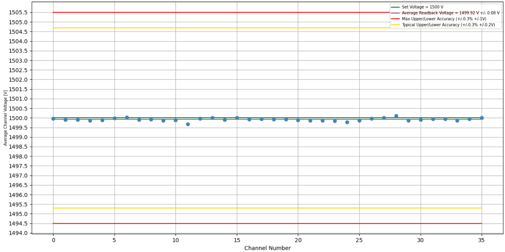
Stability Test 1500 V [With Load]: Trial #1, Crate #3, Slot #0, Board #304 Duration of Test (H:M:S) = 1 day, 0:13:07
