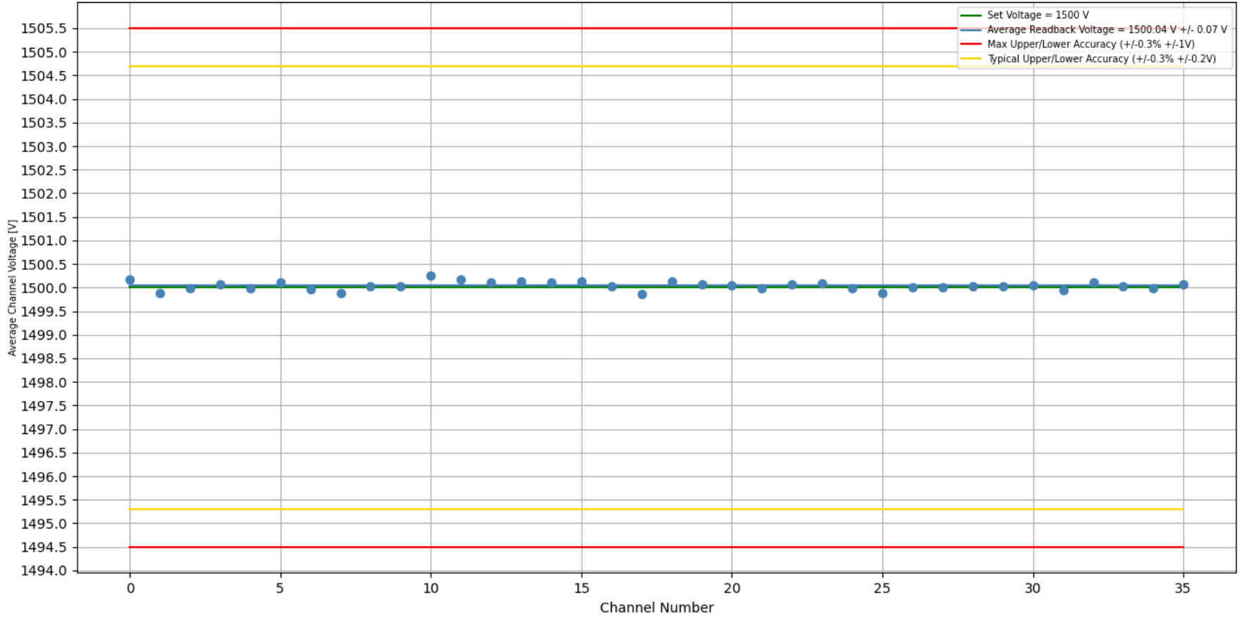
Stability Test 1500 V [With Load]: Trial #1, Crate #2, Slot #10, Board #339 Duration of Test (H:M:S) = 21:56:26
