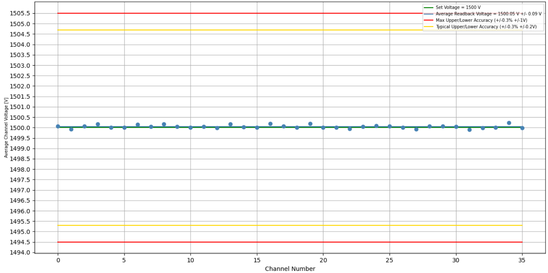
Stability Test 1500 V [With Load]: Trial #1, Crate #2, Slot #9, Board #309 Duration of Test (H:M:S) = 2 days, 23:15:36
