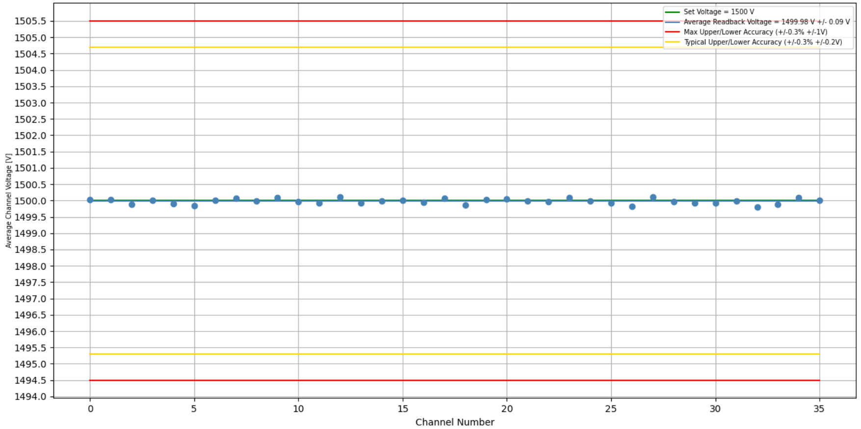
Stability Test 1500 V [With Load]: Trial #1, Crate #3, Slot #9, Board #317 Duration of Test (H:M:S) = 1 day, 0:05:07
