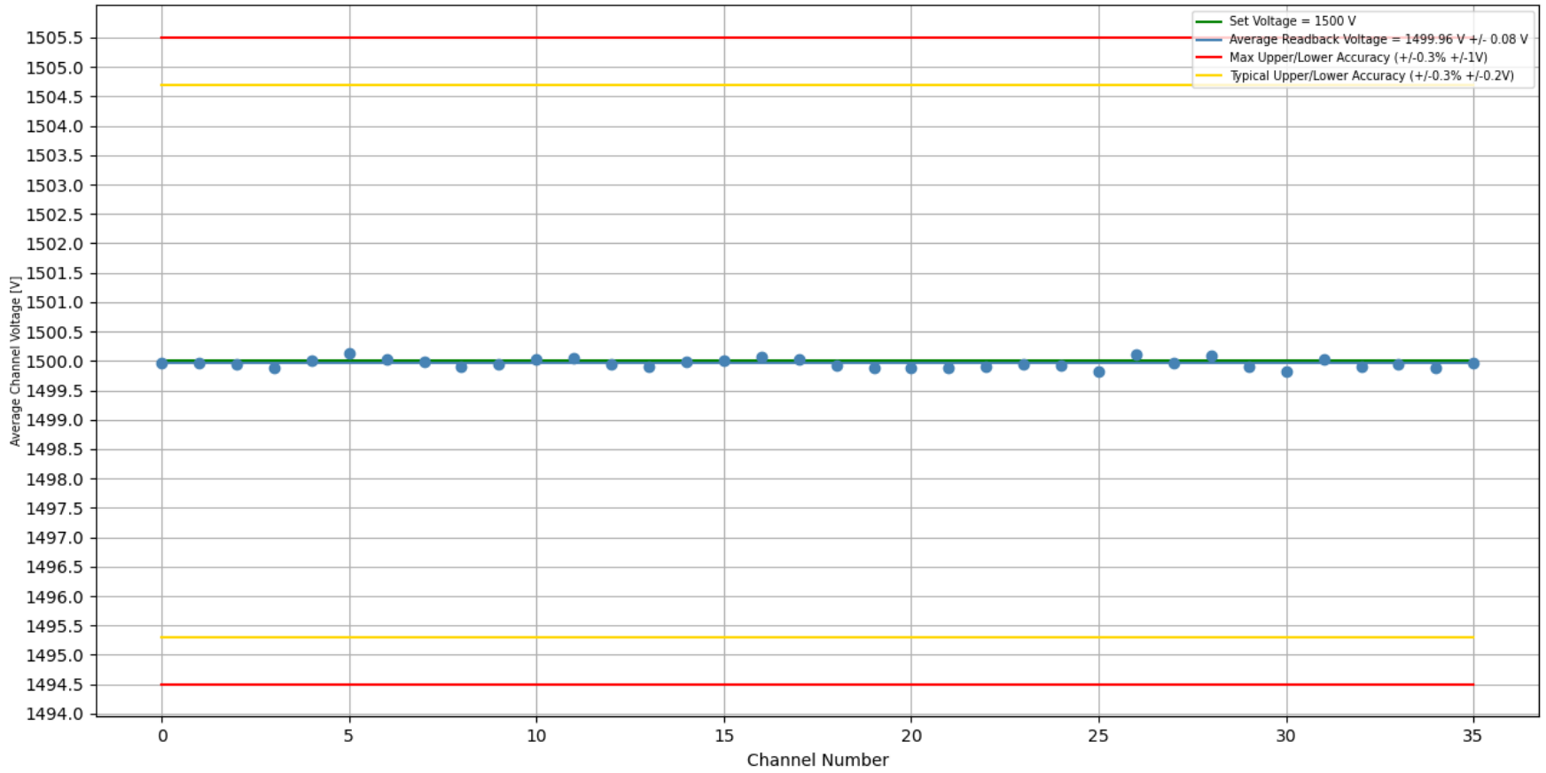
Stability Test 1500 V [With Load]: Trial #1, Crate #3, Slot #4, Board #337 Duration of Test (H:M:S) = 3 days, 0:47:20
