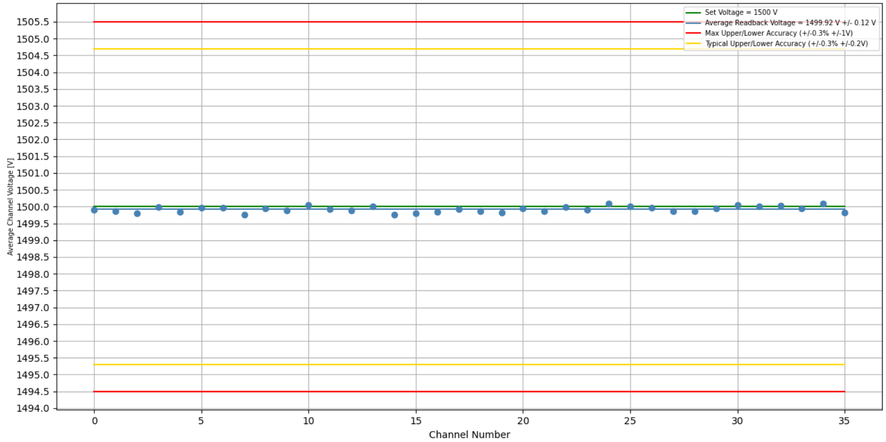
Stability Test 1500 V [With Load]: Trial #1, Crate #3, Slot #8, Board #173 Duration of Test (H:M:S) = 1 day, 0:05:07
