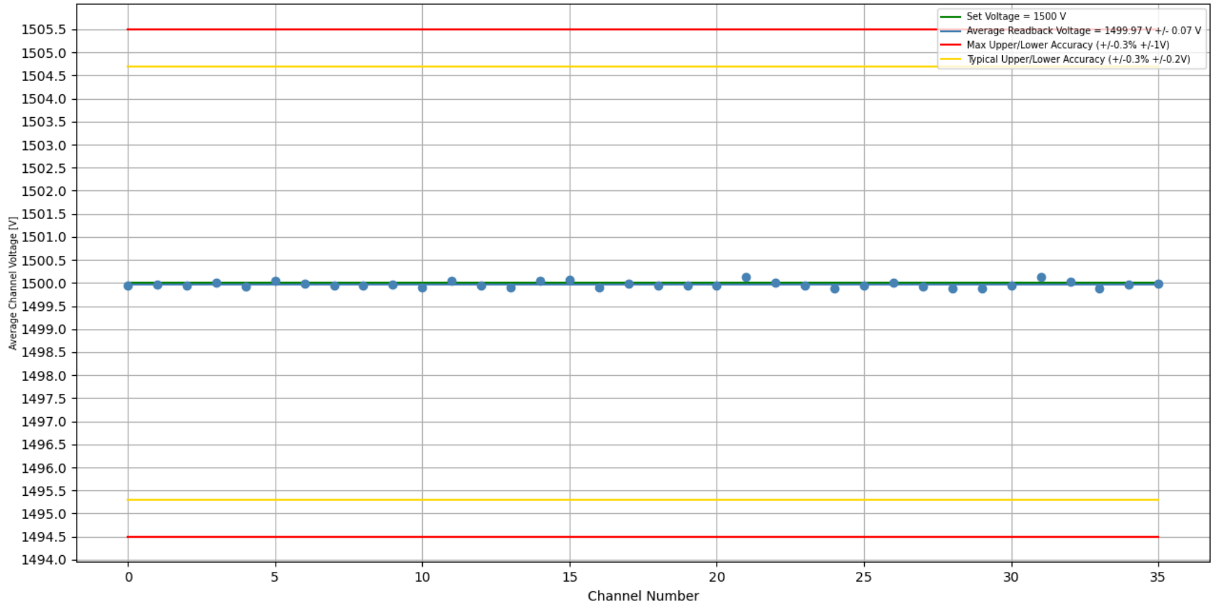
Stability Test 1500 V [With Load]: Trial #1, Crate #3, Slot #3, Board #347 Duration of Test (H:M:S) = 1 day, 0:04:19
