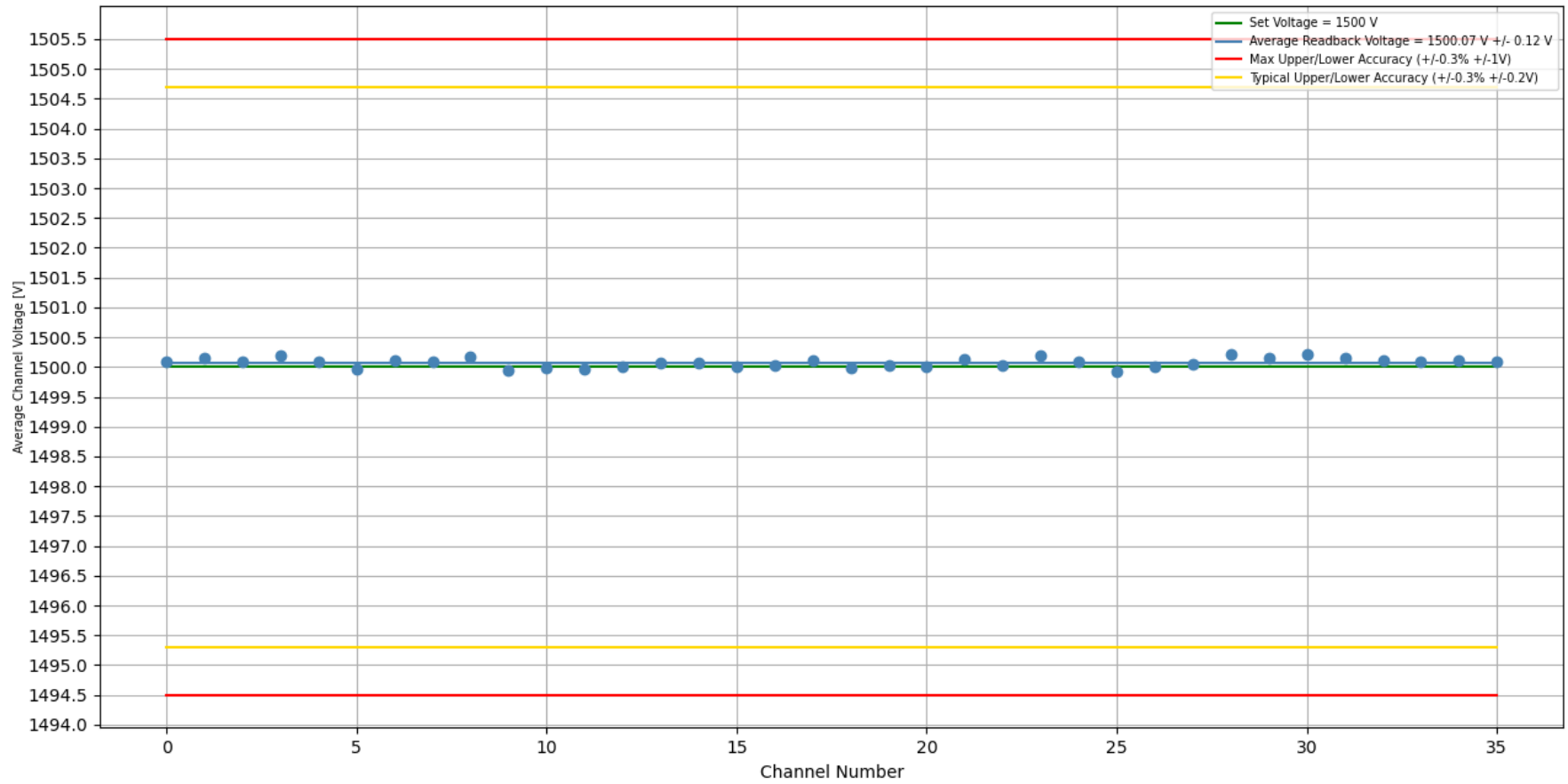
Stability Test 1500 V [With Load]: Trial #1, Crate #2, Slot #14, Board #354 Duration of Test (H:M:S) = 1 day, 0:14:24
