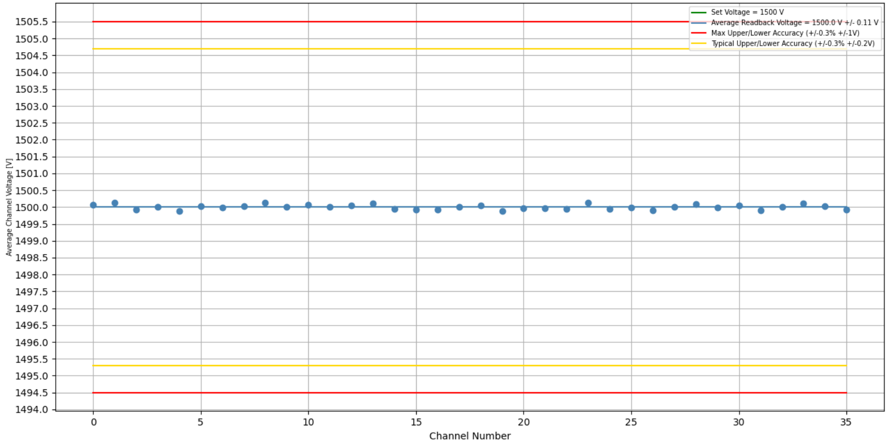
Stability Test 1500 V [With Load]: Trial #1, Crate #3, Slot #2, Board #301 Duration of Test (H:M:S) = 22:01:55
