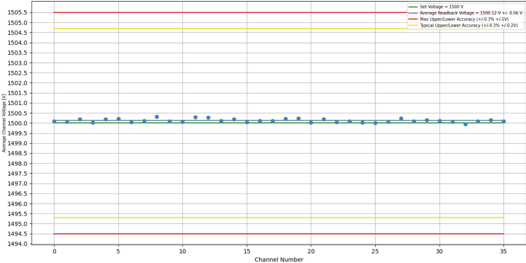
Stability Test 1500 V [With Load]: Trial #1, Crate #2, Slot #11, Board #316 Duration of Test (H:M:S) = 1 day, 1:47:44
