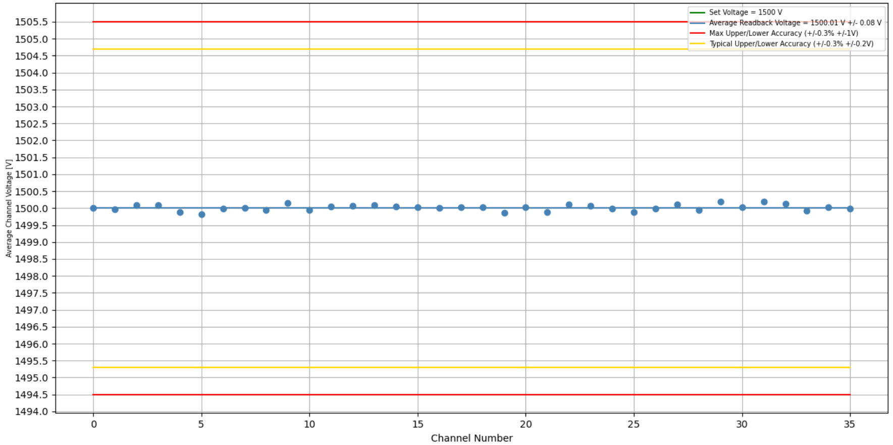
Stability Test 1500 V [With Load]: Trial #1, Crate #3, Slot #11, Board #326 Duration of Test (H:M:S) = 2 days, 18:11:21
