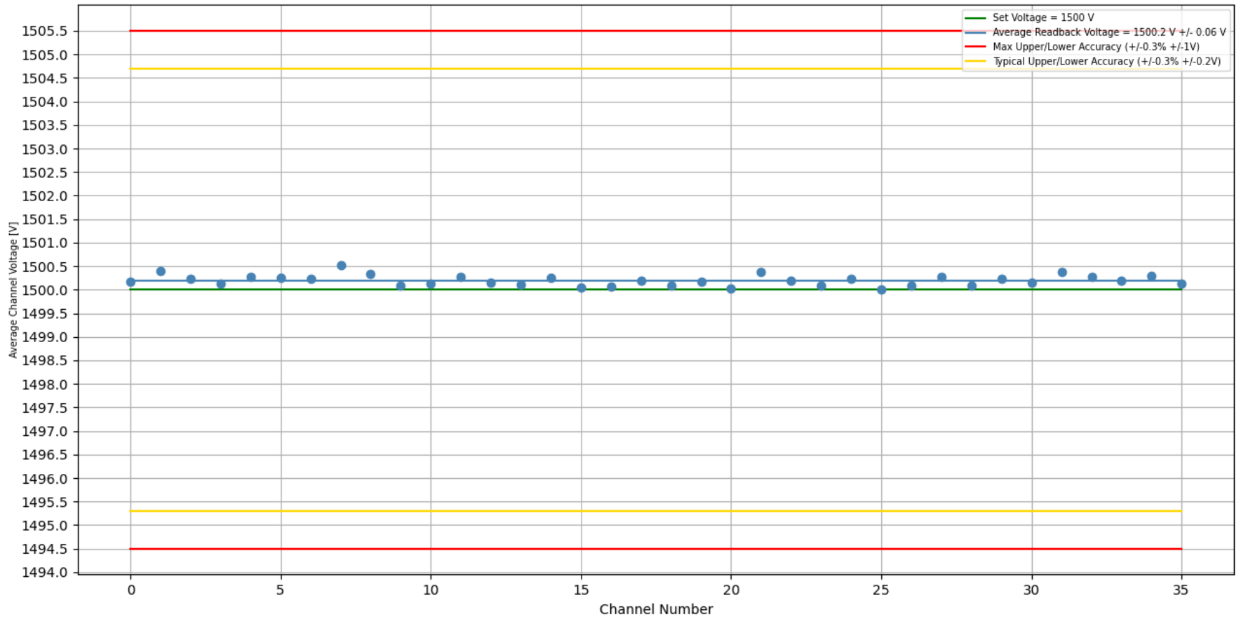
Stability Test 1500 V [With Load]: Trial #1, Crate #2, Slot #13, Board #350 Duration of Test (H:M:S) = 3 days, 23:17:18
