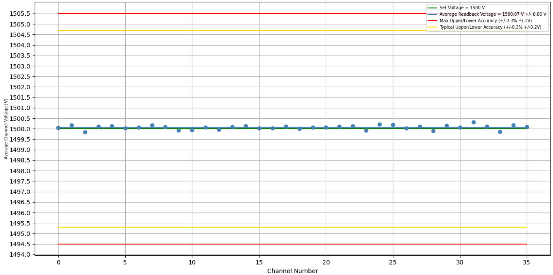
Stability Test 1500 V [With Load]: Trial #1, Crate #2, Slot #7, Board #351 Duration of Test (H:M:S) = 1 day, 0:35:03
