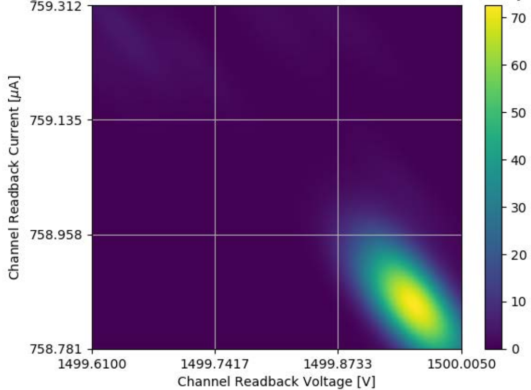
Voltage and Current Readback for Module #128 Channel 04 Stability Test
