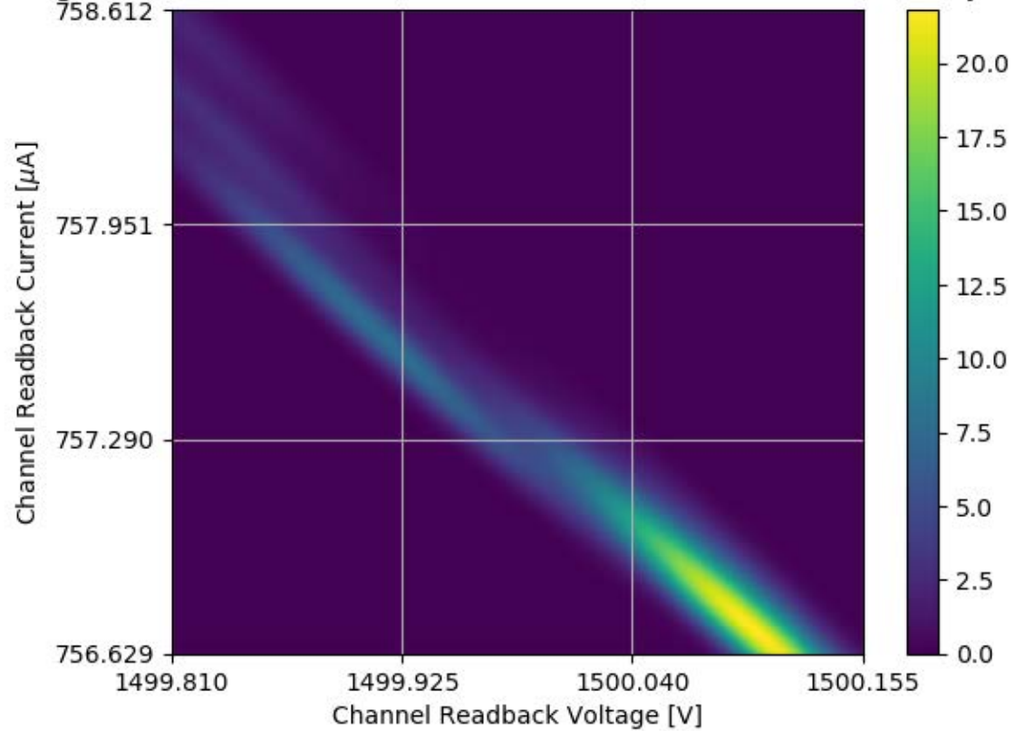
Voltage and Current Readback for Module #128 Channel 18 Stability Test
