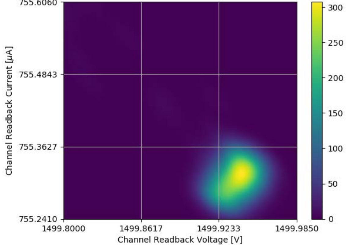
Voltage and Current Readback for Module #128 Channel 31 Stability Test
