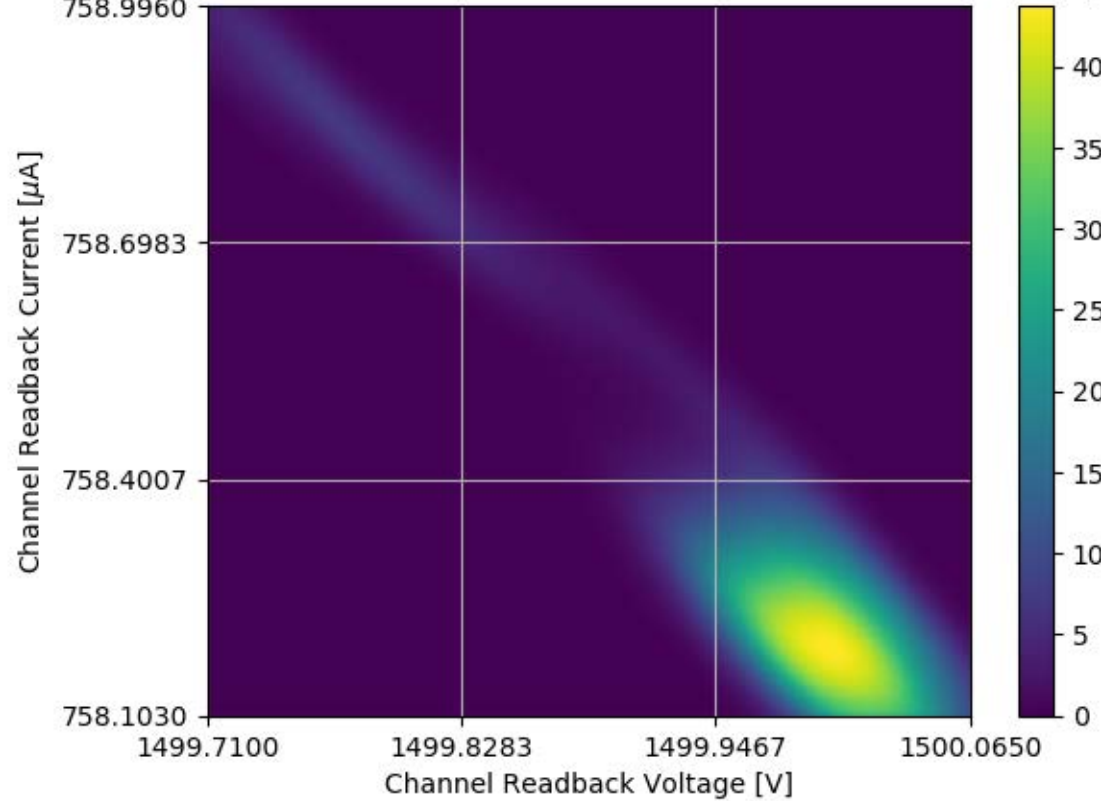
Voltage and Current Readback for Module #128 Channel 29 Stability Test
