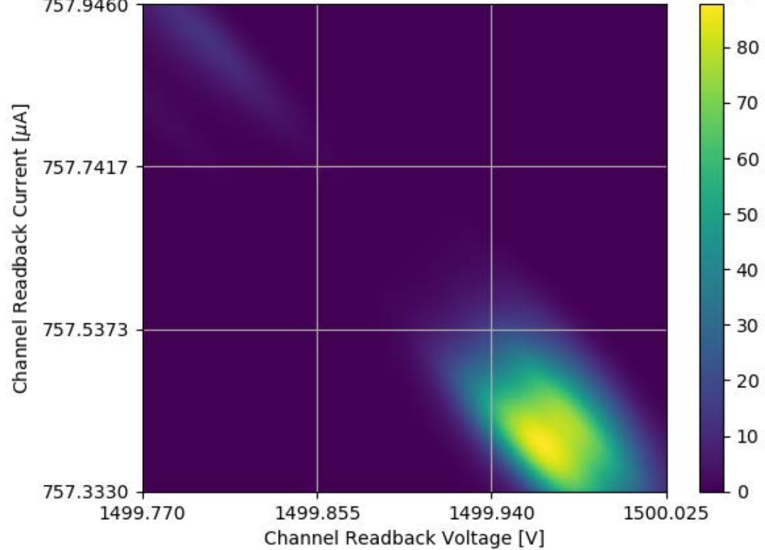
Voltage and Current Readback for Module #128 Channel 32 Stability Test
