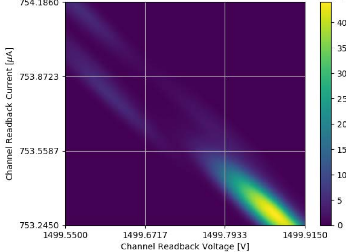
Voltage and Current Readback for Module #128 Channel 11 Stability Test
