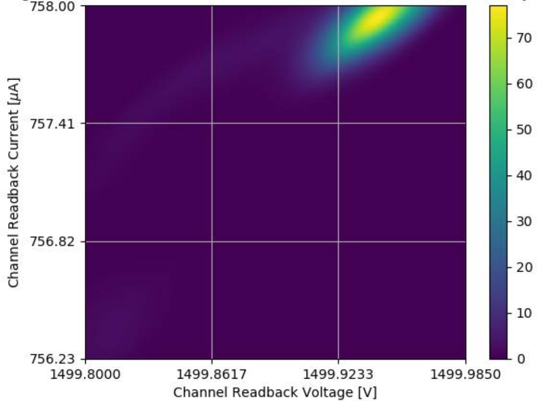
Voltage and Current Readback for Module #128 Channel 08 Stability Test
