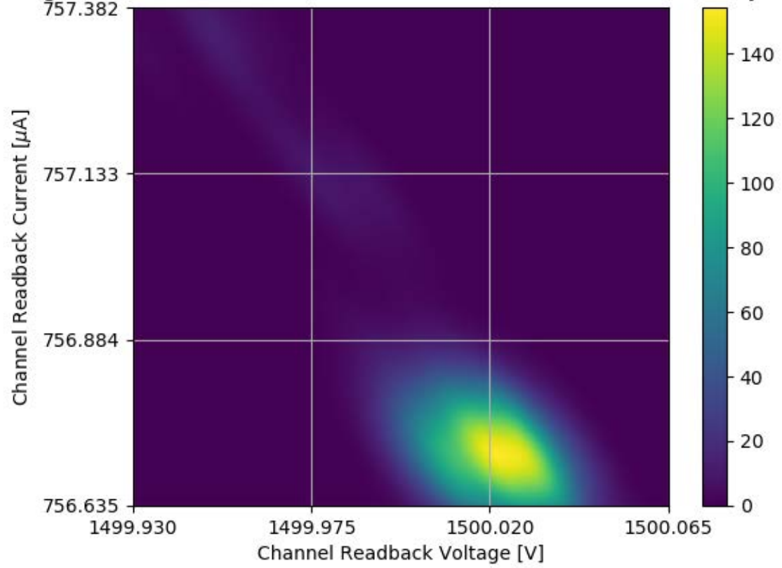
Voltage and Current Readback for Module #128 Channel 20 Stability Test
