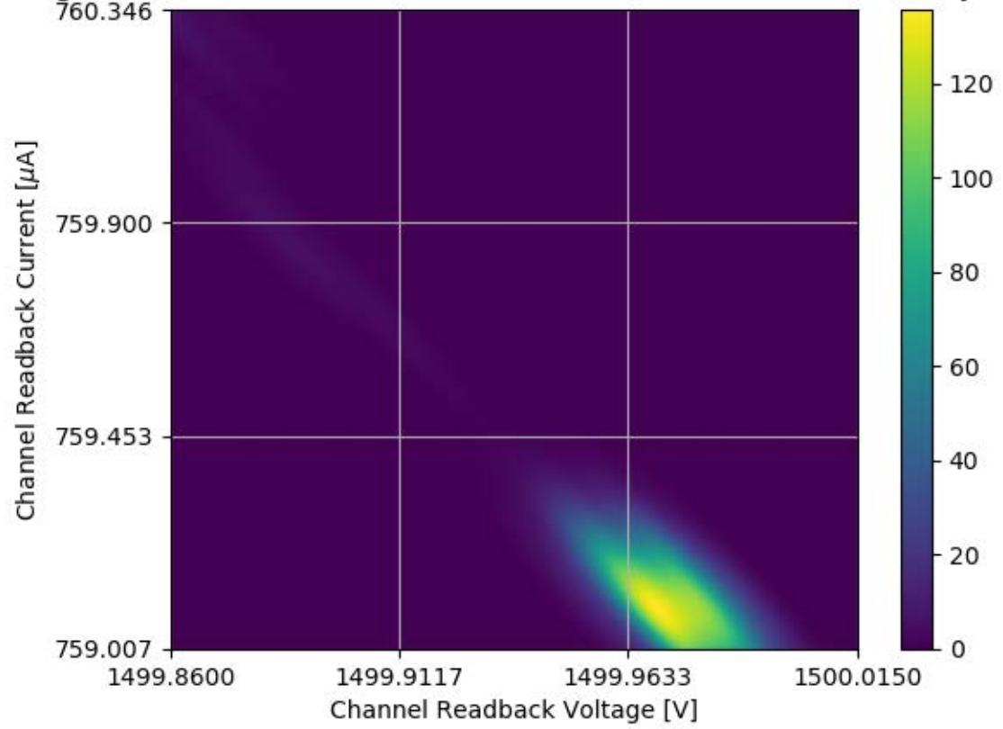
Voltage and Current Readback for Module #128 Channel 22 Stability Test
