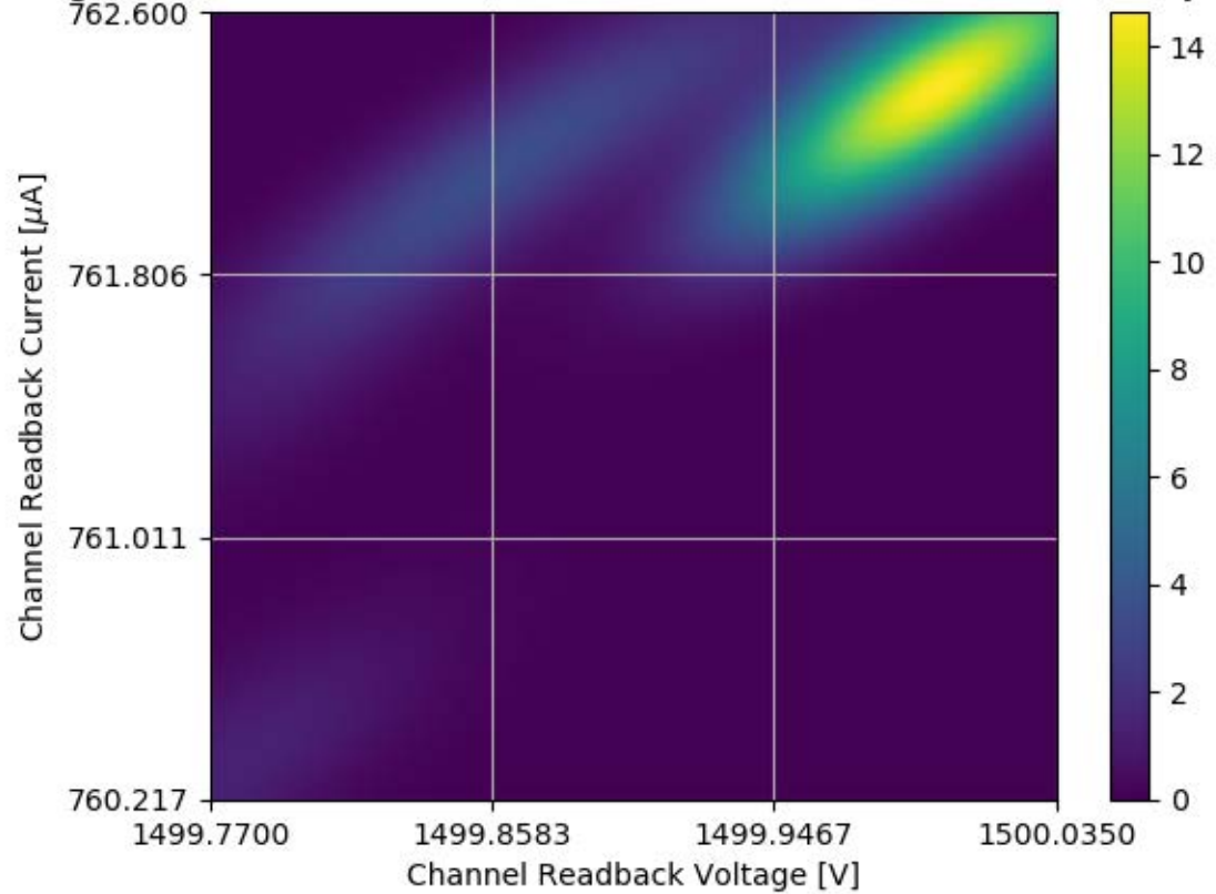
Voltage and Current Readback for Module #128 Channel 09 Stability Test
