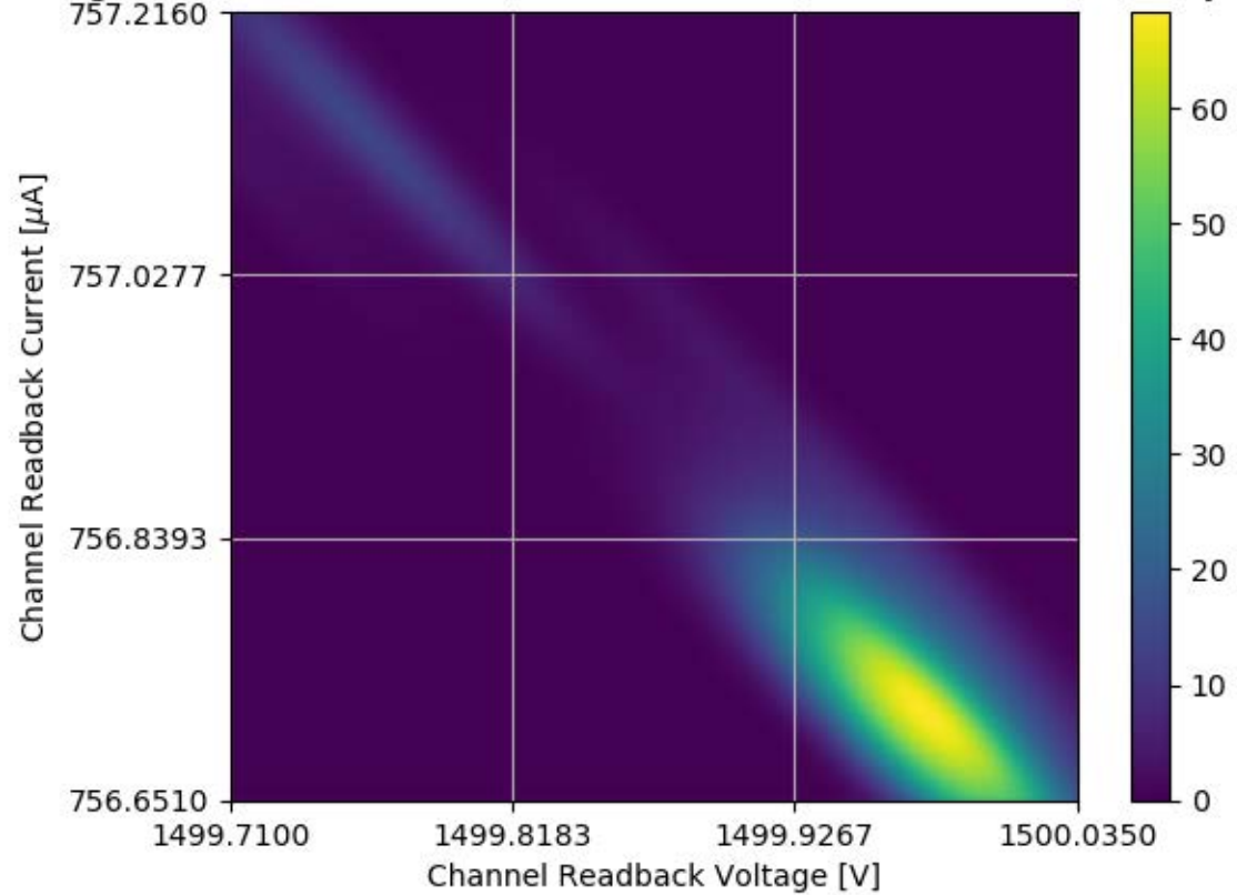
Voltage and Current Readback for Module #128 Channel 23 Stability Test
