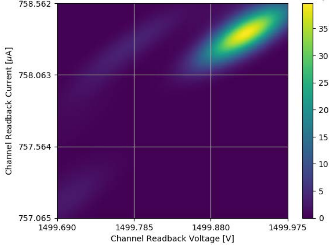
Voltage and Current Readback for Module #128 Channel 24 Stability Test
