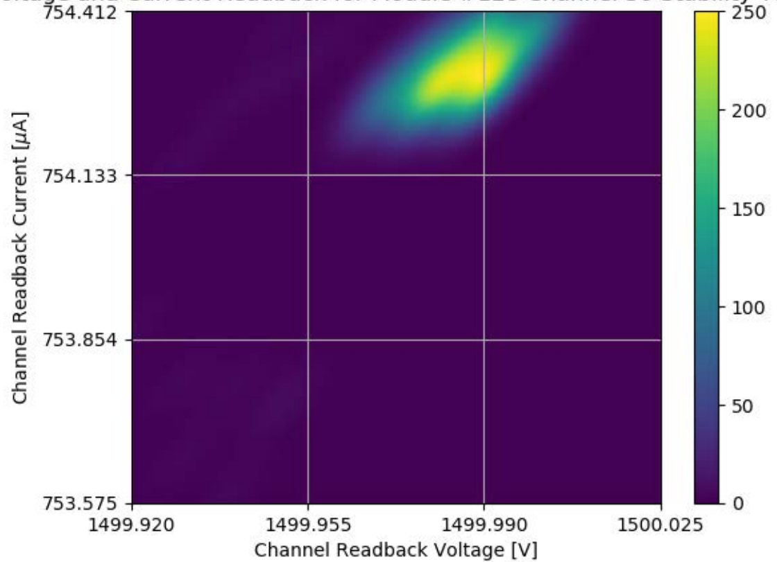
Voltage and Current Readback for Module #128 Channel 30 Stability Test
