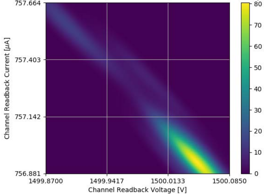
Voltage and Current Readback for Module #128 Channel 27 Stability Test
