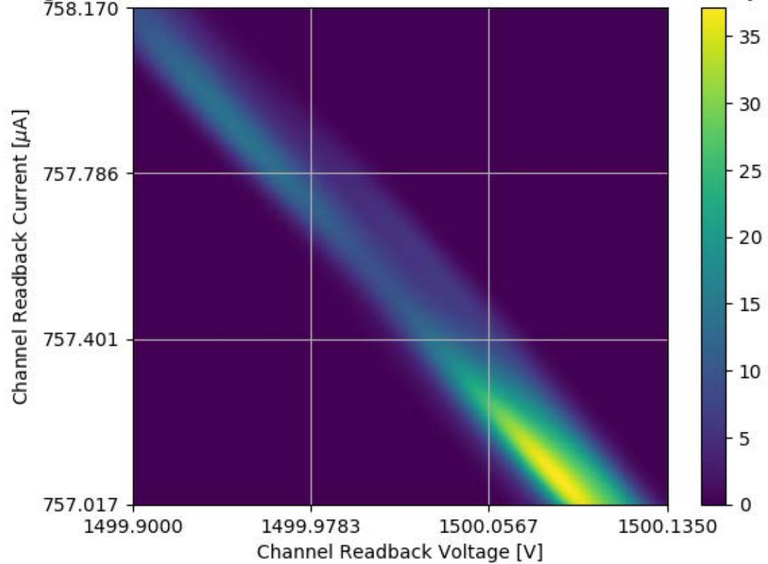
Voltage and Current Readback for Module #128 Channel 21 Stability Test
