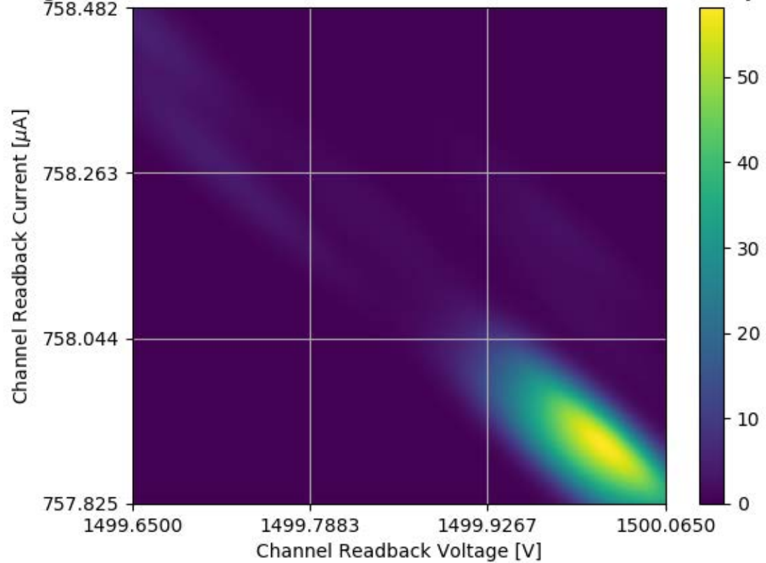
Voltage and Current Readback for Module #128 Channel 06 Stability Test
