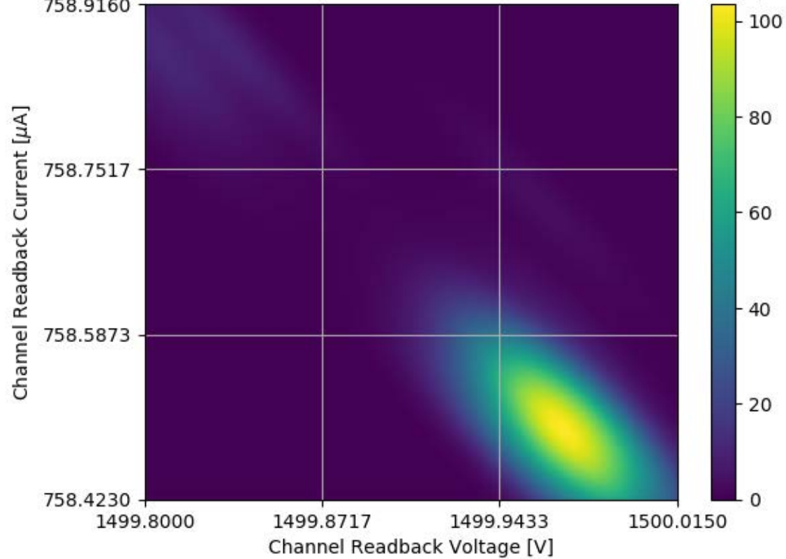
Voltage and Current Readback for Module #128 Channel 16 Stability Test
