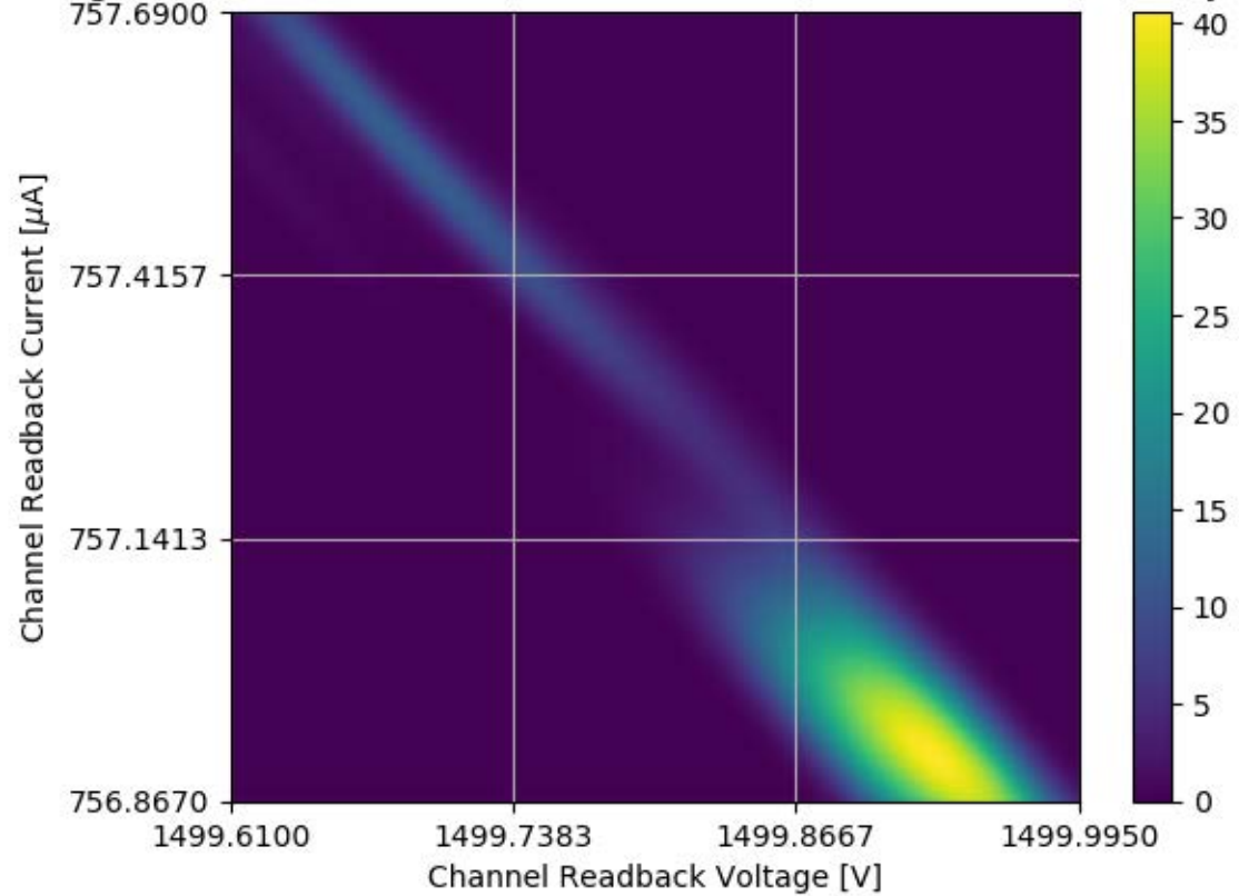
Voltage and Current Readback for Module #128 Channel 34 Stability Test
