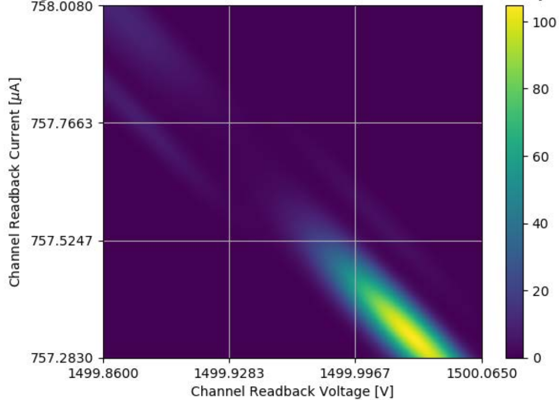
Voltage and Current Readback for Module #128 Channel 07 Stability Test
