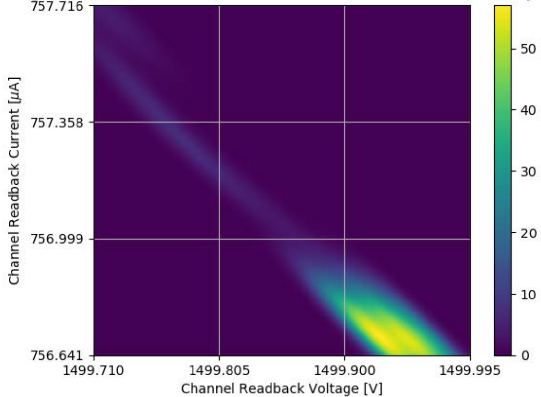
Voltage and Current Readback for Module #128 Channel 28 Stability Test
