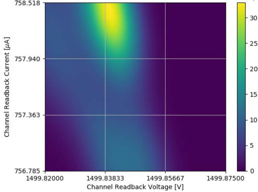
Voltage and Current Readback for Module #128 Channel 25 Stability Test
