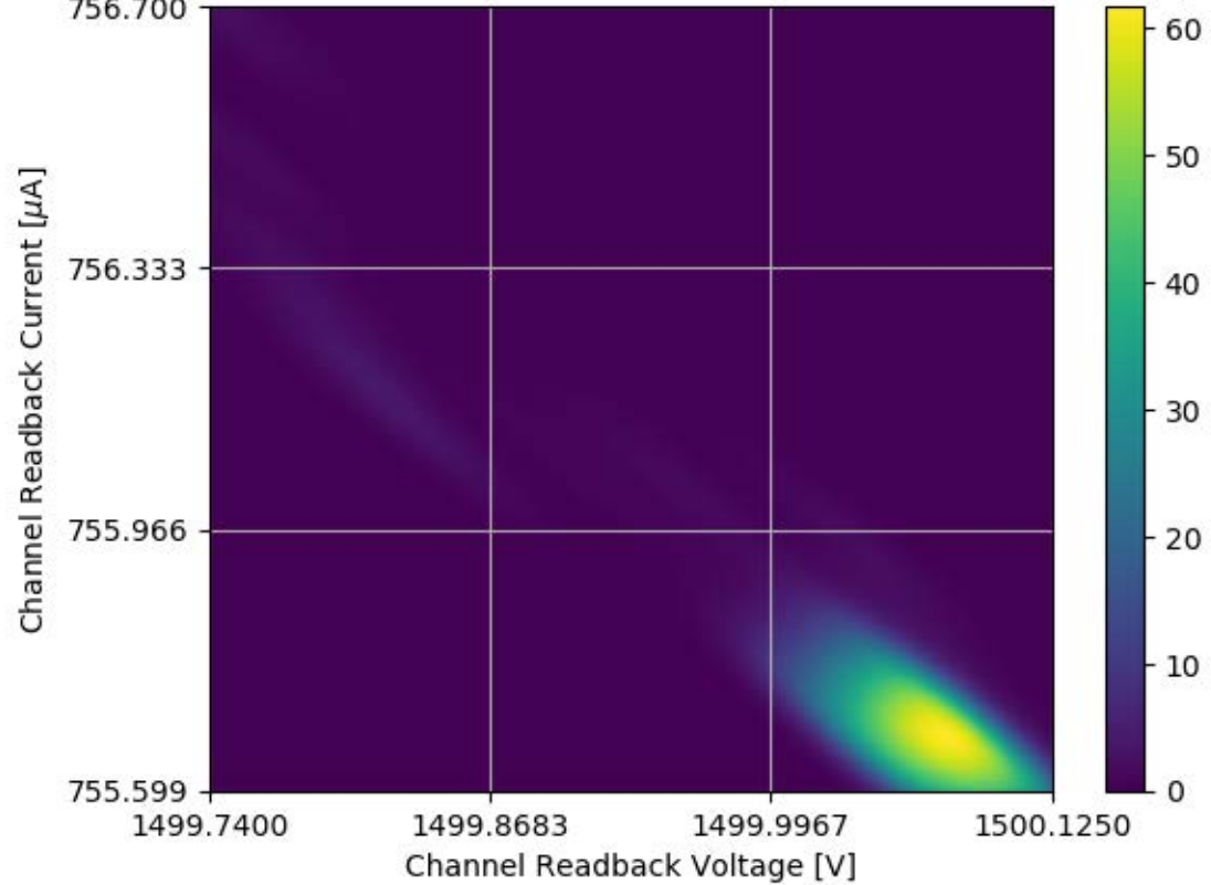
Voltage and Current Readback for Module #128 Channel 03 Stability Test
