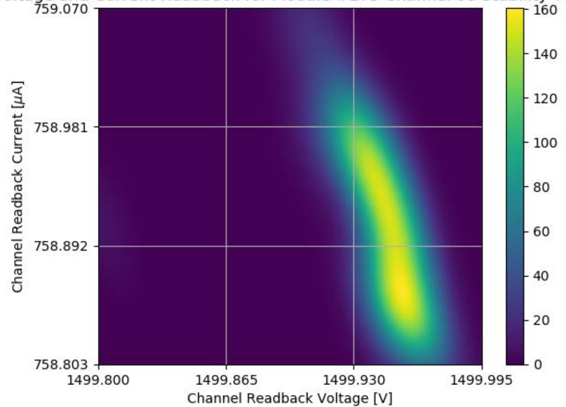
Voltage and Current Readback for Module #173 Channel 08 Stability Test
