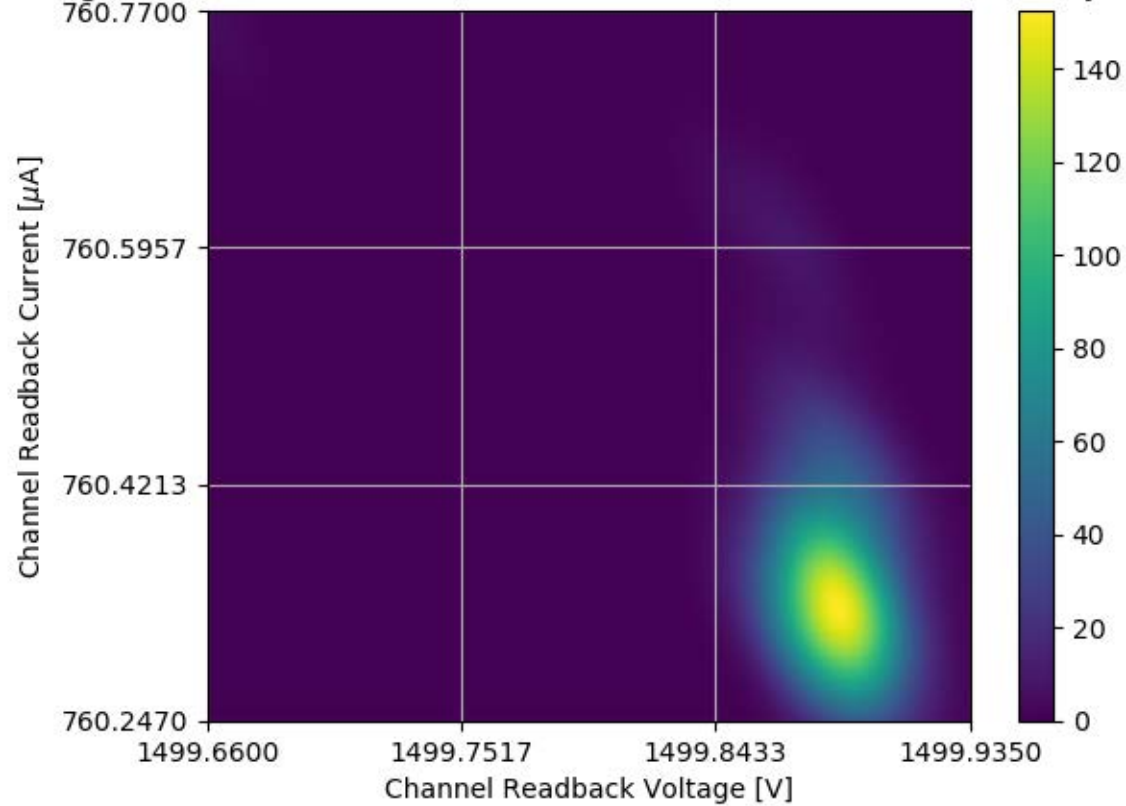
Voltage and Current Readback for Module #173 Channel 12 Stability Test
