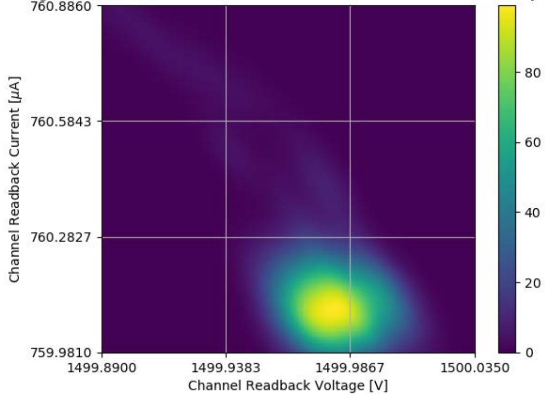
Voltage and Current Readback for Module #173 Channel 22 Stability Test
