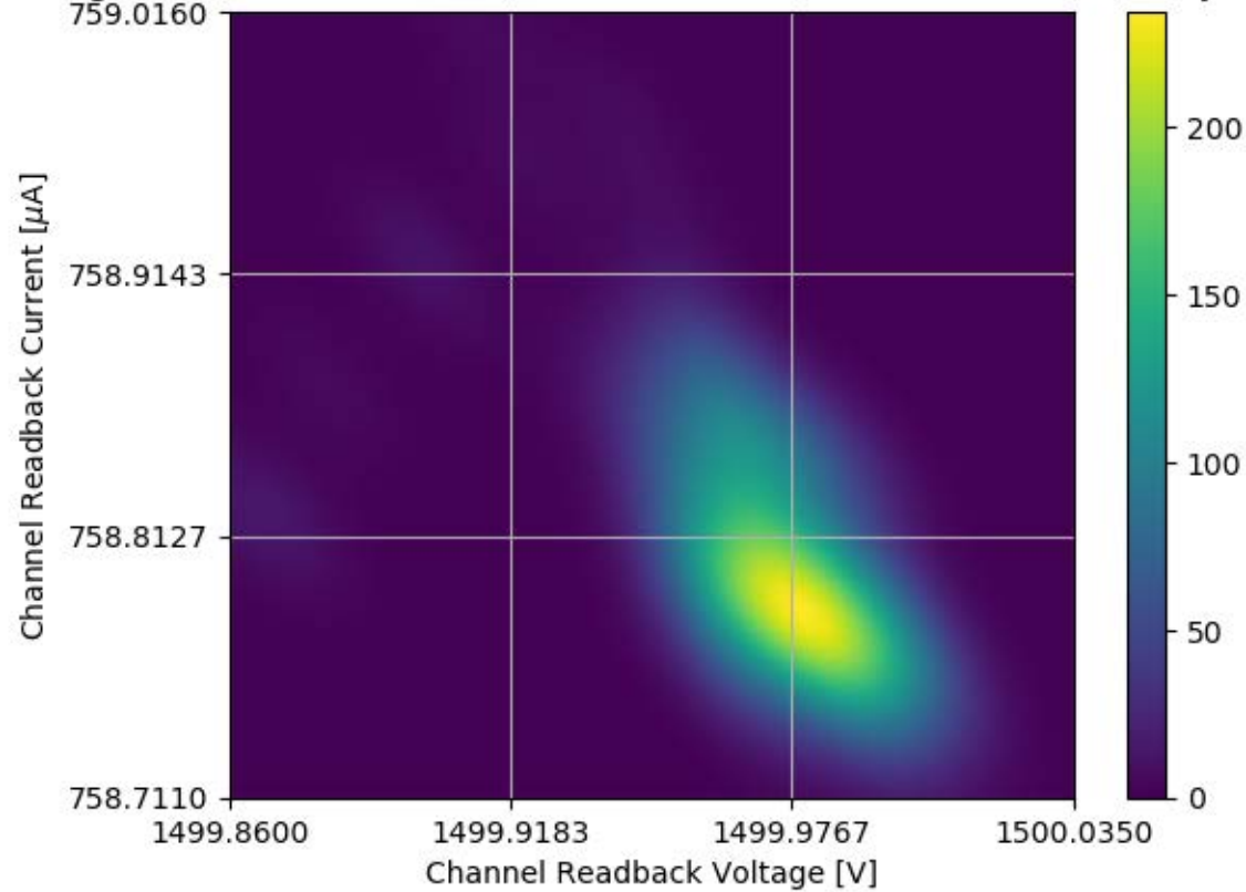
Voltage and Current Readback for Module #173 Channel 26 Stability Test
