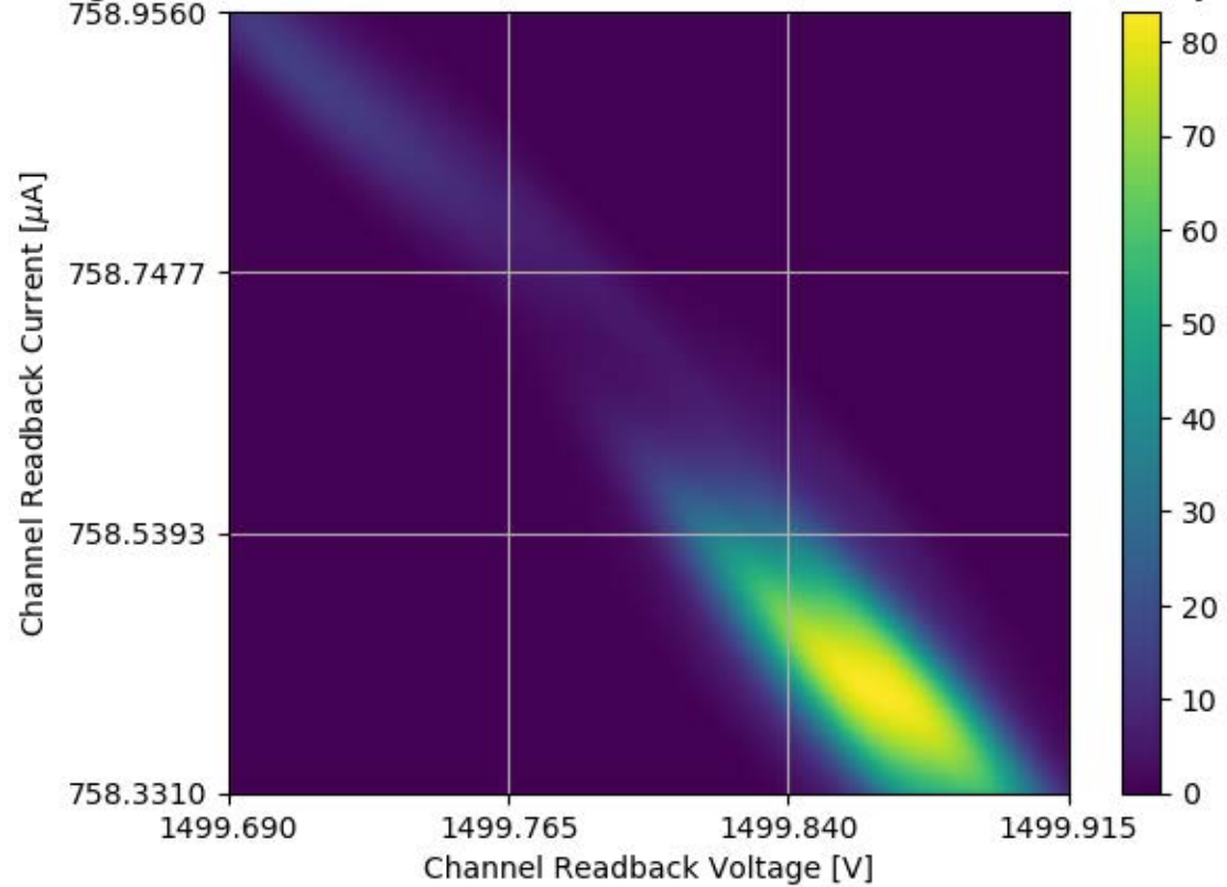
Voltage and Current Readback for Module #173 Channel 21 Stability Test
