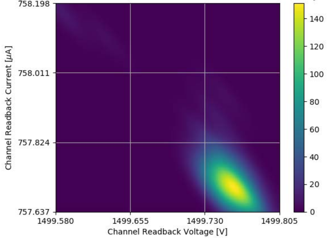
Voltage and Current Readback for Module #173 Channel 14 Stability Test
