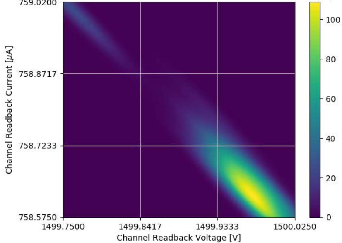
Voltage and Current Readback for Module #173 Channel 06 Stability Test
