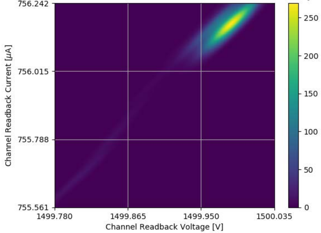
Voltage and Current Readback for Module #173 Channel 03 Stability Test
