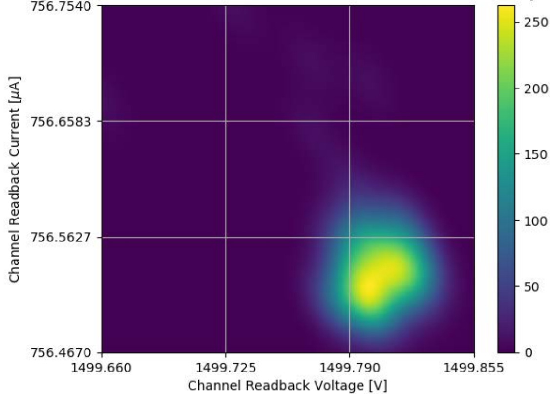
Voltage and Current Readback for Module #173 Channel 15 Stability Test
