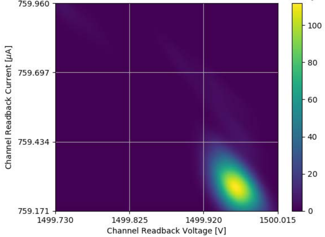
Voltage and Current Readback for Module #173 Channel 05 Stability Test
