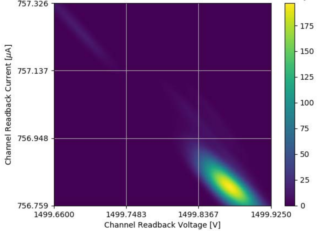
Voltage and Current Readback for Module #173 Channel 01 Stability Test
