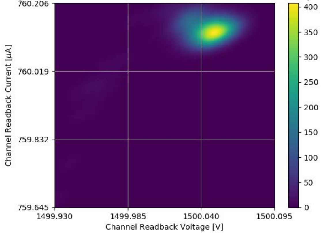
Voltage and Current Readback for Module #173 Channel 10 Stability Test
