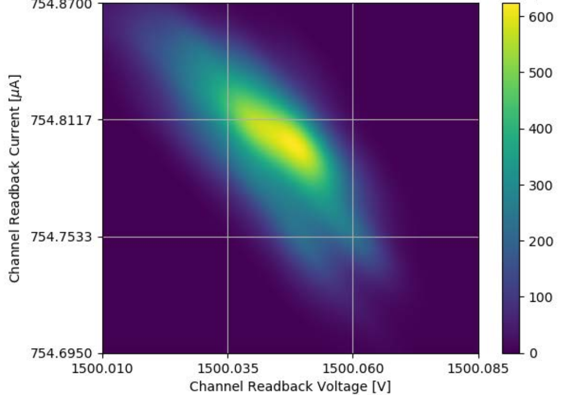
Voltage and Current Readback for Module #173 Channel 30 Stability Test
