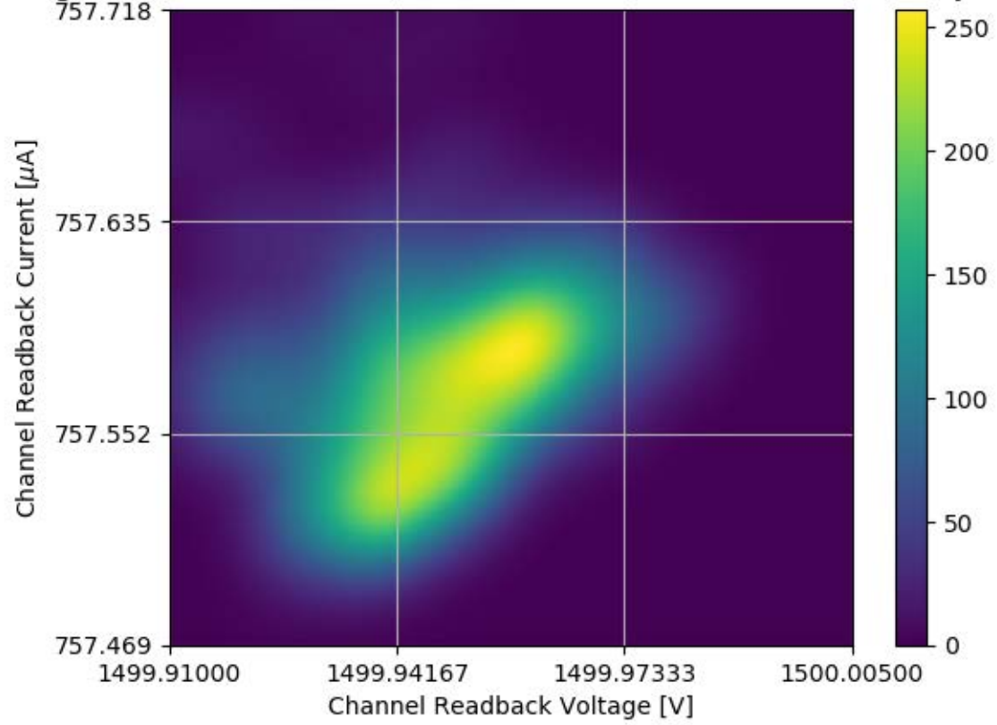
Voltage and Current Readback for Module #173 Channel 20 Stability Test
