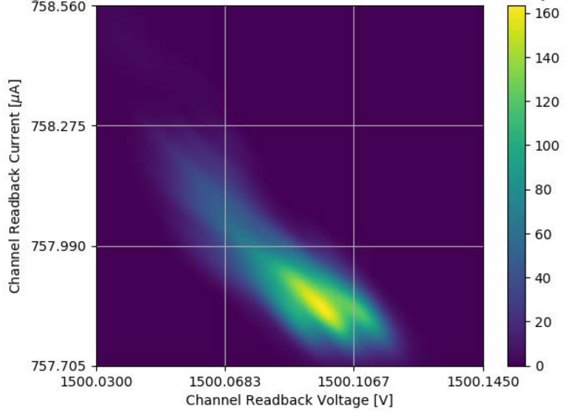
Voltage and Current Readback for Module #173 Channel 34 Stability Test
