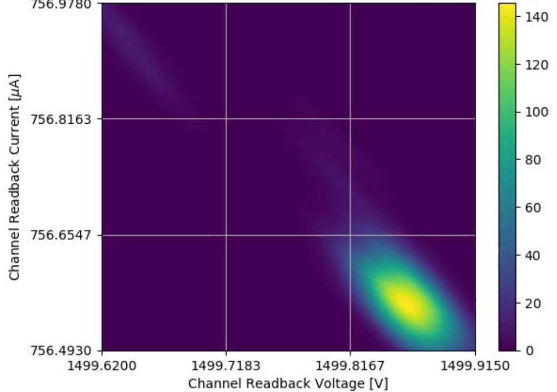
Voltage and Current Readback for Module #173 Channel 18 Stability Test
