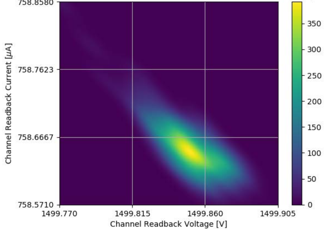
Voltage and Current Readback for Module #173 Channel 16 Stability Test
