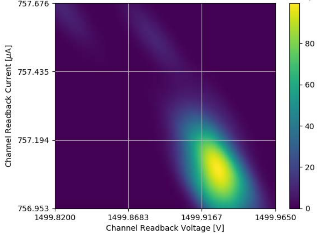
Voltage and Current Readback for Module #173 Channel 17 Stability Test
