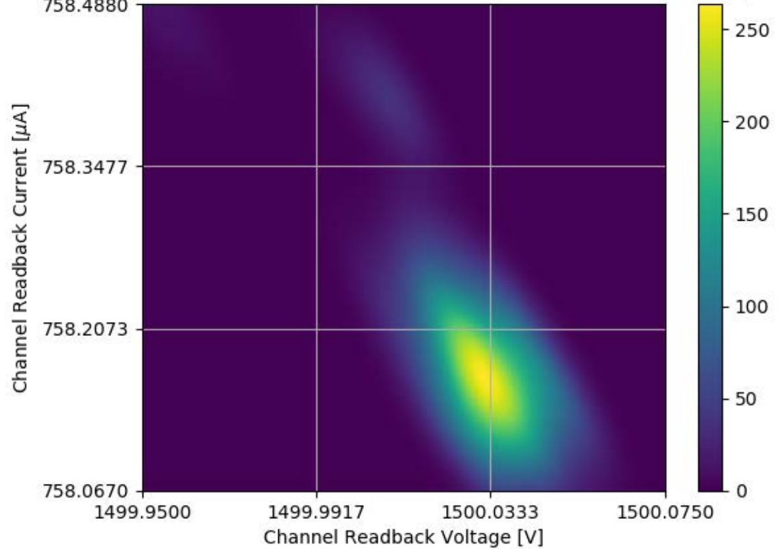
Voltage and Current Readback for Module #173 Channel 32 Stability Test
