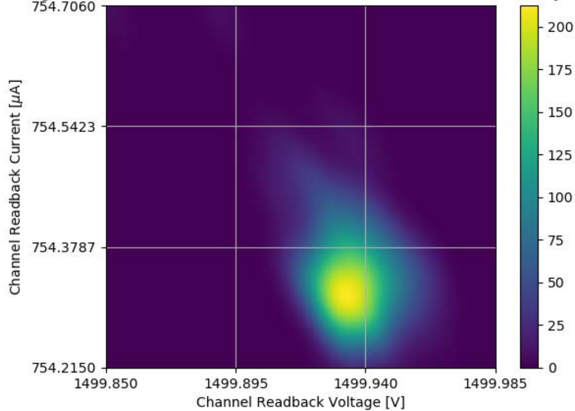
Voltage and Current Readback for Module #173 Channel 33 Stability Test
