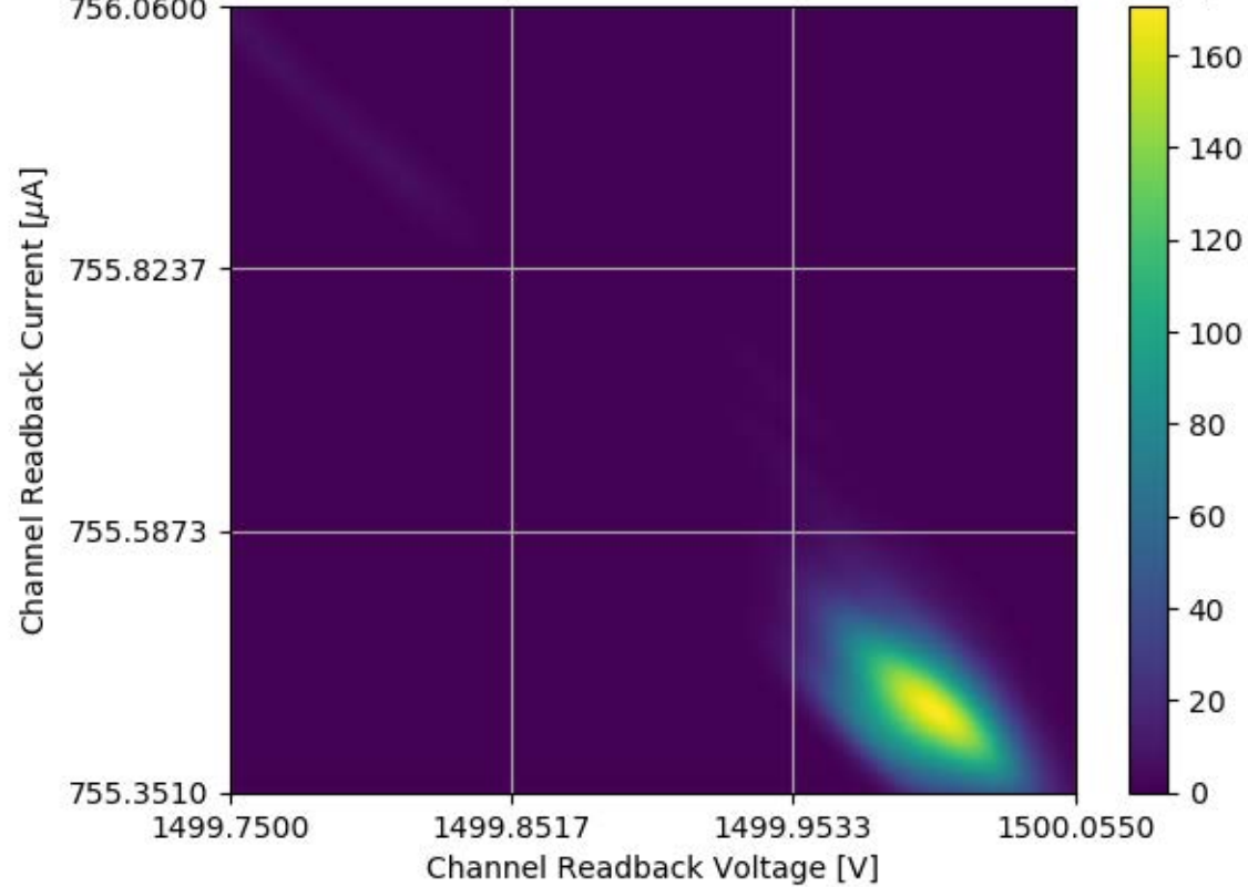
Voltage and Current Readback for Module #173 Channel 13 Stability Test
