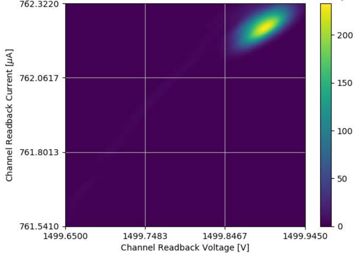
Voltage and Current Readback for Module #173 Channel 09 Stability Test
