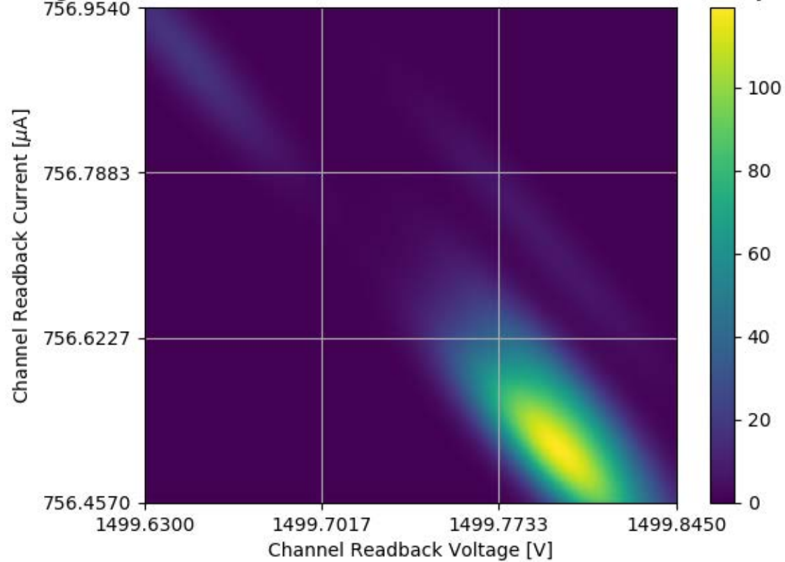
Voltage and Current Readback for Module #173 Channel 02 Stability Test
