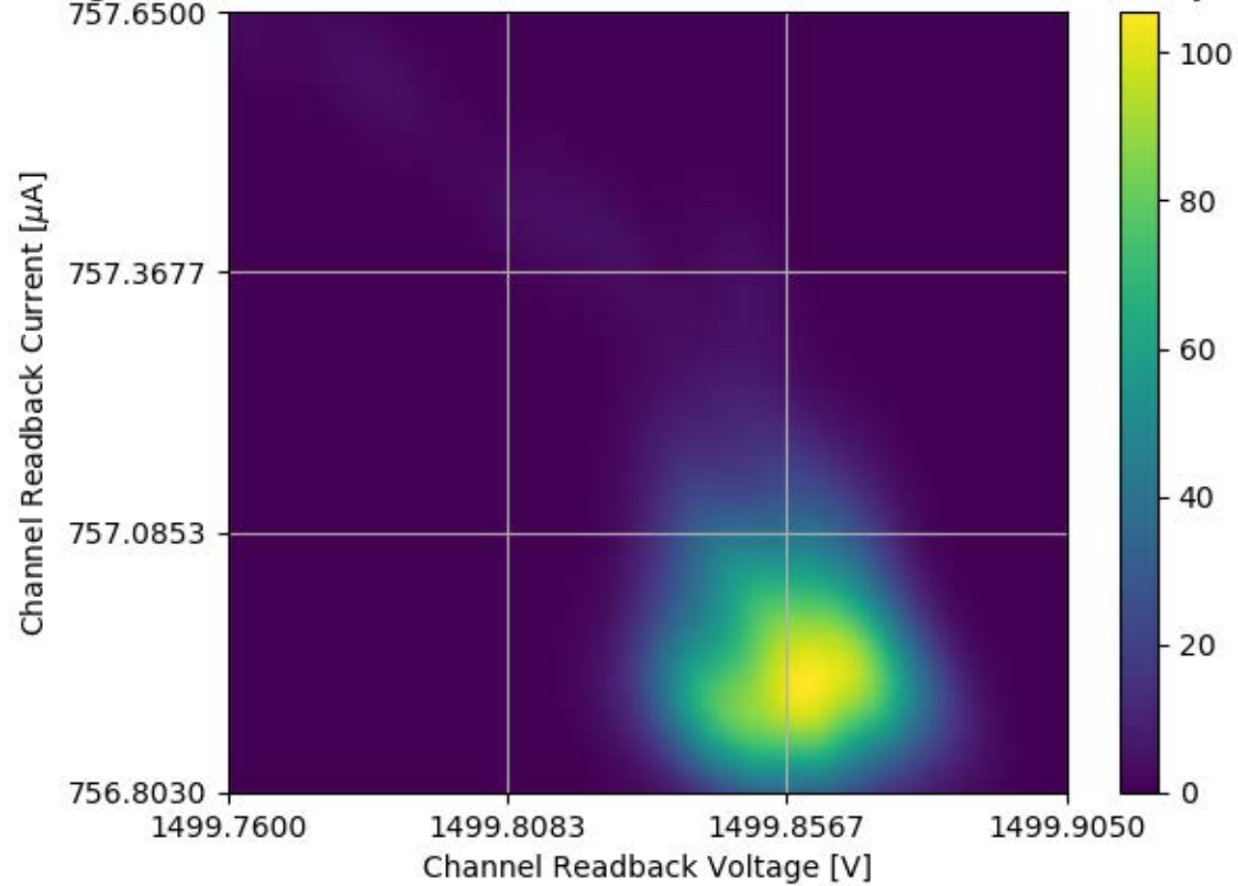
Voltage and Current Readback for Module #173 Channel 28 Stability Test
