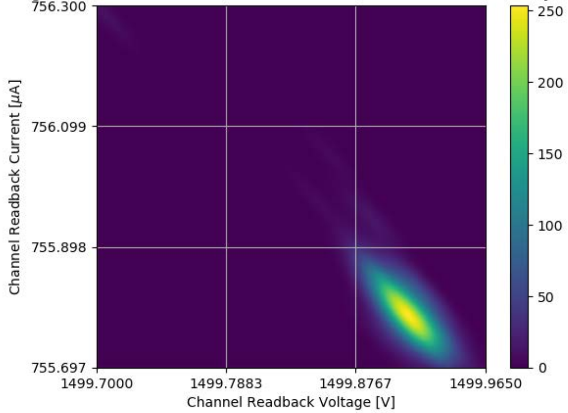
Voltage and Current Readback for Module #173 Channel 00 Stability Test
