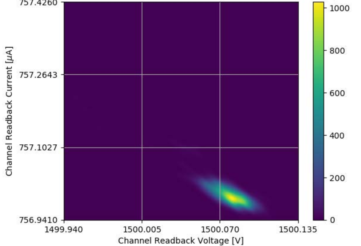
Voltage and Current Readback for Module #256 Channel 06 Stability Test
