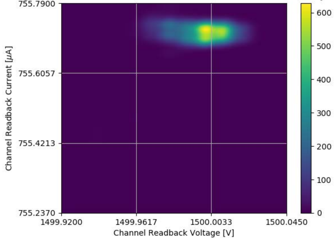
Voltage and Current Readback for Module #256 Channel 01 Stability Test
