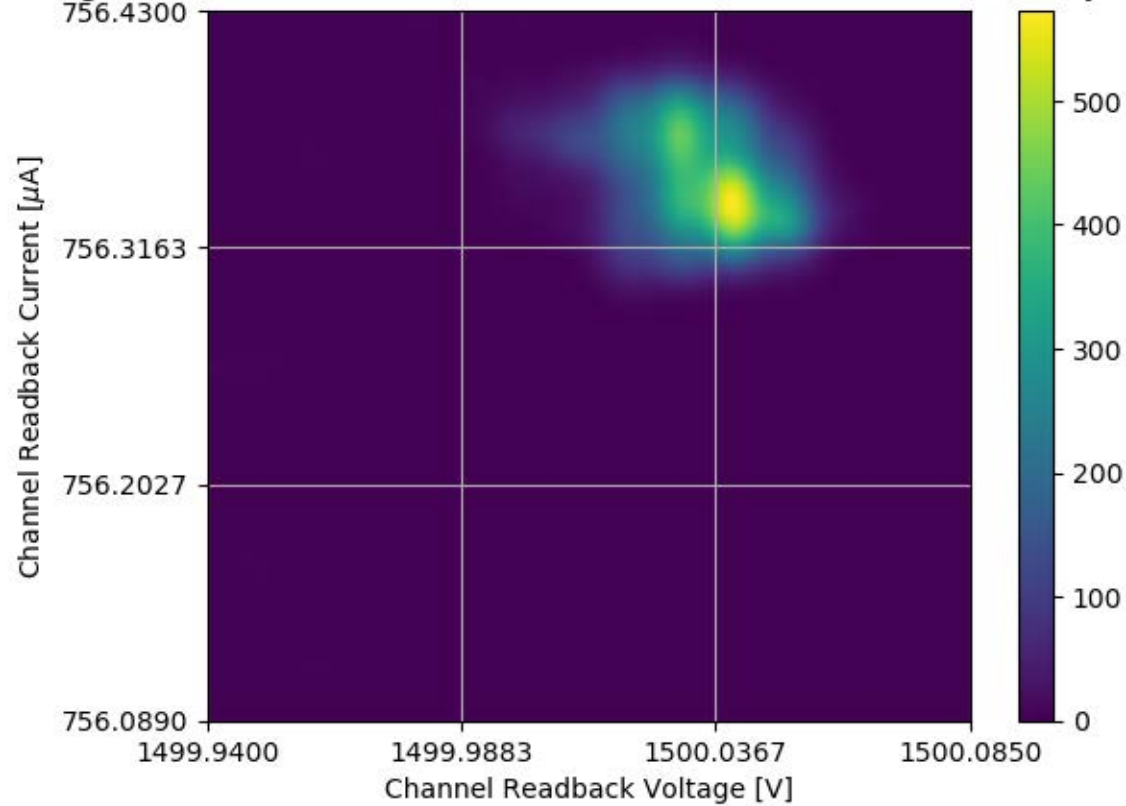
Voltage and Current Readback for Module #256 Channel 27 Stability Test
