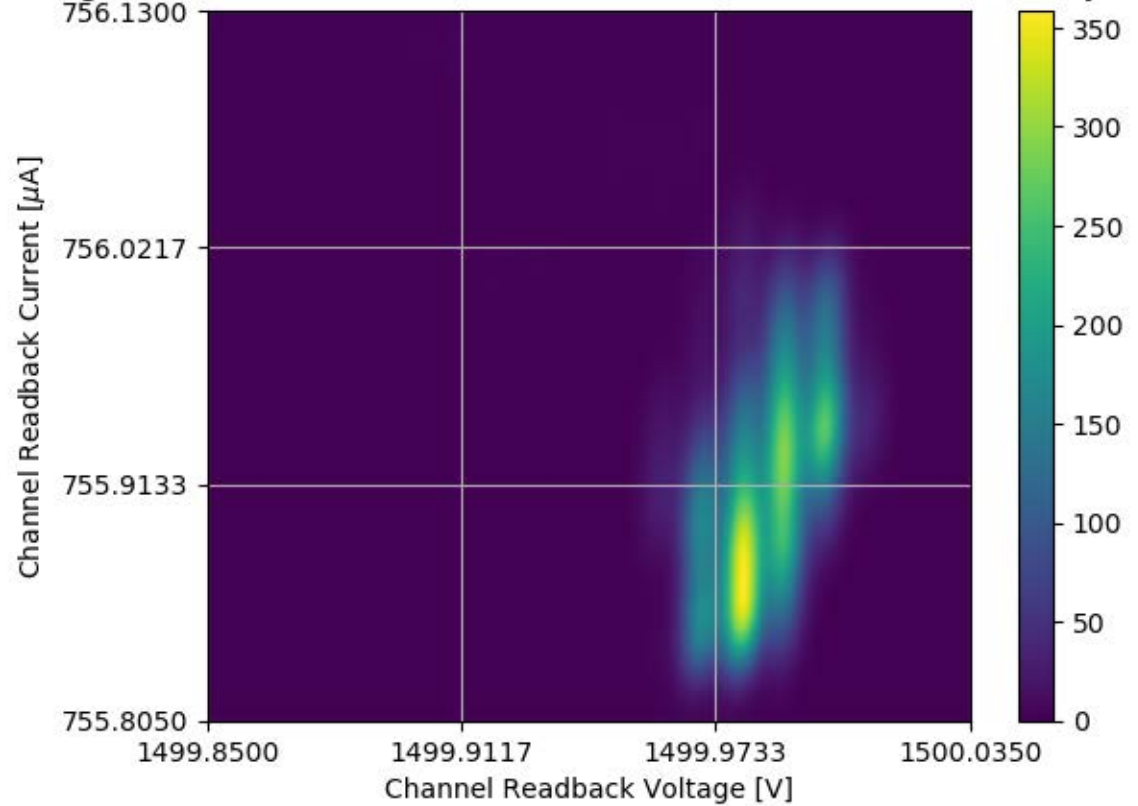
Voltage and Current Readback for Module #256 Channel 28 Stability Test
