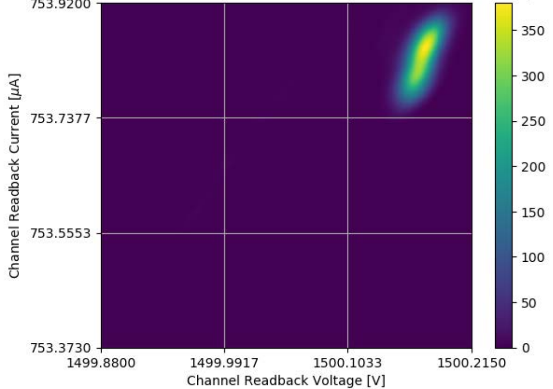
Voltage and Current Readback for Module #256 Channel 00 Stability Test
