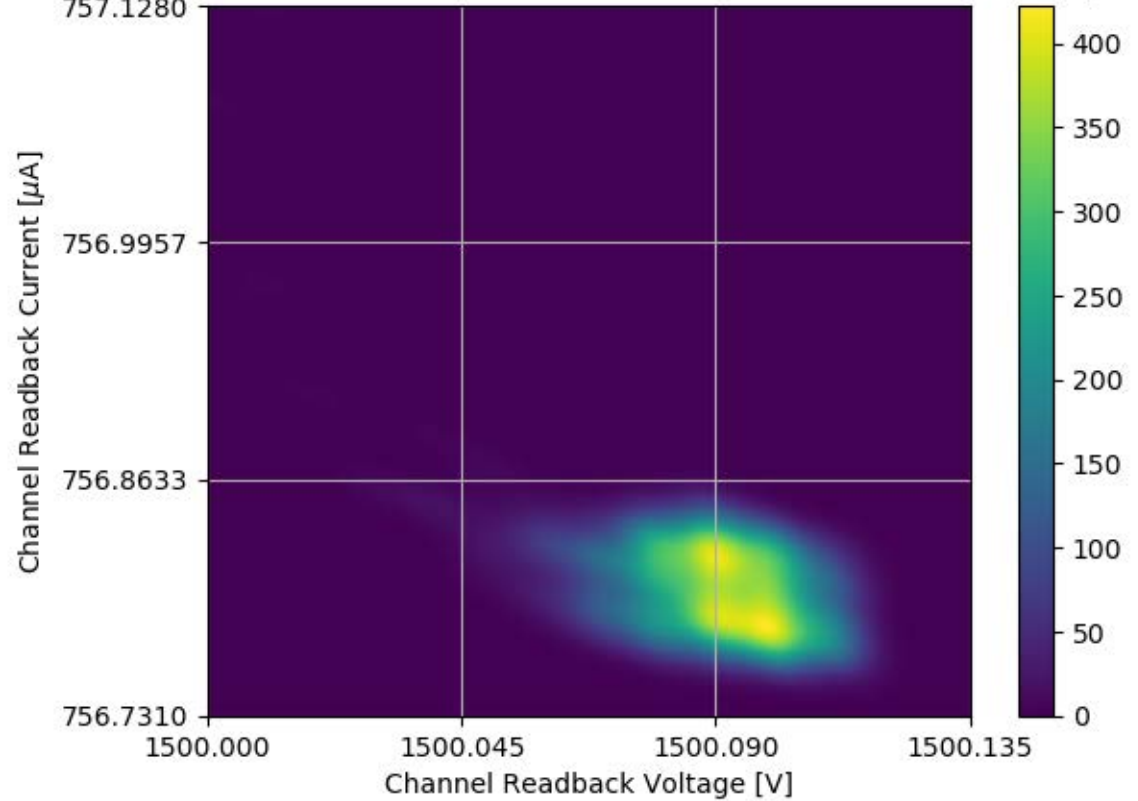
Voltage and Current Readback for Module #256 Channel 20 Stability Test
