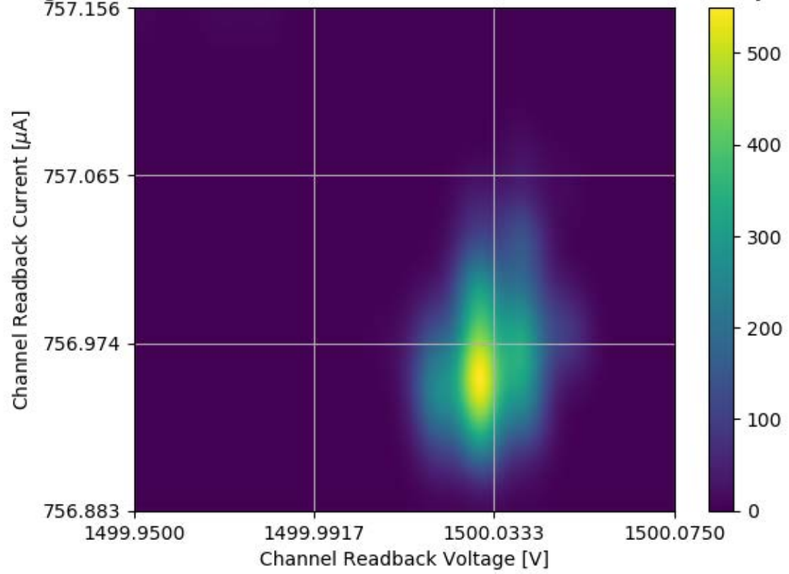
Voltage and Current Readback for Module #256 Channel 16 Stability Test
