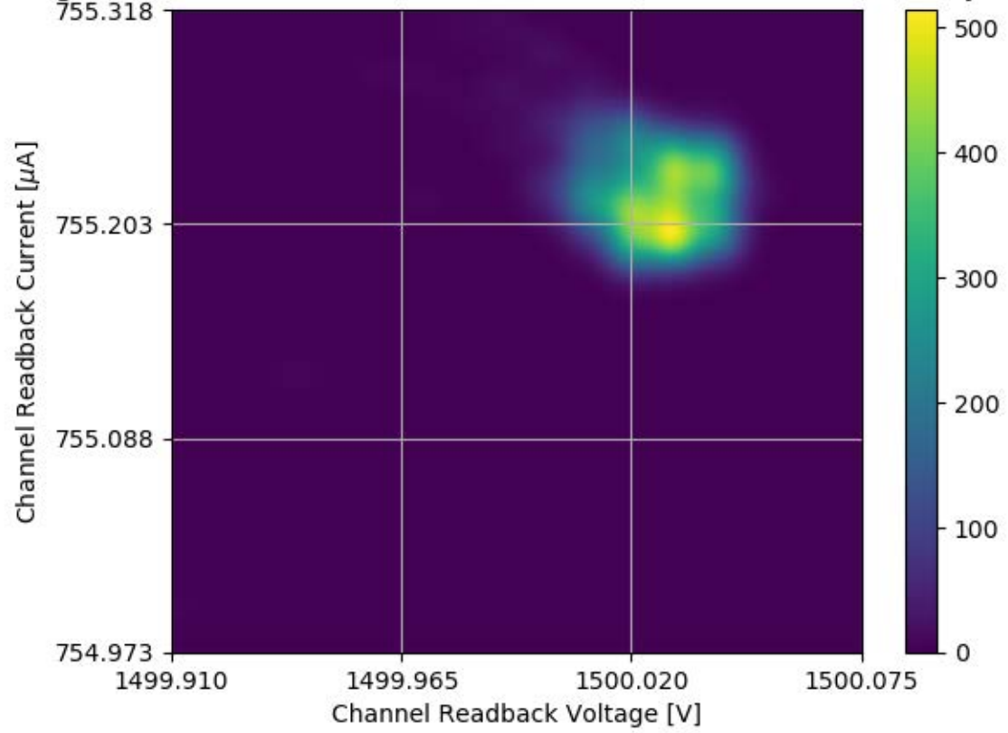
Voltage and Current Readback for Module #256 Channel 03 Stability Test
