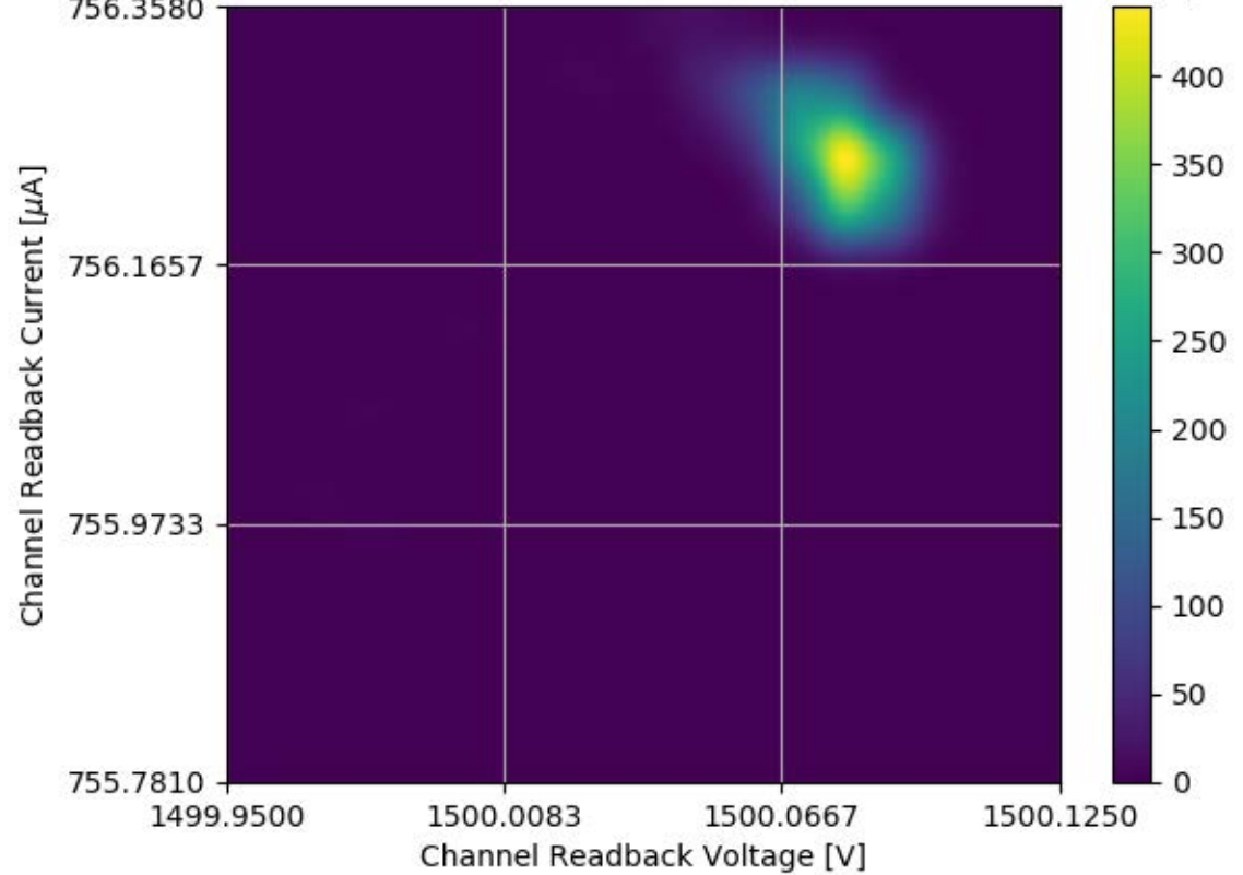
Voltage and Current Readback for Module #256 Channel 17 Stability Test
