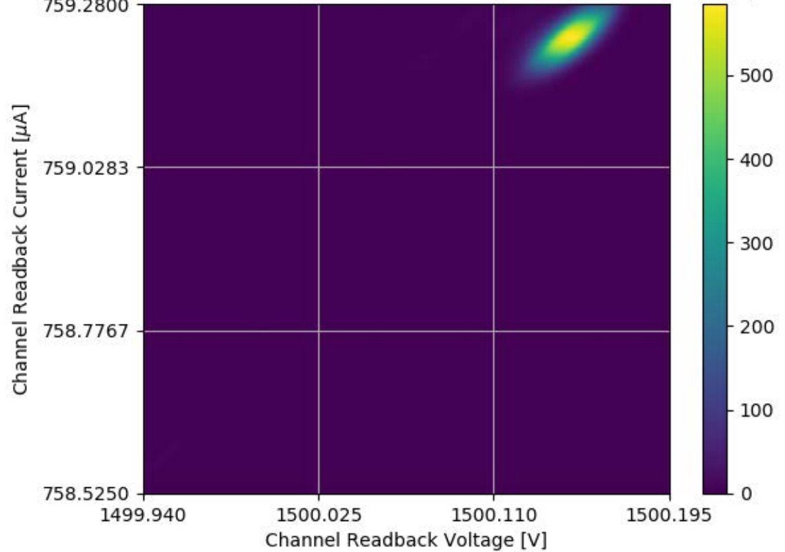
Voltage and Current Readback for Module #256 Channel 12 Stability Test
