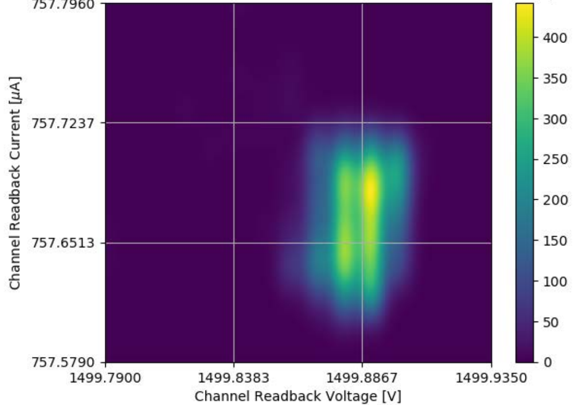
Voltage and Current Readback for Module #256 Channel 21 Stability Test
