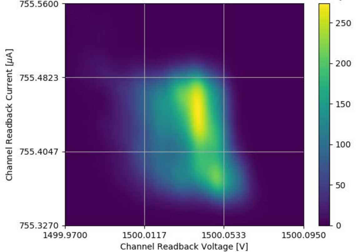
Voltage and Current Readback for Module #256 Channel 23 Stability Test
