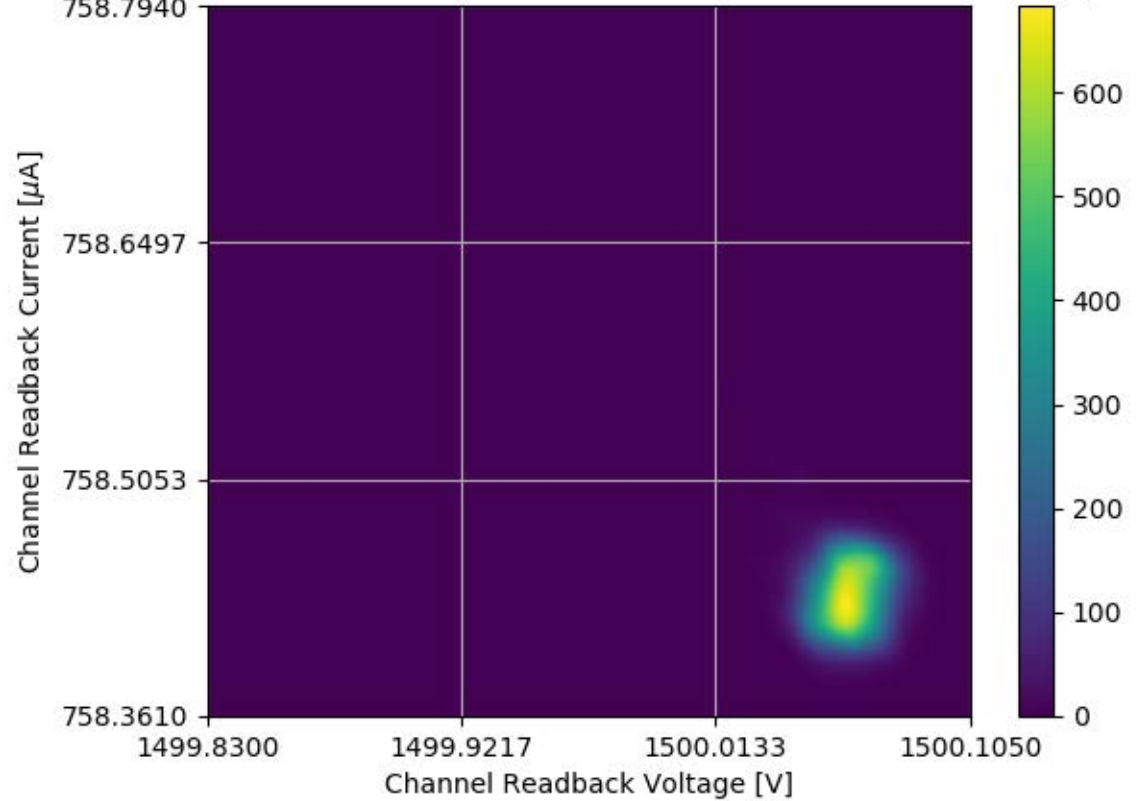
Voltage and Current Readback for Module #256 Channel 05 Stability Test
