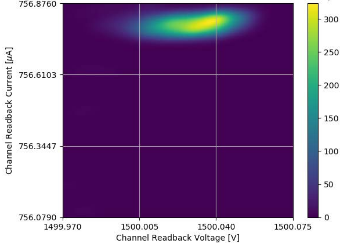
Voltage and Current Readback for Module #256 Channel 15 Stability Test
