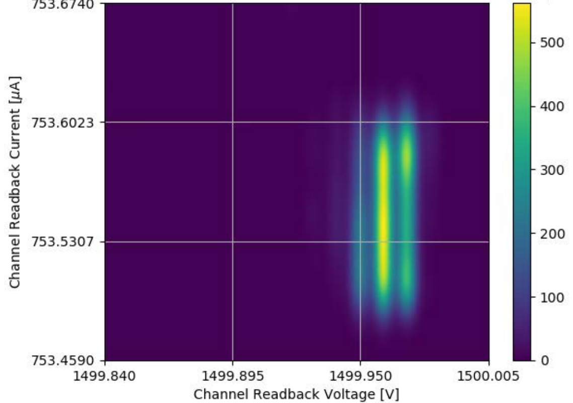
Voltage and Current Readback for Module #256 Channel 33 Stability Test
