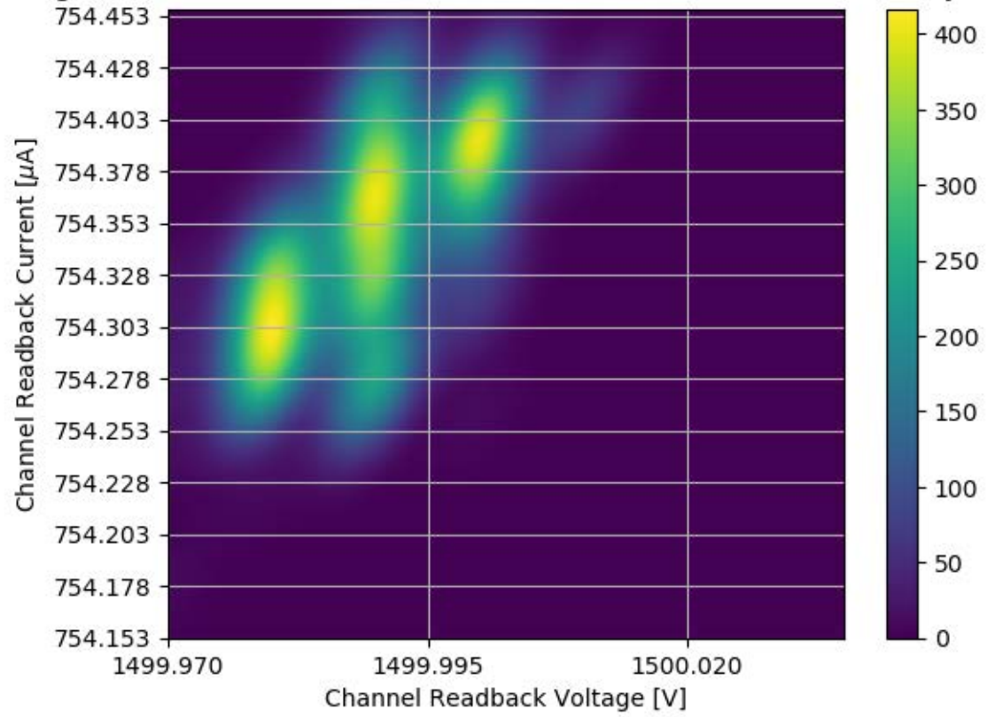
Voltage and Current Readback for Module #262 Channel 30 Stability Test
