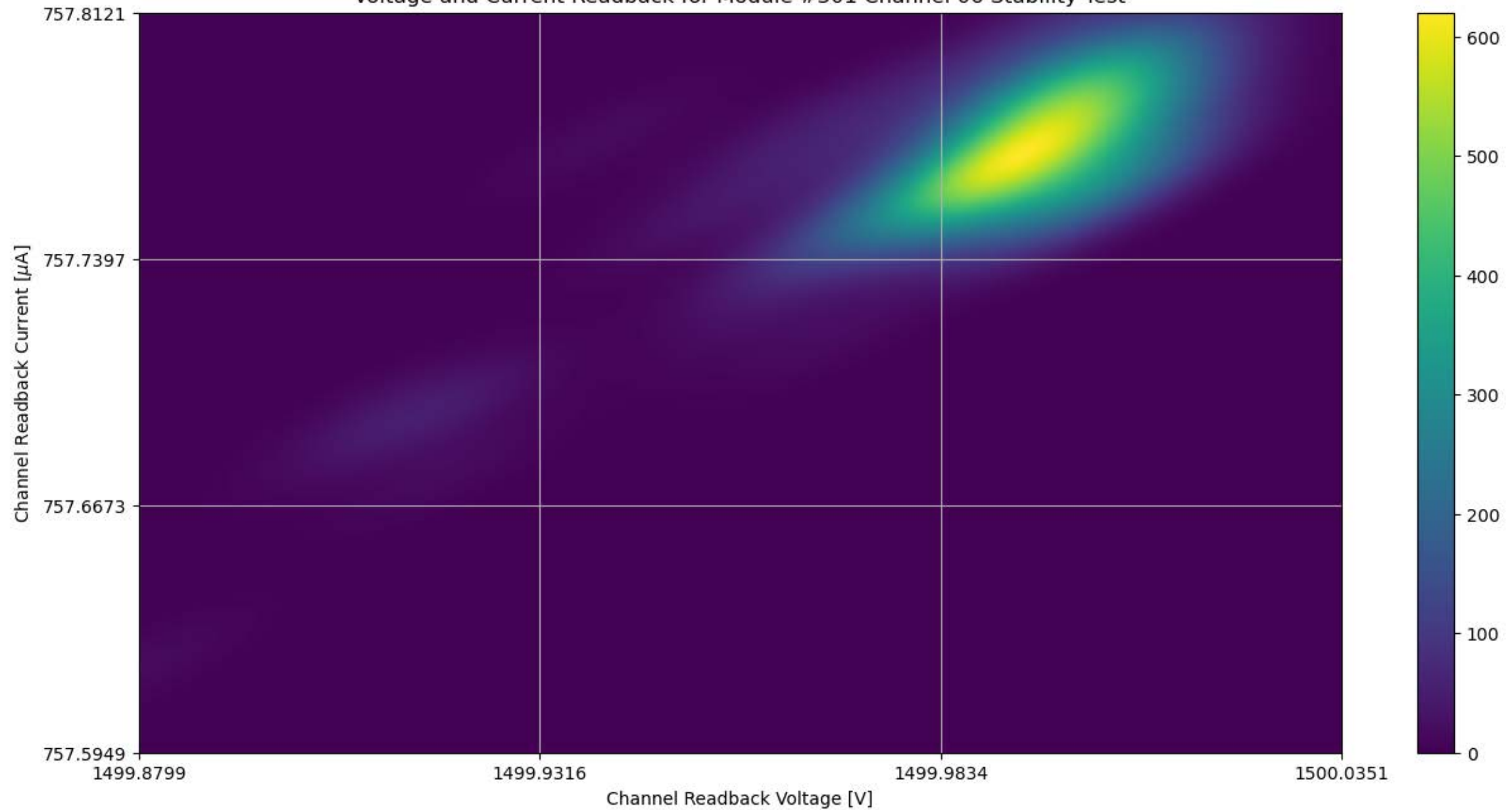
Voltage and Current Readback for Module #301 Channel 06 Stability Test
