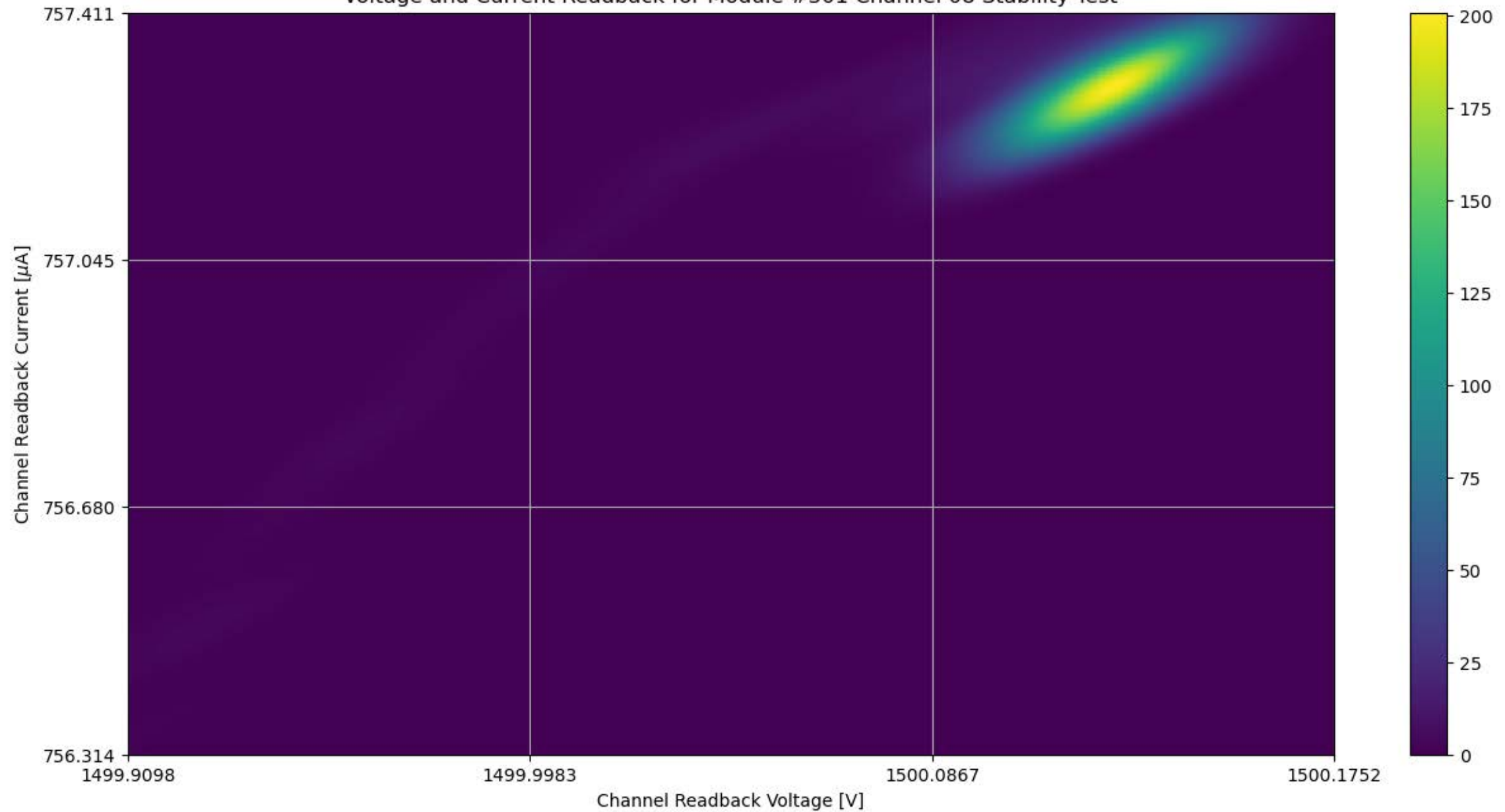
Voltage and Current Readback for Module #301 Channel 08 Stability Test
