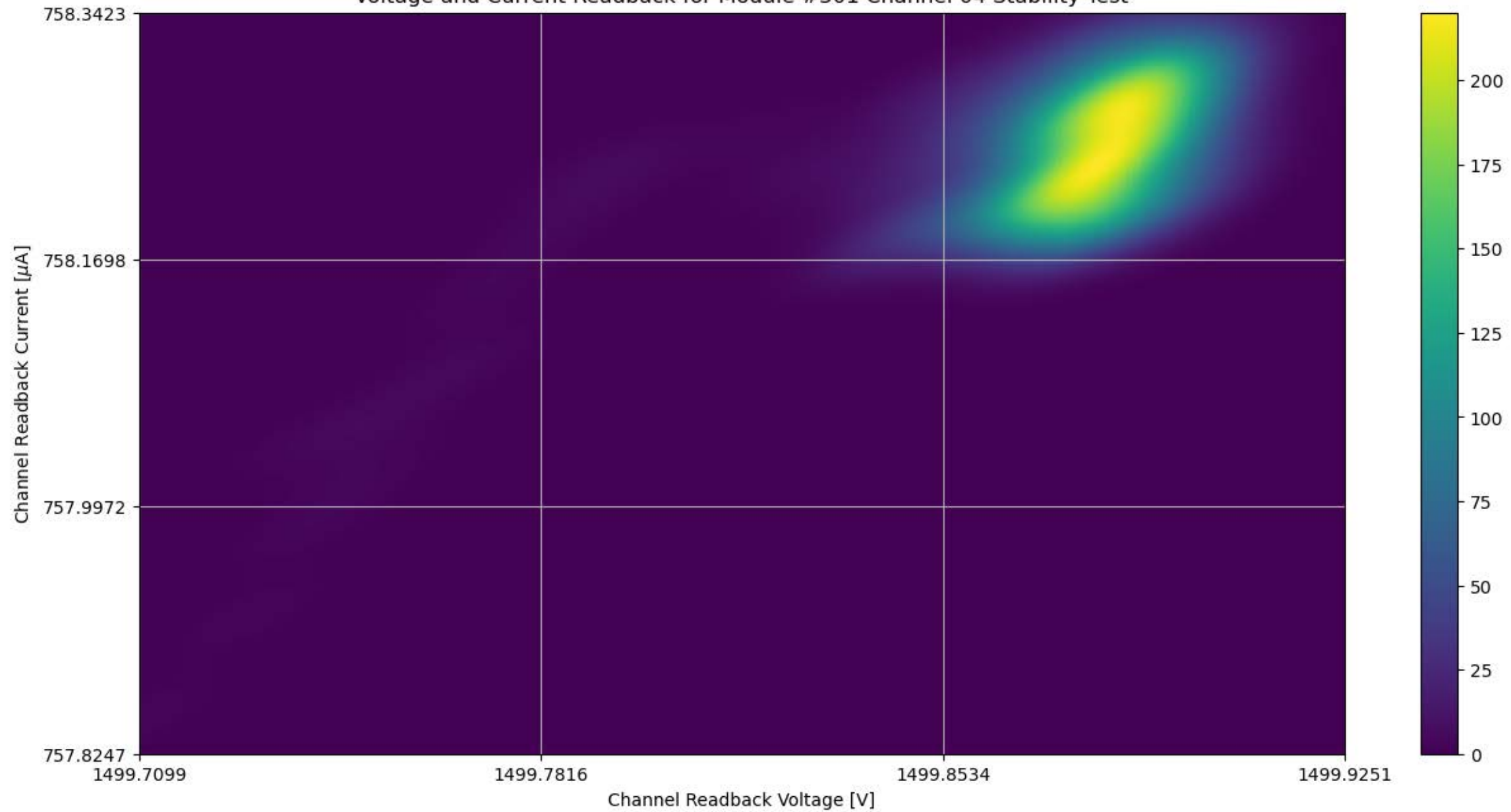
Voltage and Current Readback for Module #301 Channel 04 Stability Test
