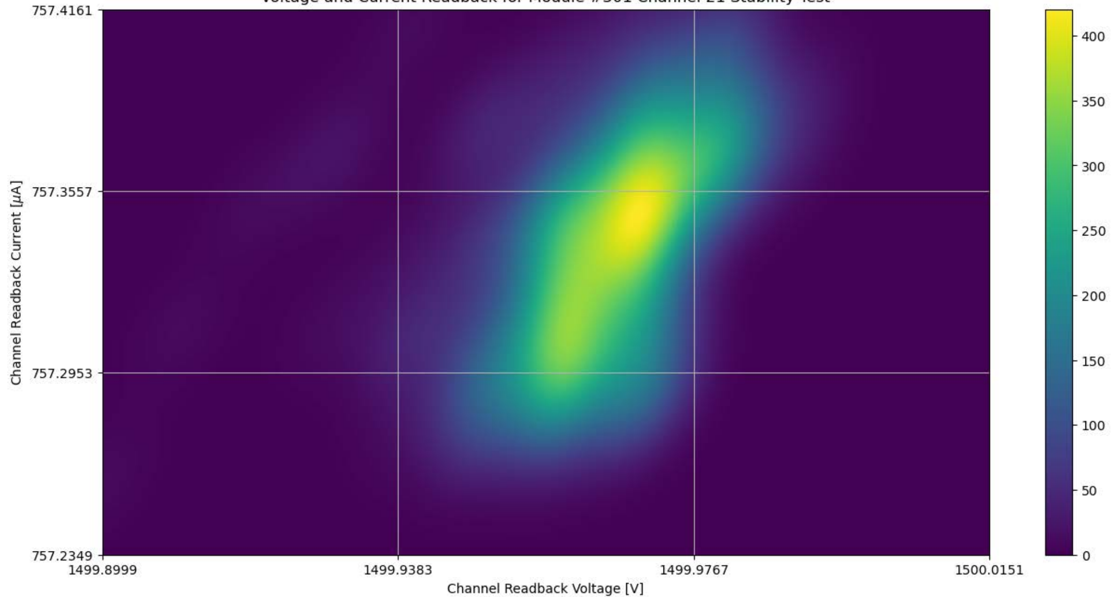
Voltage and Current Readback for Module #301 Channel 21 Stability Test
