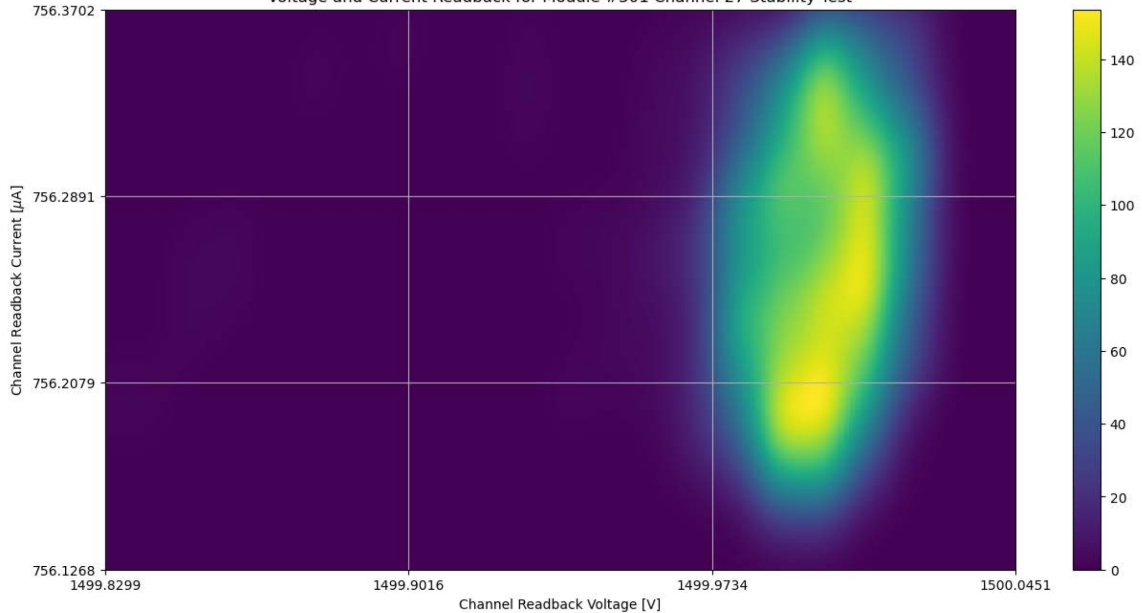
Voltage and Current Readback for Module #301 Channel 27 Stability Test
