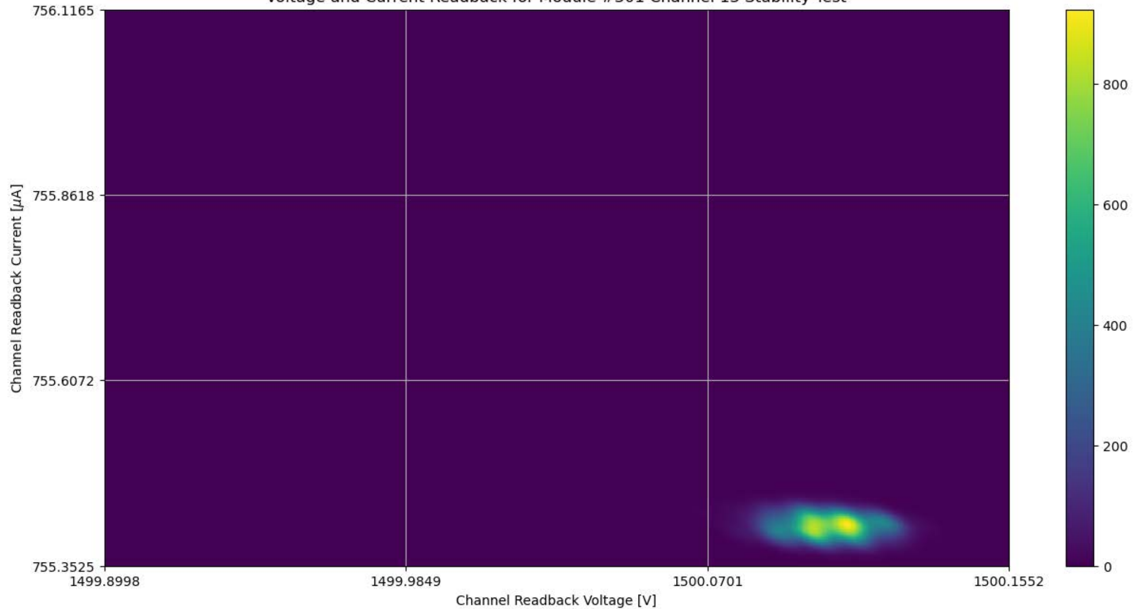
Voltage and Current Readback for Module #301 Channel 13 Stability Test
