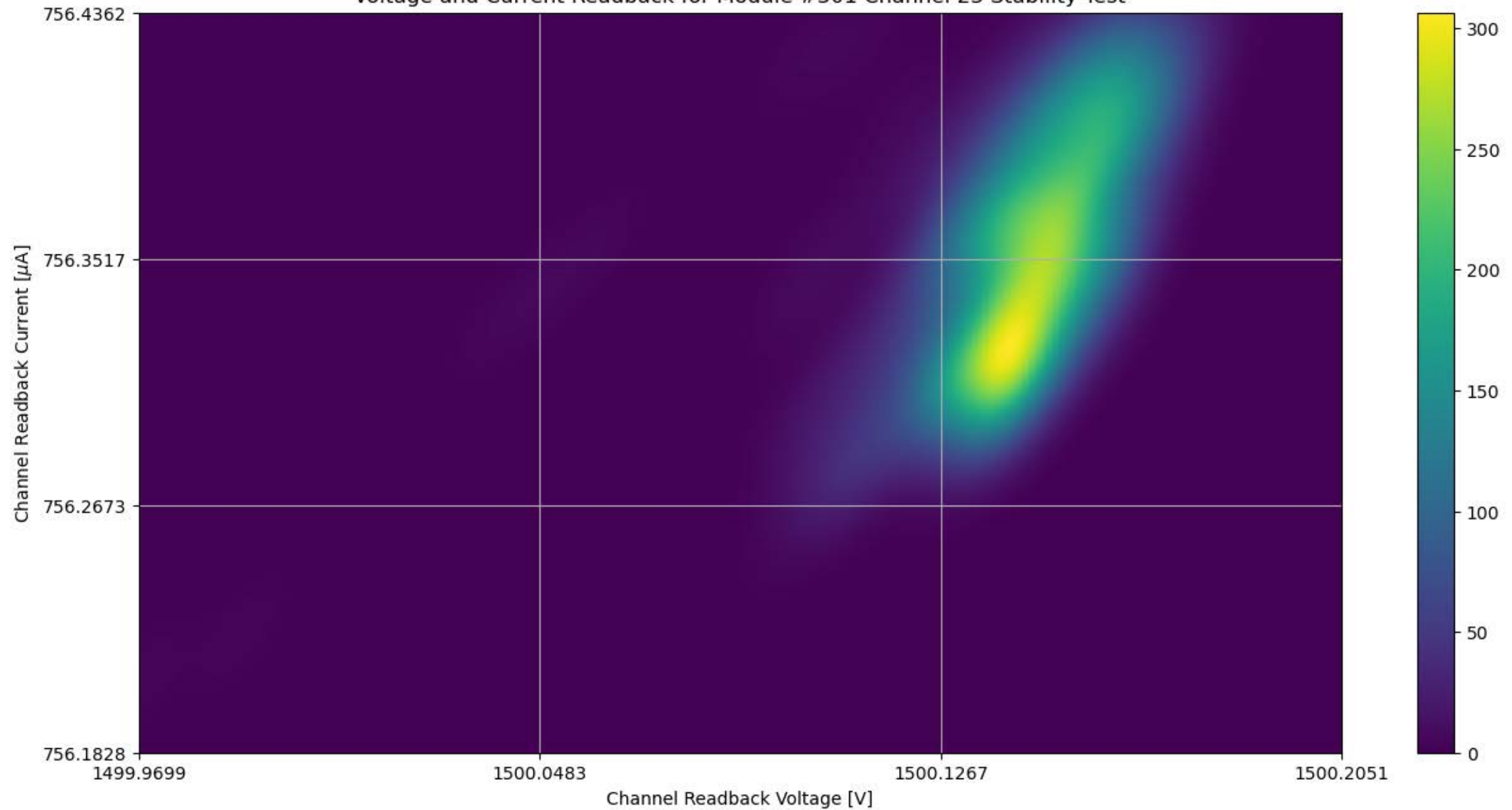
Voltage and Current Readback for Module #301 Channel 23 Stability Test
