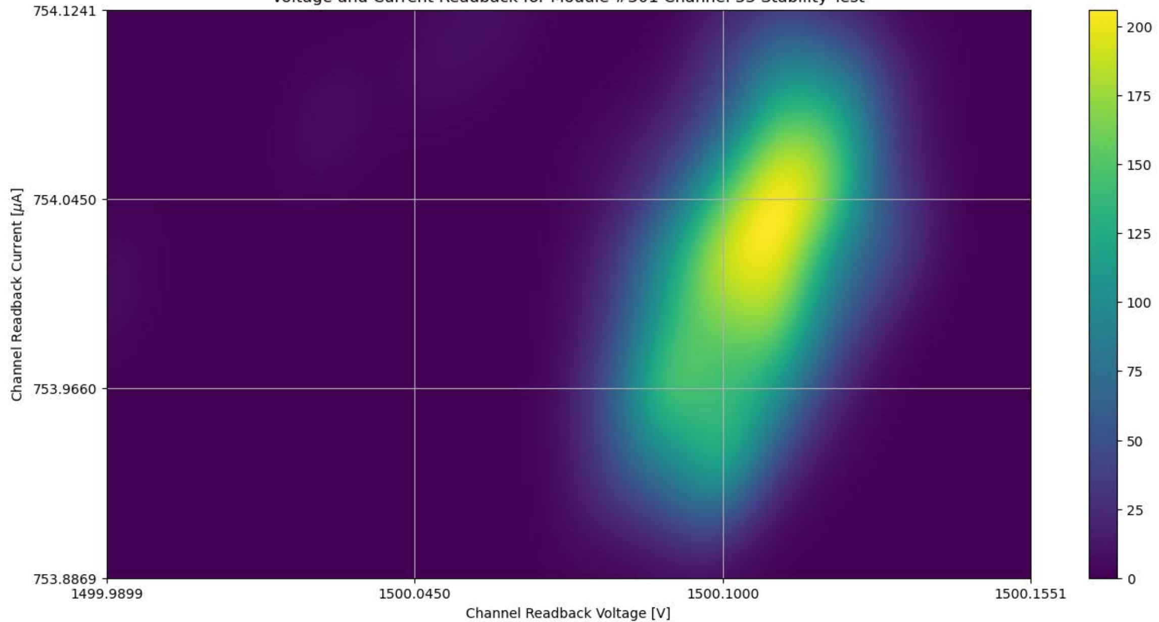
Voltage and Current Readback for Module #301 Channel 33 Stability Test
