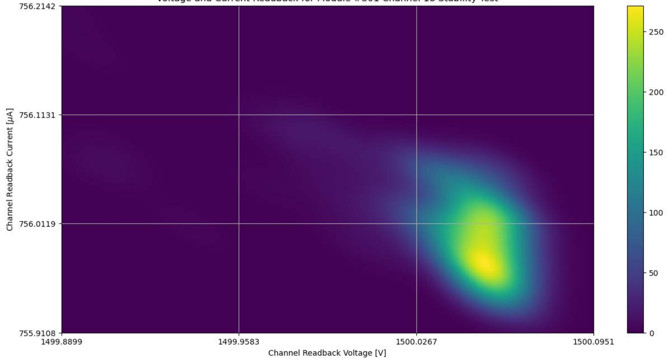
Voltage and Current Readback for Module #301 Channel 18 Stability Test
