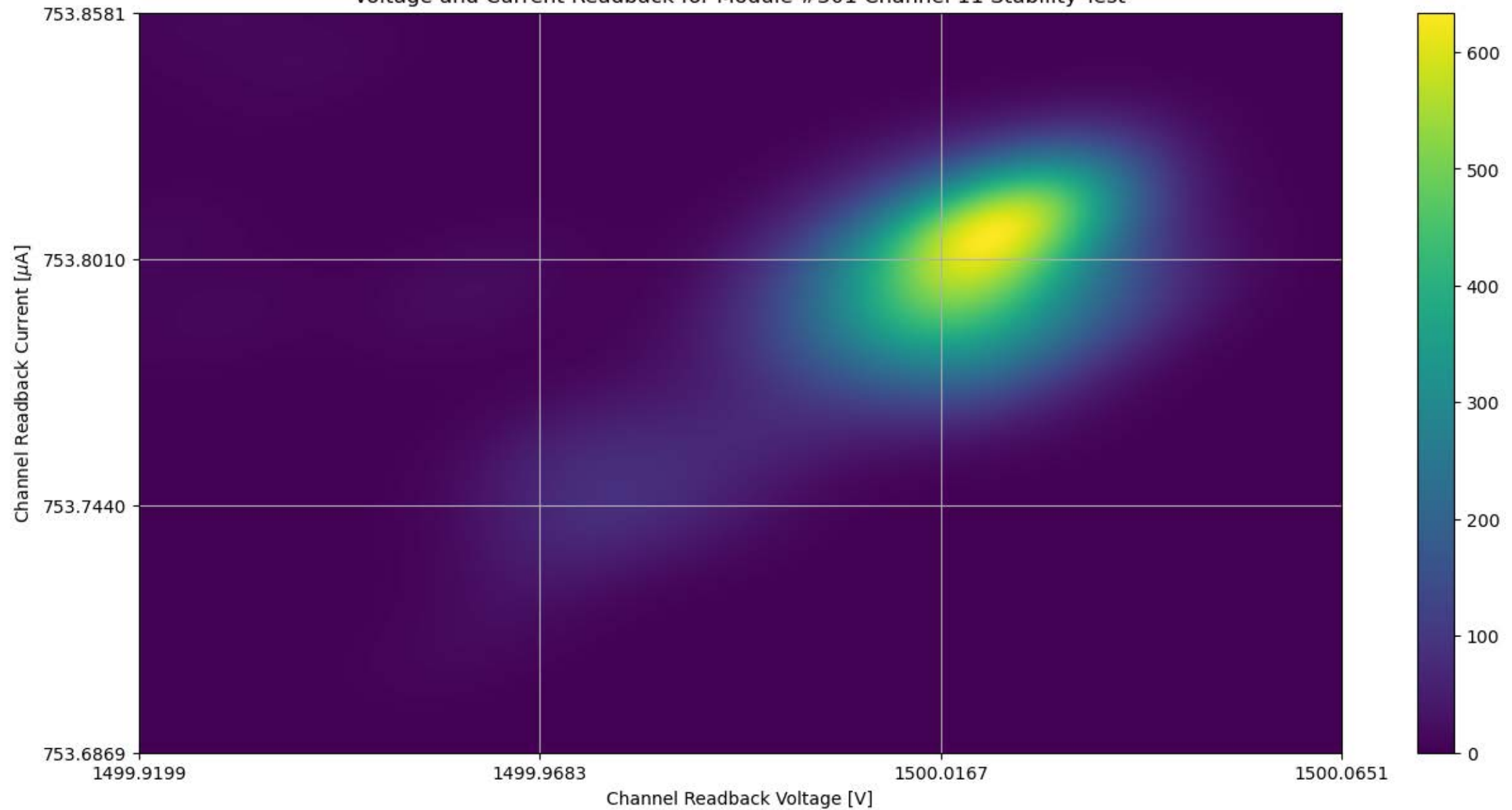
Voltage and Current Readback for Module #301 Channel 11 Stability Test
