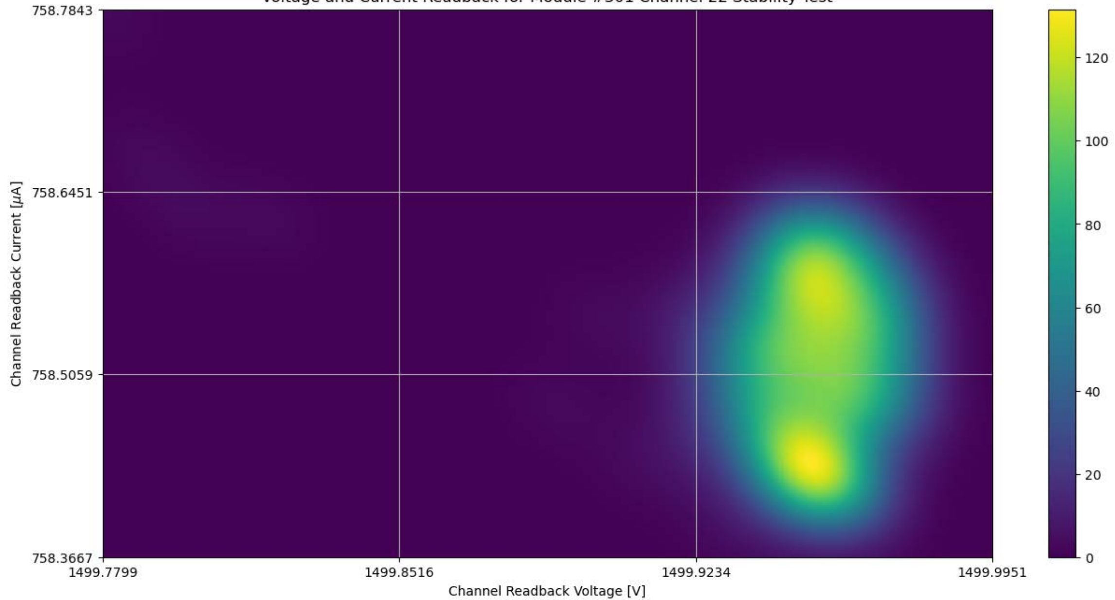
Voltage and Current Readback for Module #301 Channel 22 Stability Test
