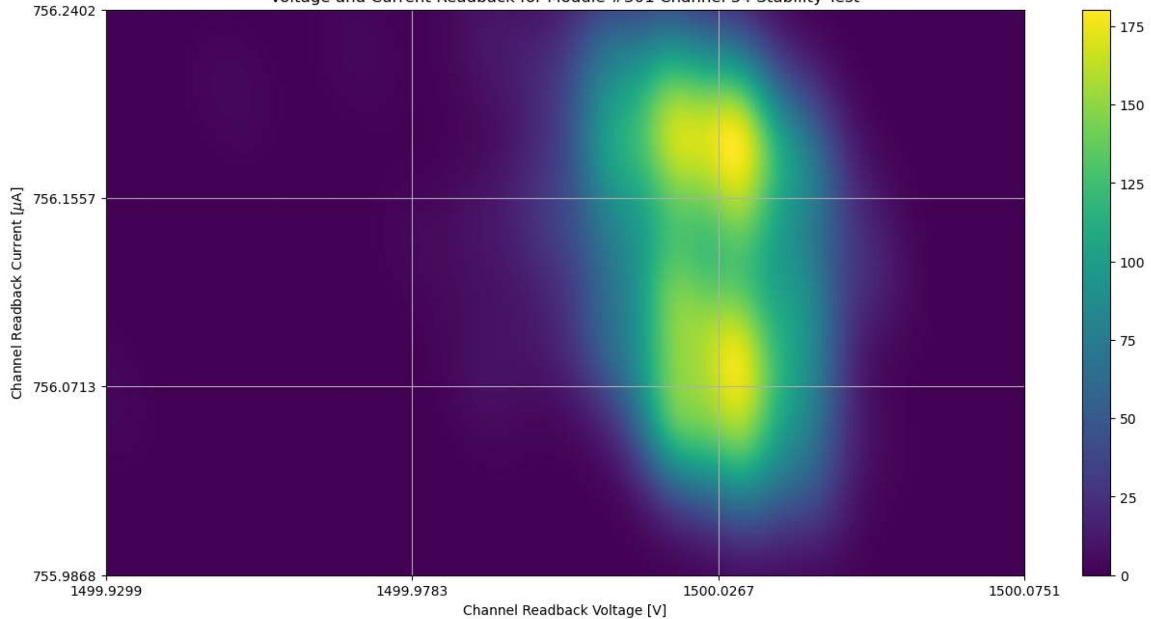
Voltage and Current Readback for Module #301 Channel 34 Stability Test
