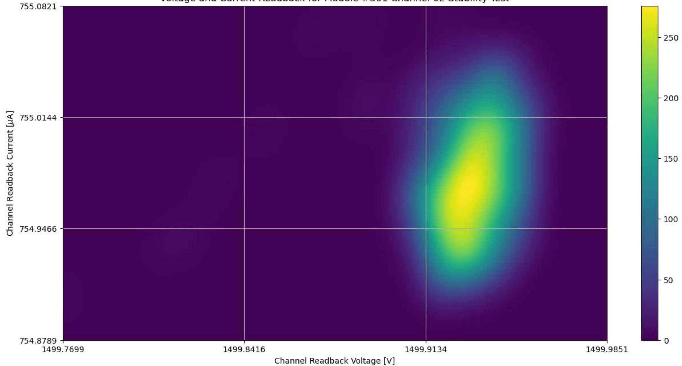
Voltage and Current Readback for Module #301 Channel 02 Stability Test
