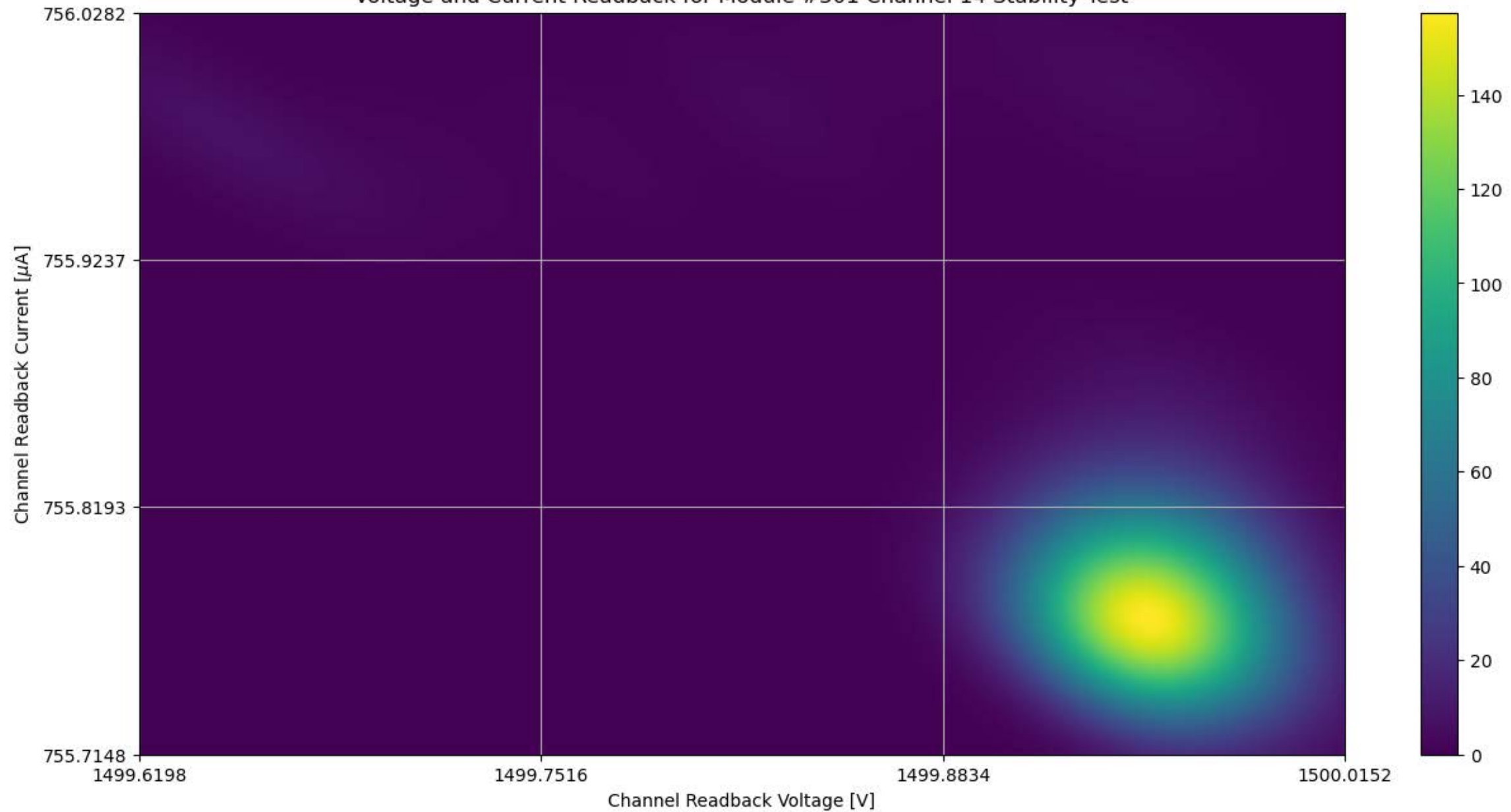
Voltage and Current Readback for Module #301 Channel 14 Stability Test
