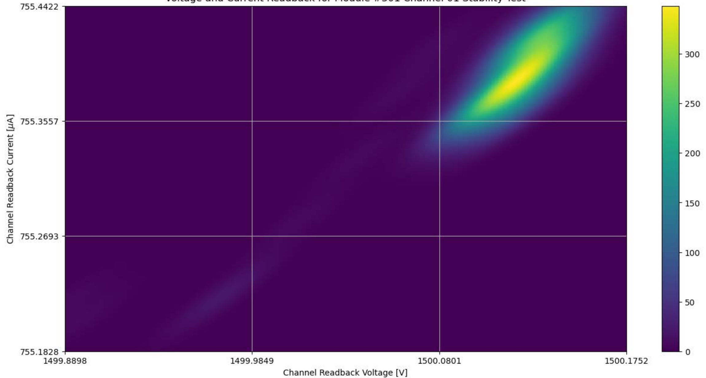
Voltage and Current Readback for Module #301 Channel 01 Stability Test
