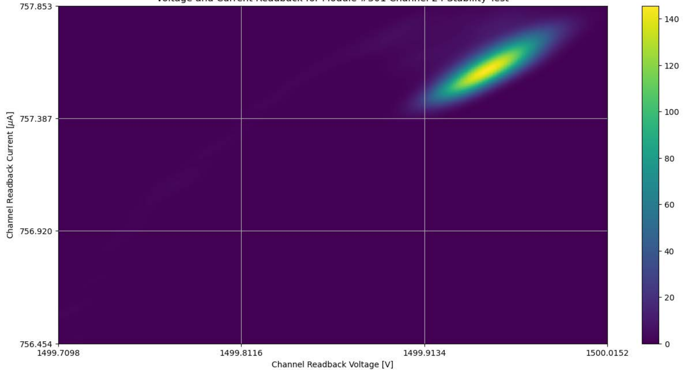
Voltage and Current Readback for Module #301 Channel 24 Stability Test
