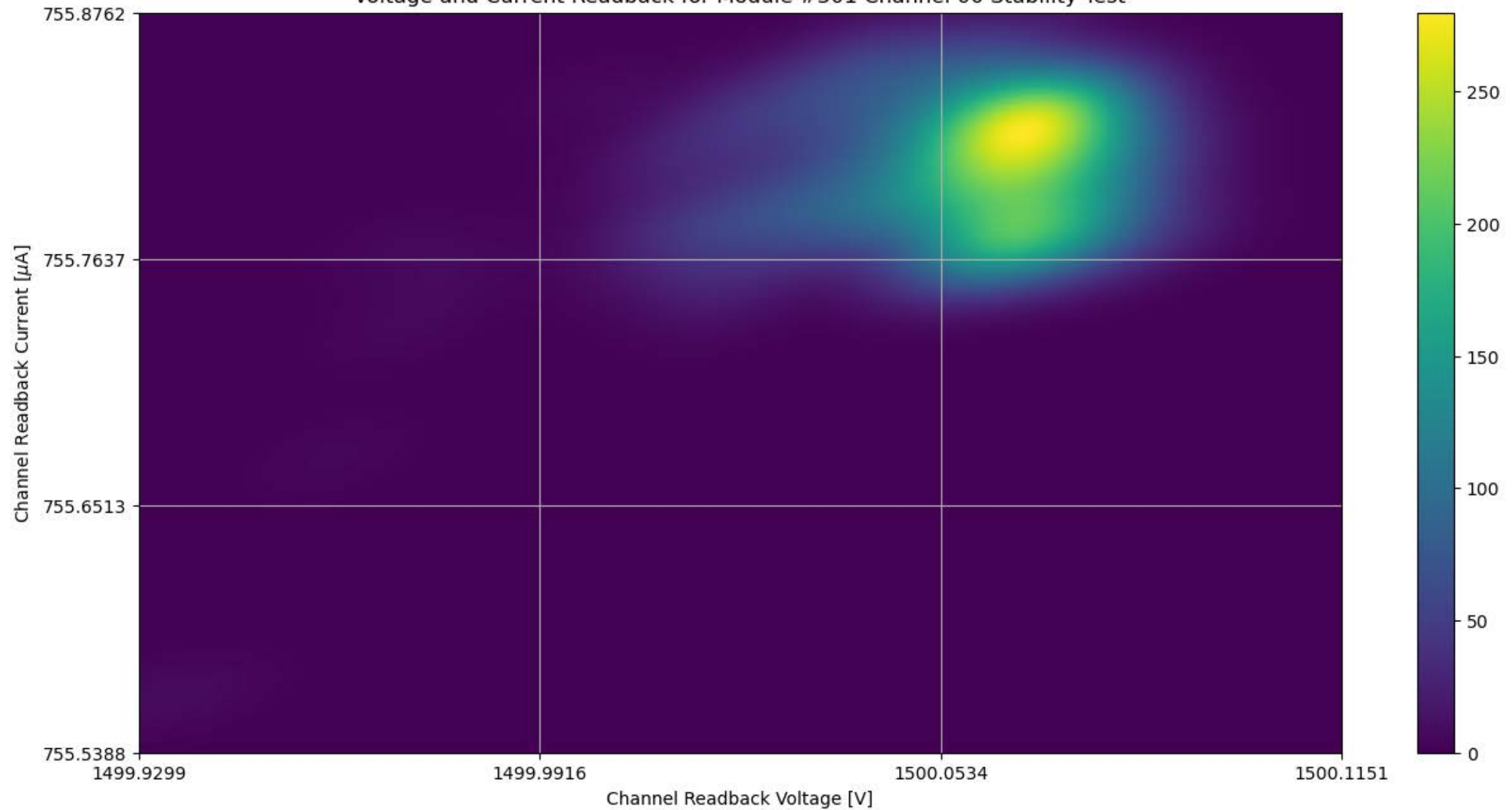
Voltage and Current Readback for Module #301 Channel 00 Stability Test
