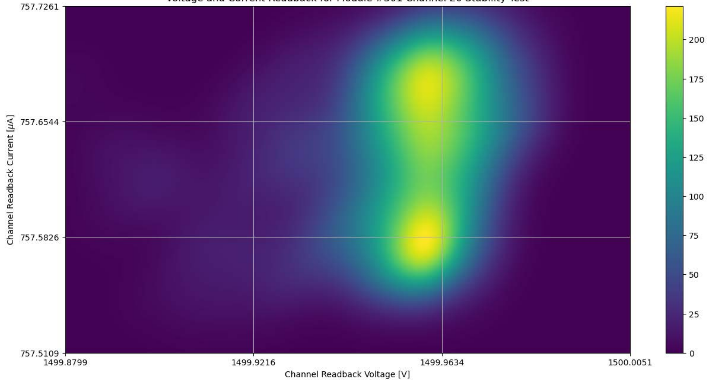
Voltage and Current Readback for Module #301 Channel 20 Stability Test
