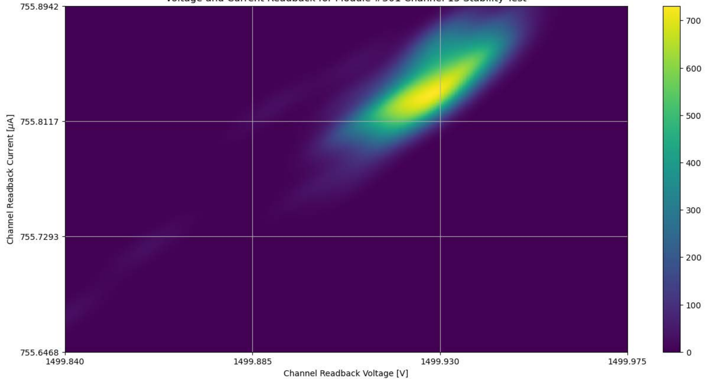
Voltage and Current Readback for Module #301 Channel 15 Stability Test
