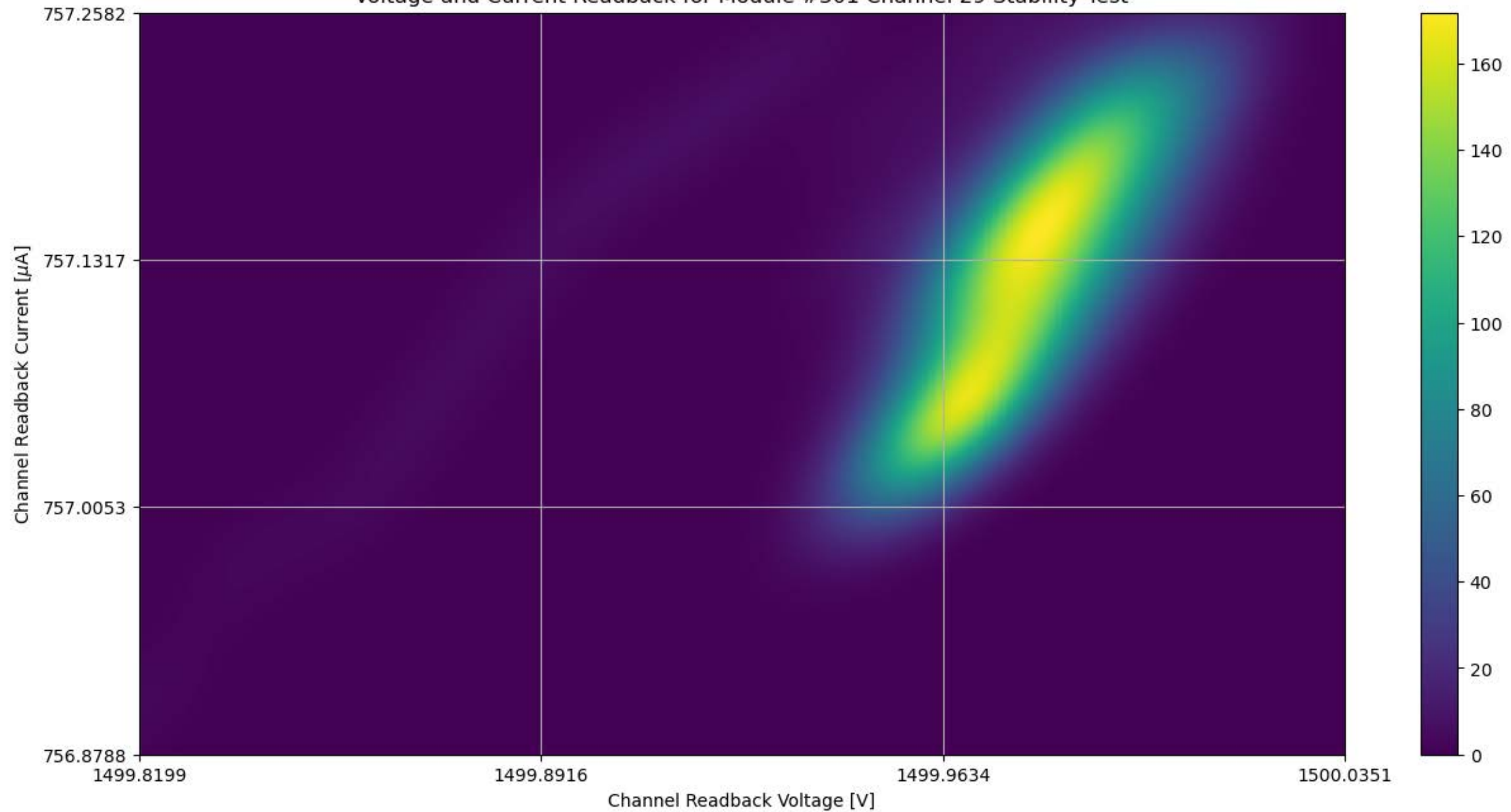
Voltage and Current Readback for Module #301 Channel 29 Stability Test
