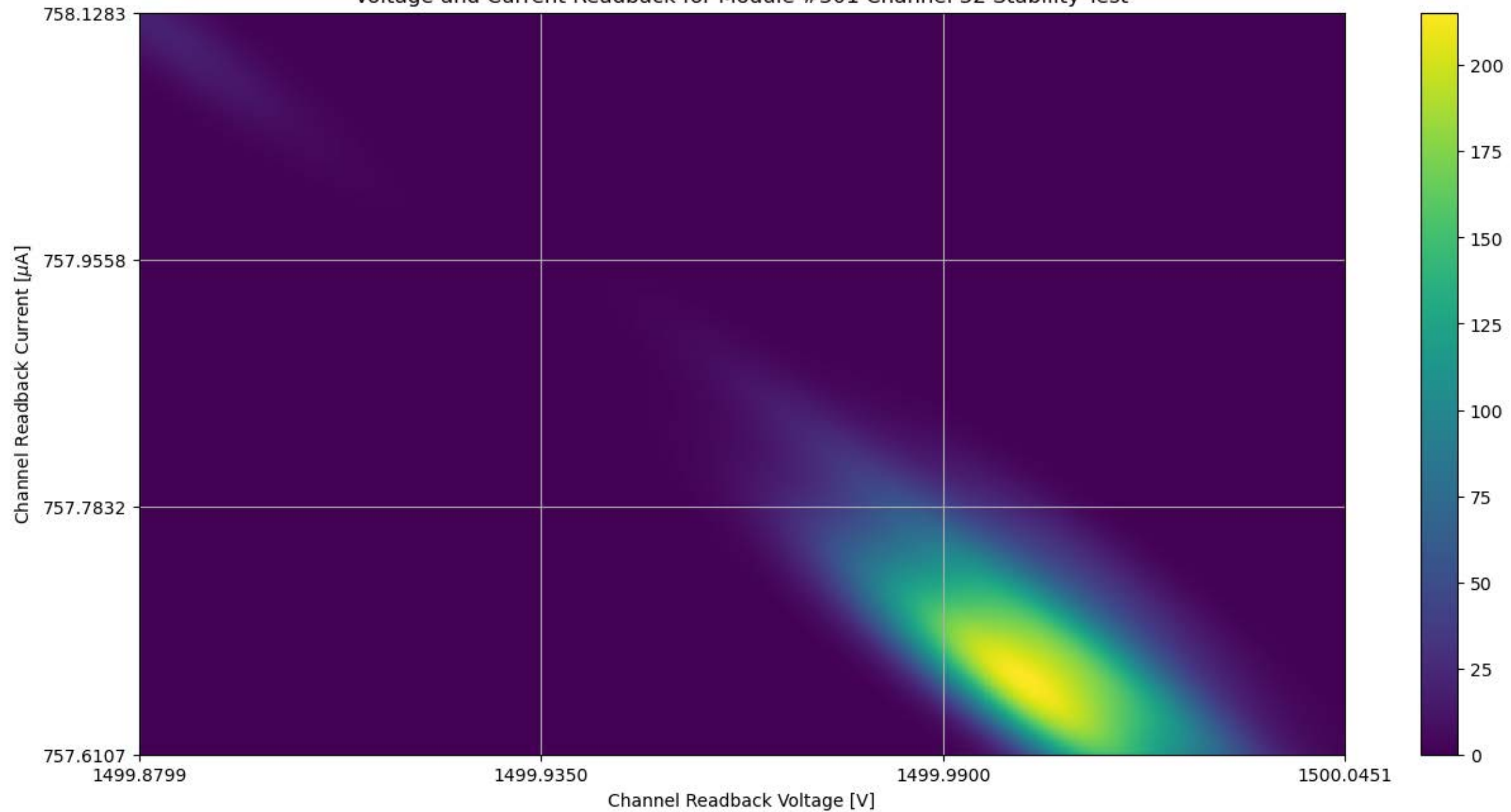
Voltage and Current Readback for Module #301 Channel 32 Stability Test
