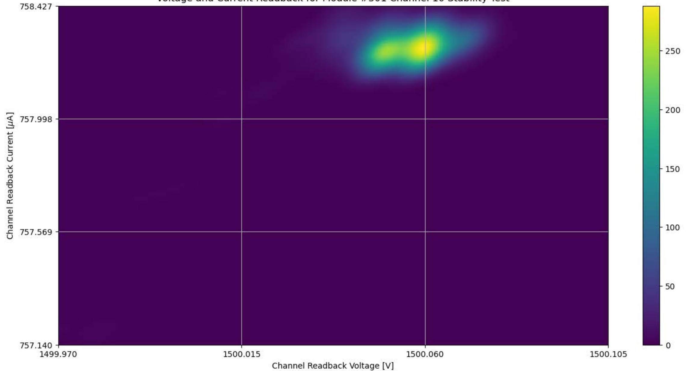
Voltage and Current Readback for Module #301 Channel 10 Stability Test
