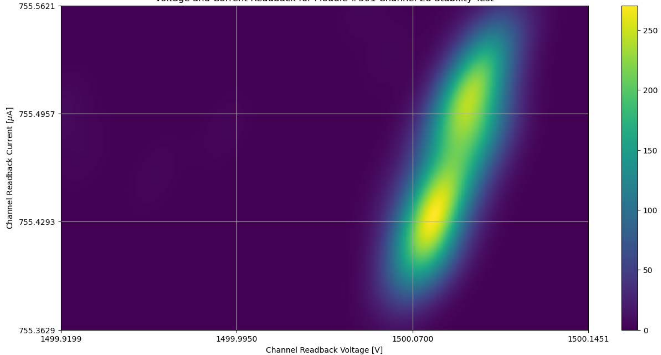
Voltage and Current Readback for Module #301 Channel 28 Stability Test
