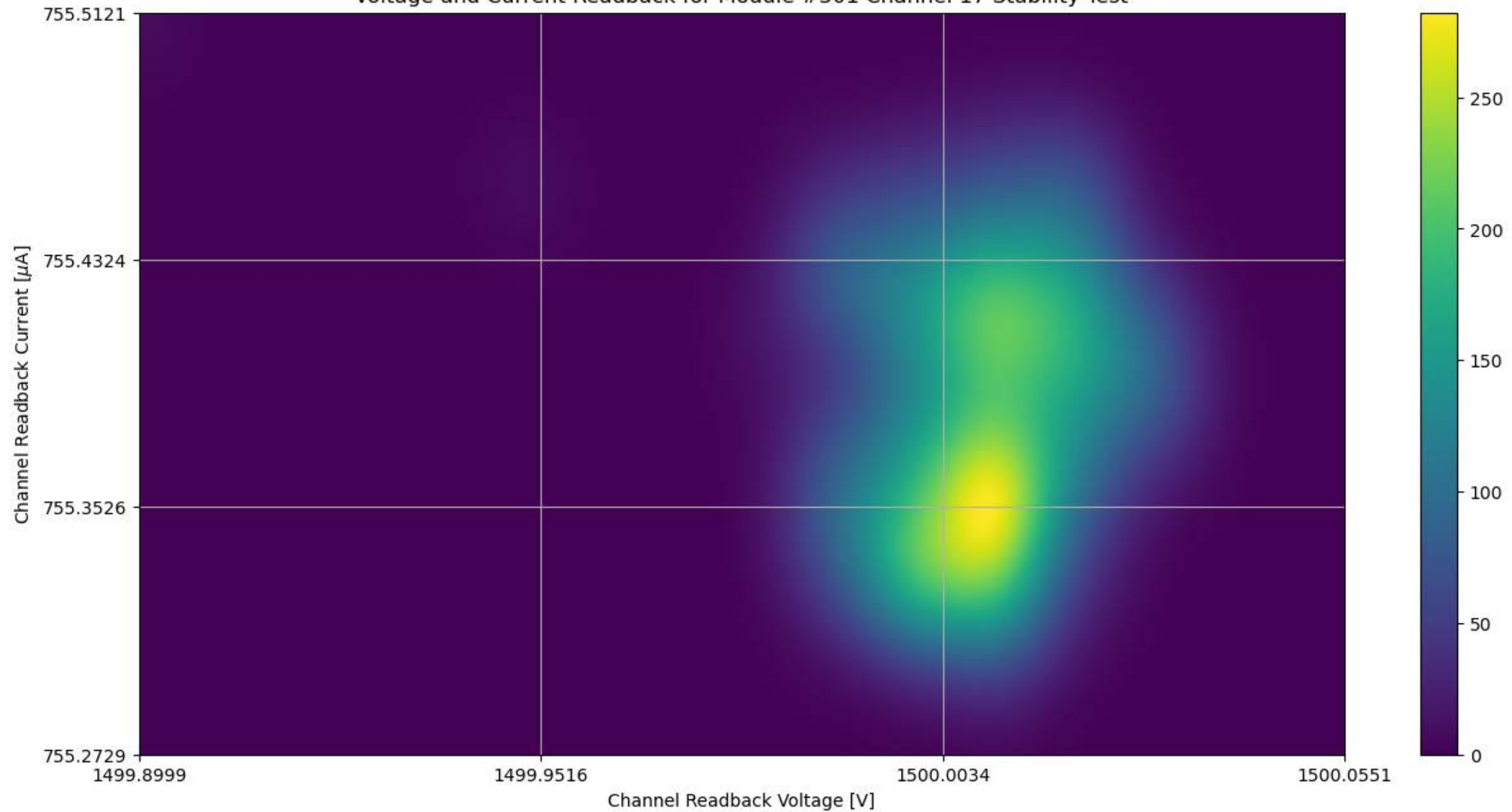
Voltage and Current Readback for Module #301 Channel 17 Stability Test
