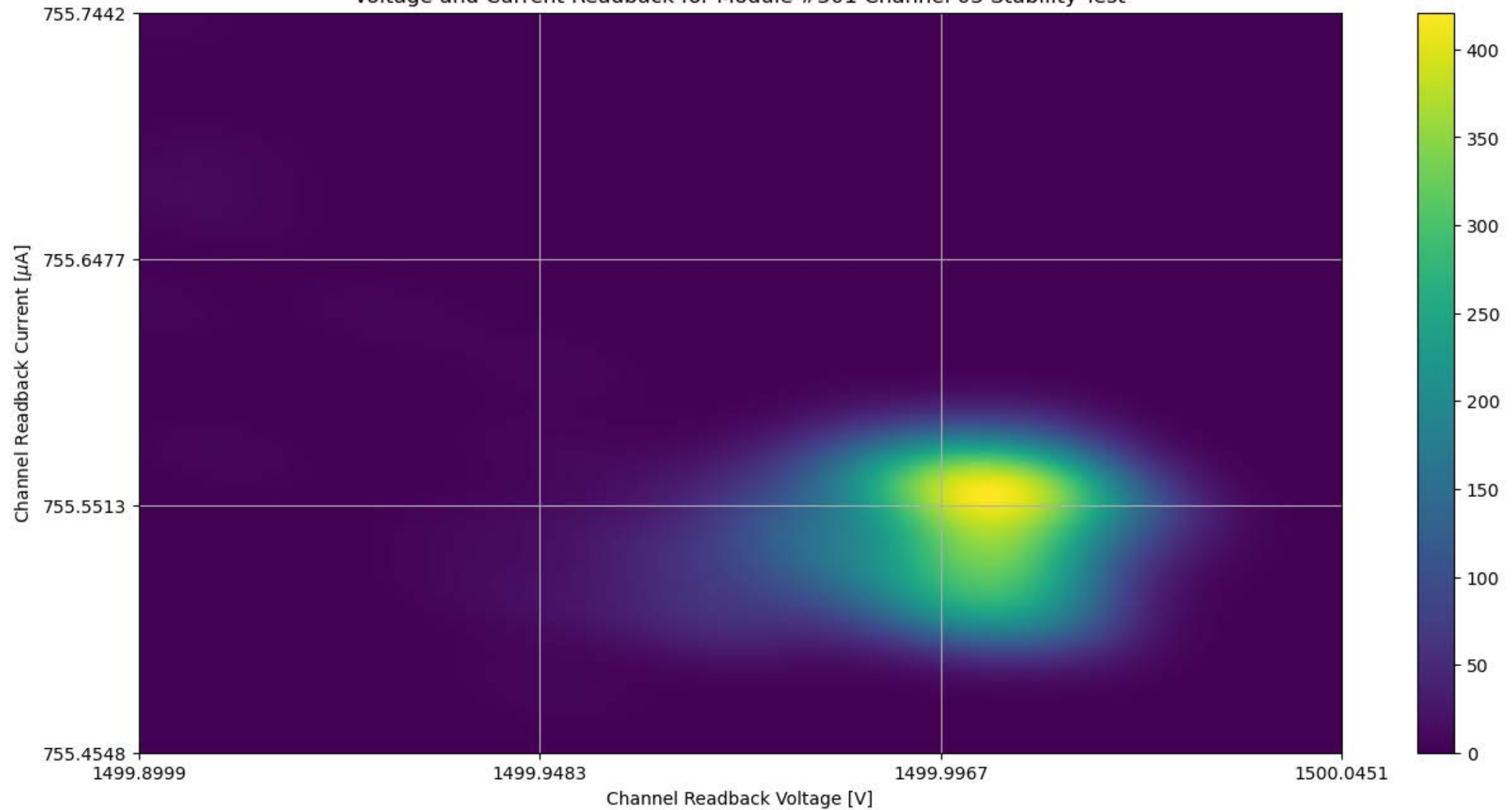
Voltage and Current Readback for Module #301 Channel 03 Stability Test
