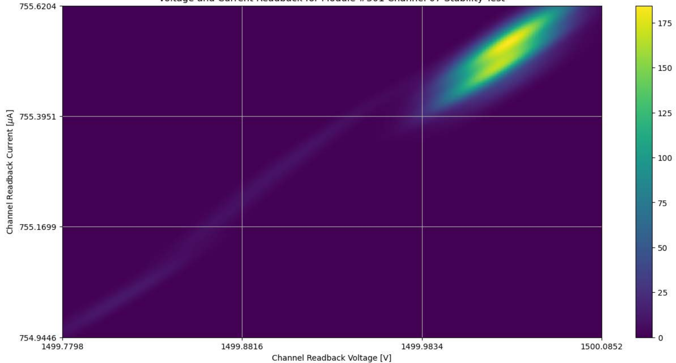
Voltage and Current Readback for Module #301 Channel 07 Stability Test
