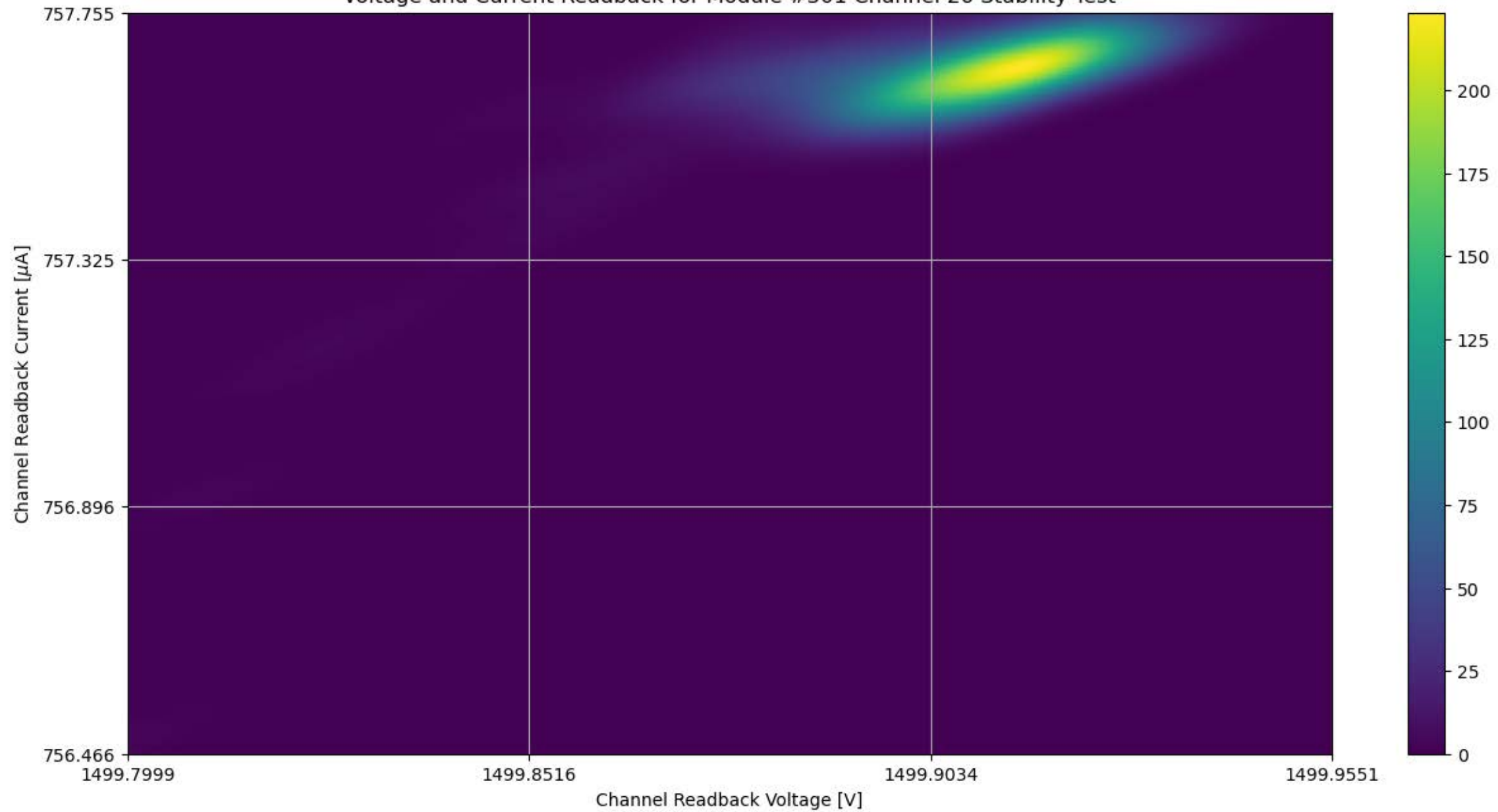
Voltage and Current Readback for Module #301 Channel 26 Stability Test
