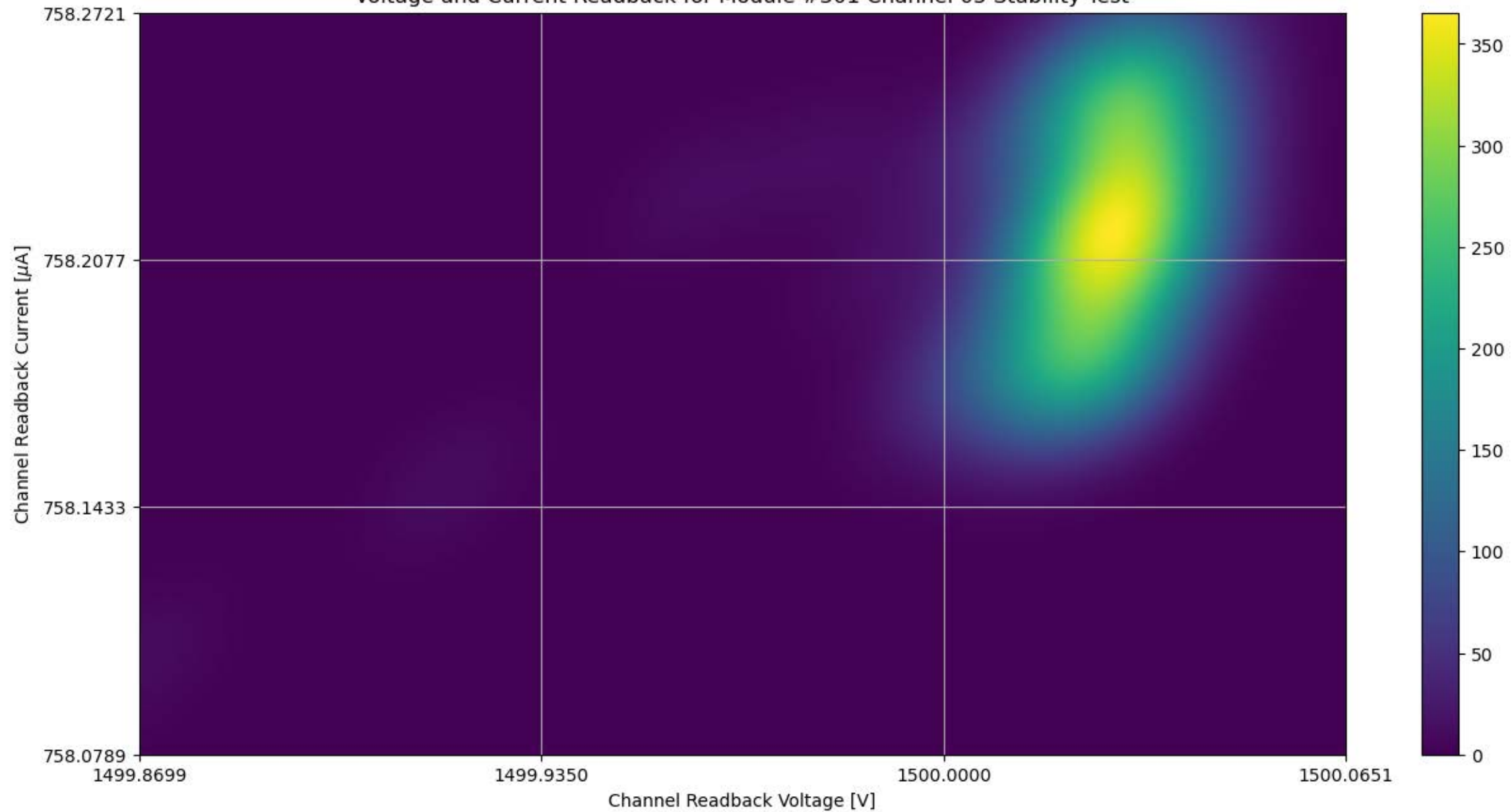
Voltage and Current Readback for Module #301 Channel 05 Stability Test
