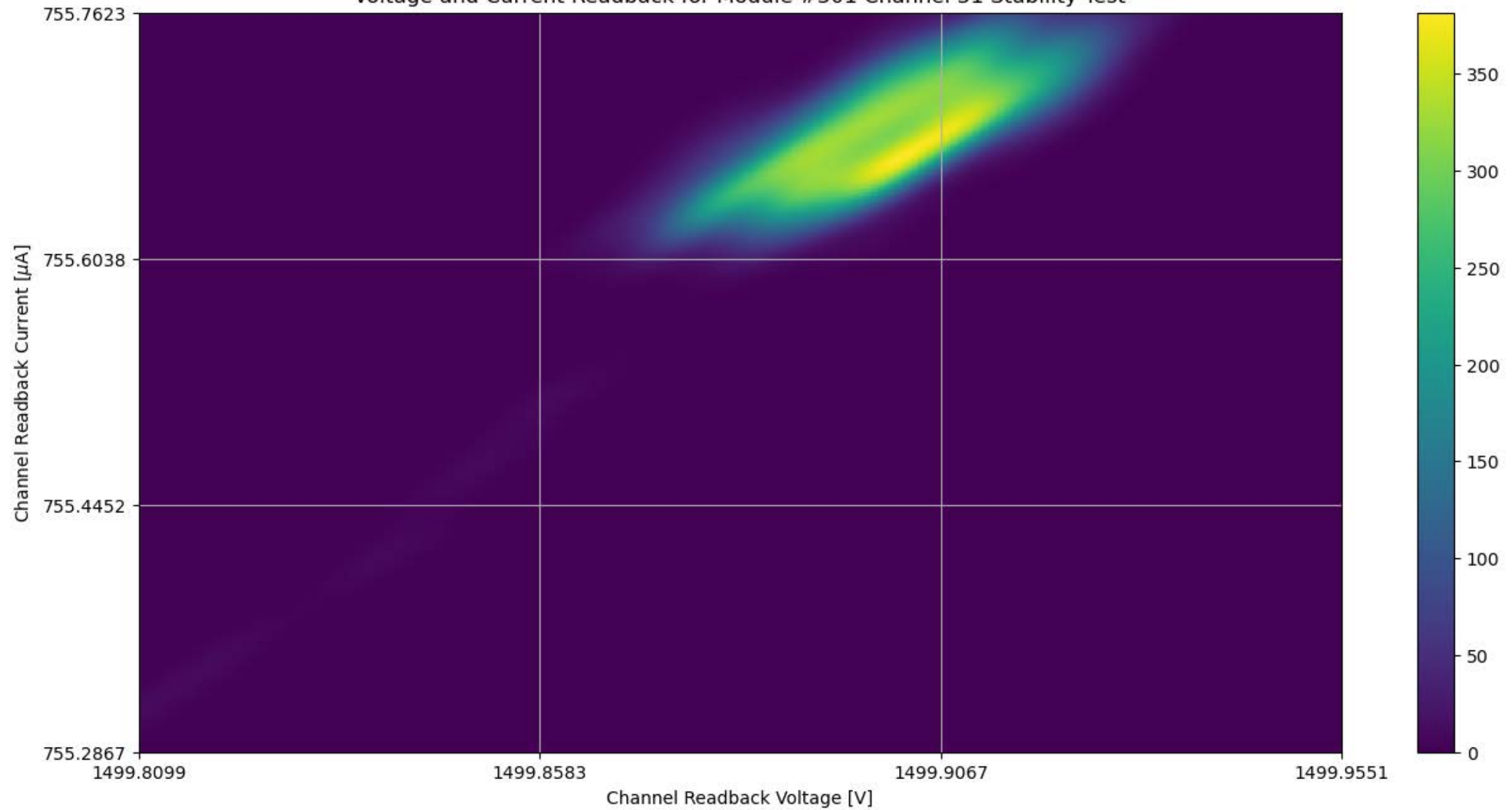
Voltage and Current Readback for Module #301 Channel 31 Stability Test
