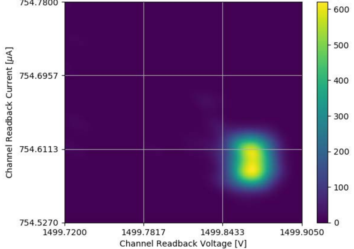
Voltage and Current Readback for Module #302 Channel 13 Stability Test
