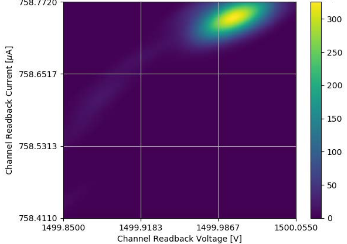
Voltage and Current Readback for Module #302 Channel 25 Stability Test
