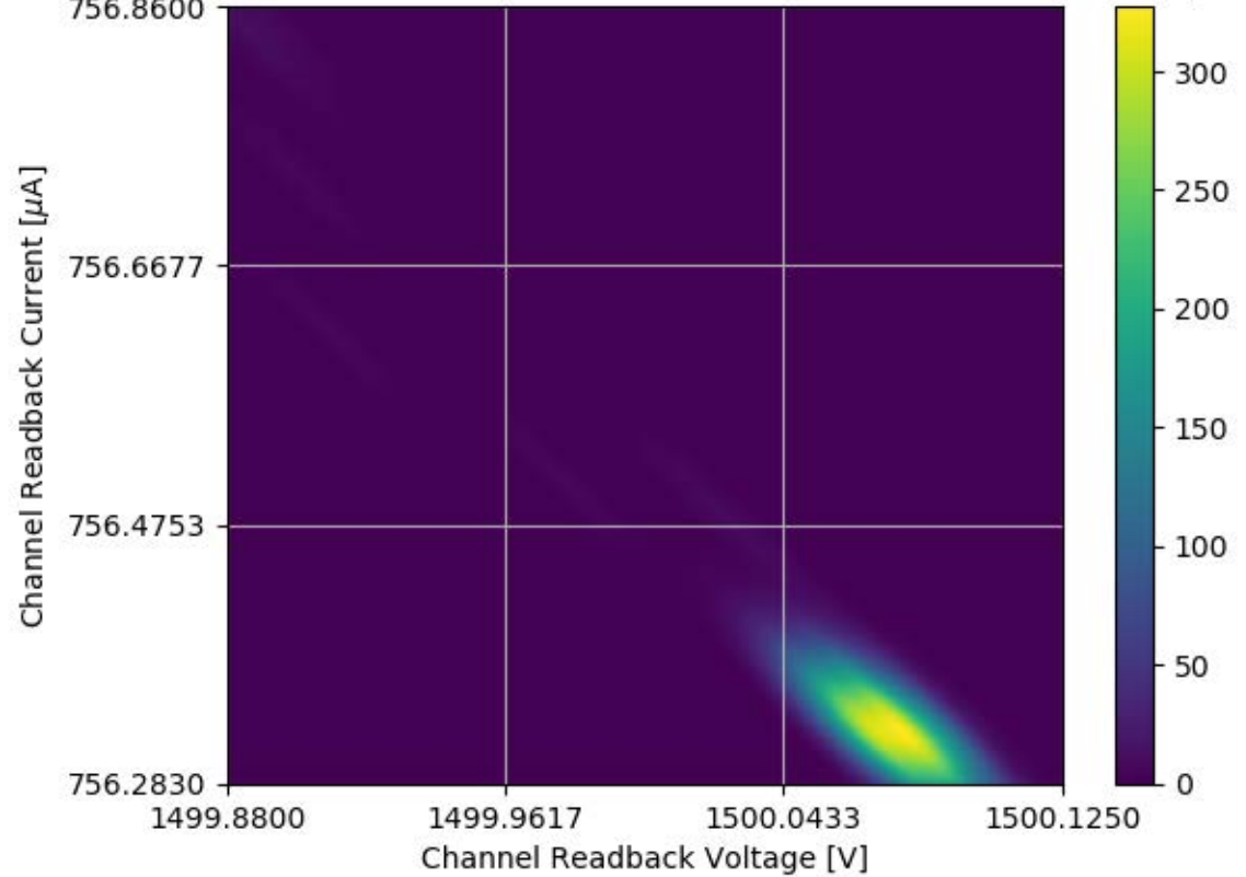
Voltage and Current Readback for Module #302 Channel 02 Stability Test
