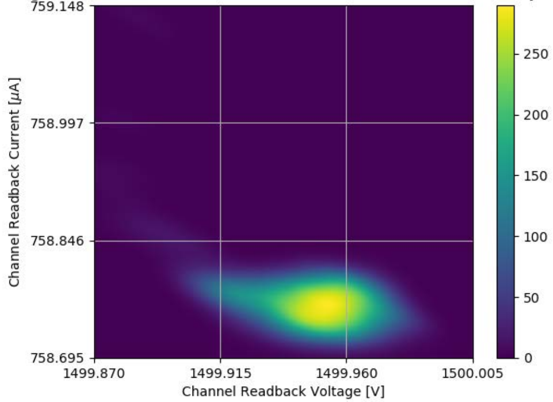
Voltage and Current Readback for Module #302 Channel 05 Stability Test
