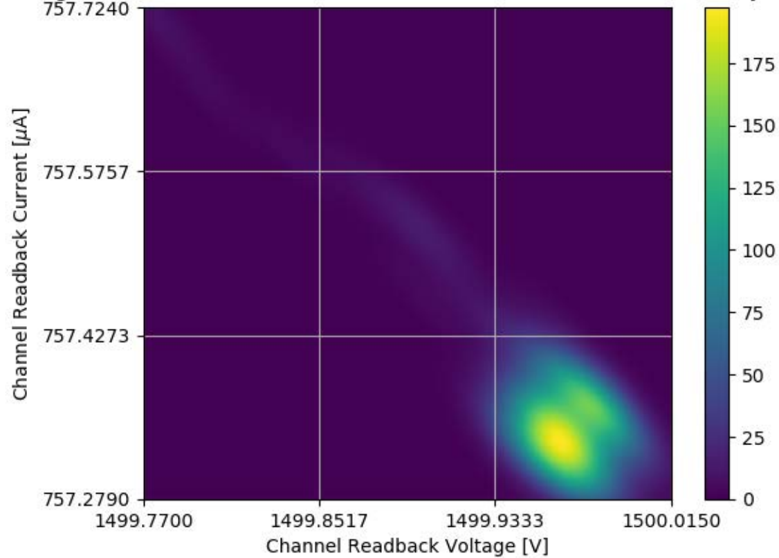
Voltage and Current Readback for Module #302 Channel 35 Stability Test
