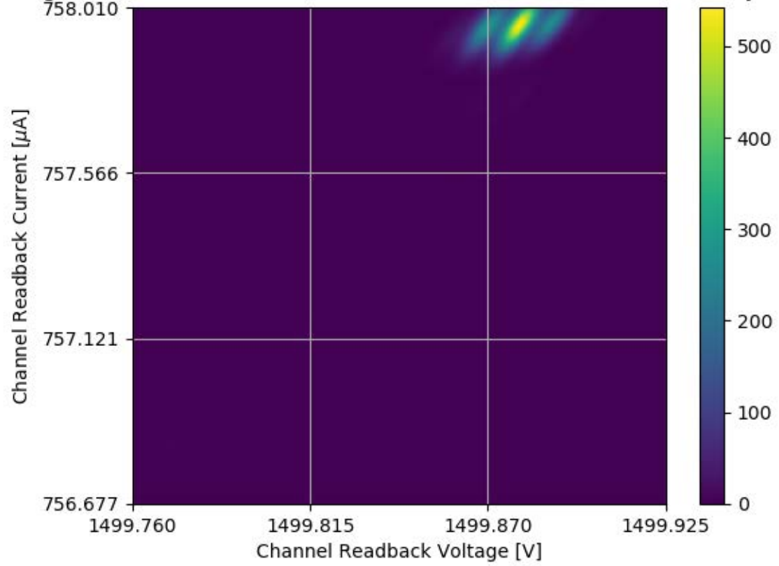
Voltage and Current Readback for Module #302 Channel 19 Stability Test
