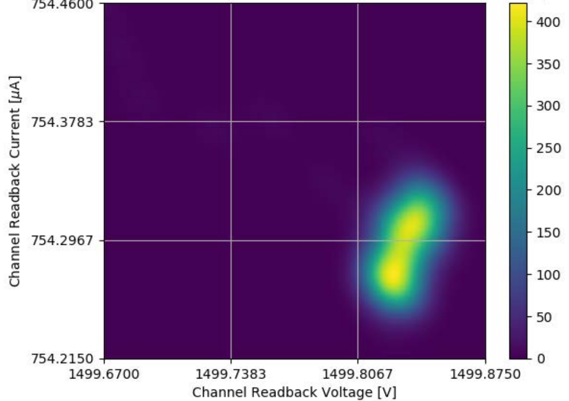
Voltage and Current Readback for Module #302 Channel 33 Stability Test
