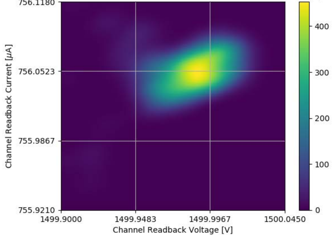
Voltage and Current Readback for Module #302 Channel 03 Stability Test
