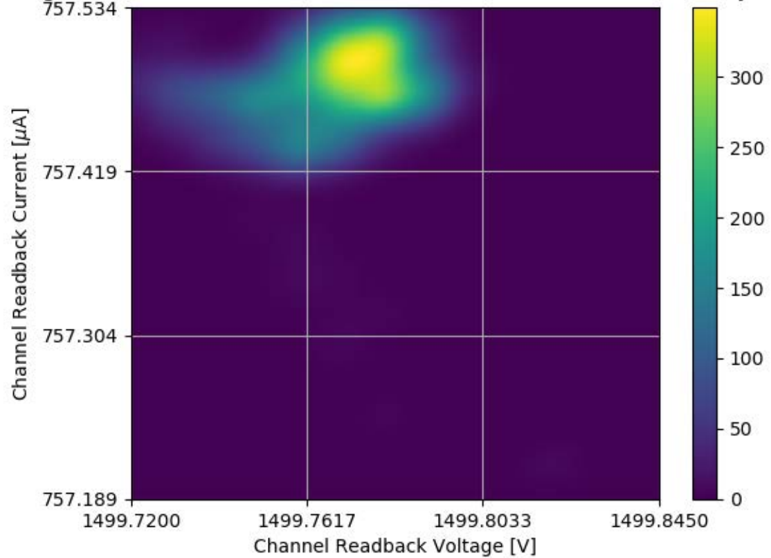
Voltage and Current Readback for Module #302 Channel 21 Stability Test
