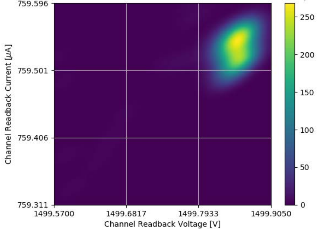
Voltage and Current Readback for Module #302 Channel 22 Stability Test
