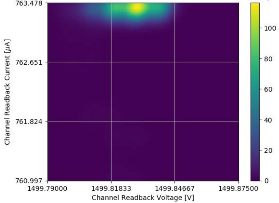
Voltage and Current Readback for Module #302 Channel 09 Stability Test
