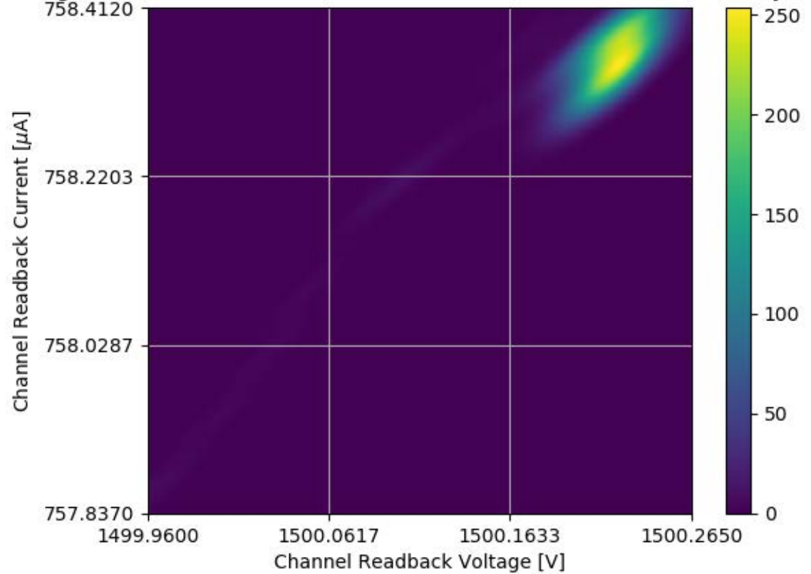
Voltage and Current Readback for Module #302 Channel 32 Stability Test
