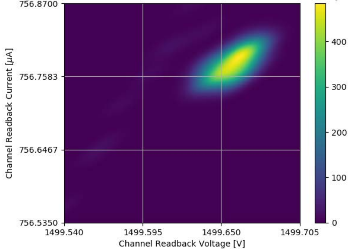
Voltage and Current Readback for Module #302 Channel 15 Stability Test
