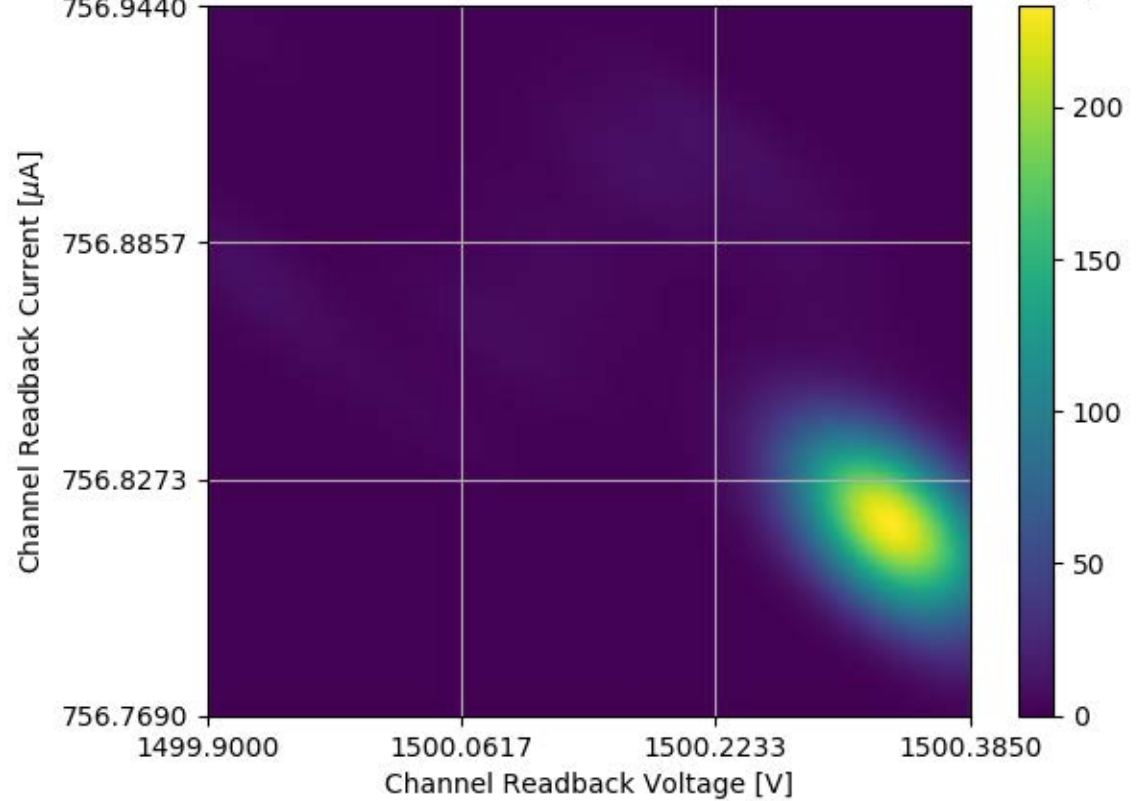
Voltage and Current Readback for Module #302 Channel 31 Stability Test
