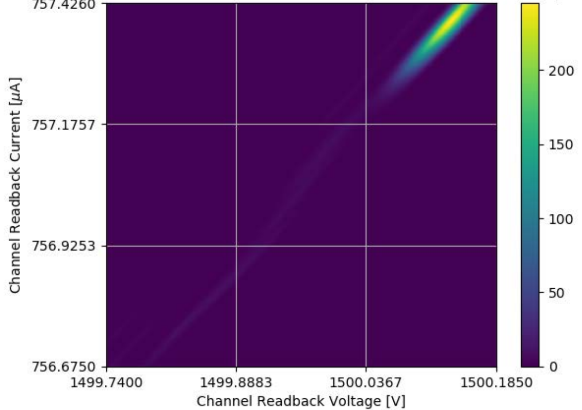
Voltage and Current Readback for Module #302 Channel 34 Stability Test
