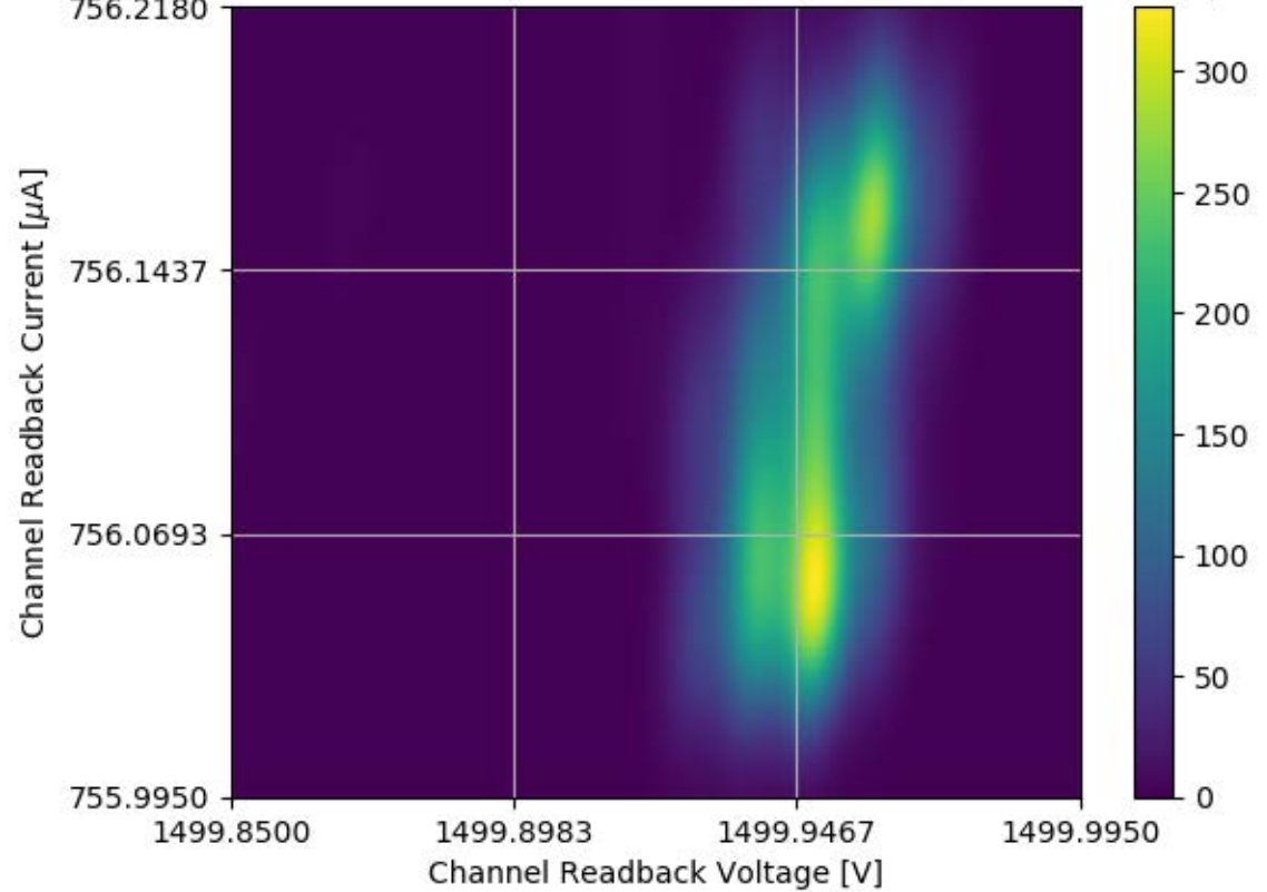
Voltage and Current Readback for Module #302 Channel 28 Stability Test
