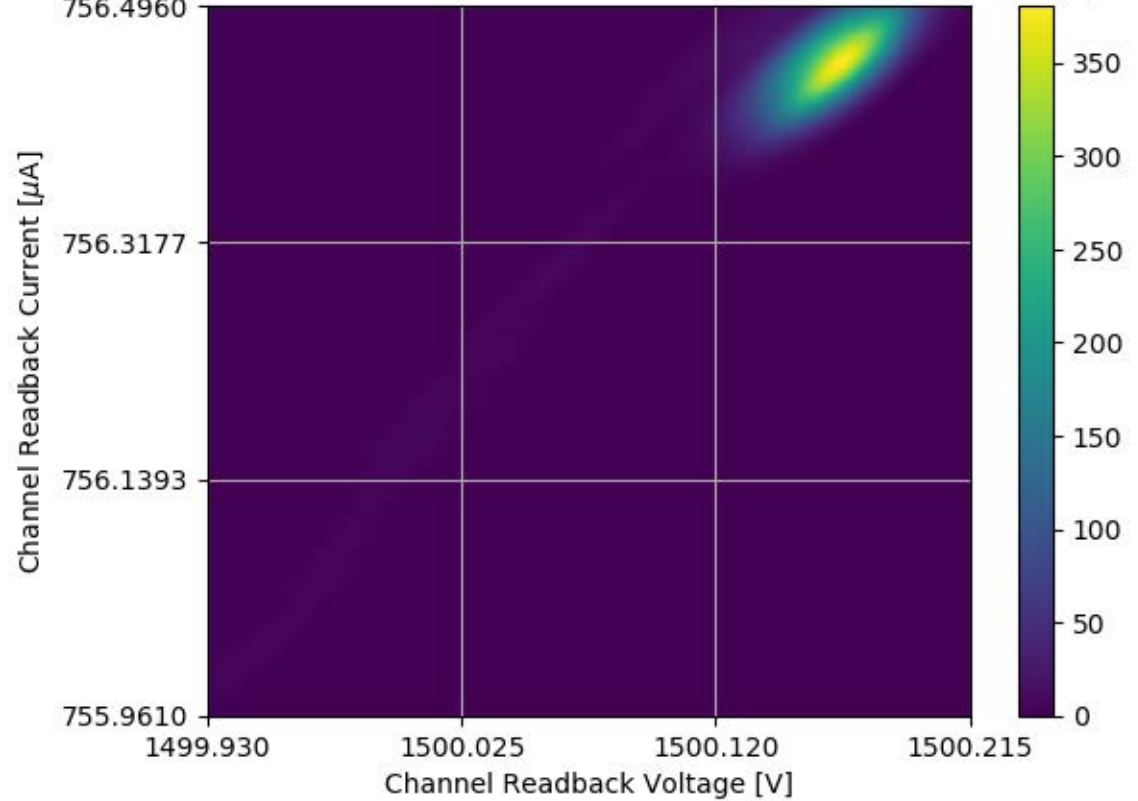
Voltage and Current Readback for Module #302 Channel 17 Stability Test
