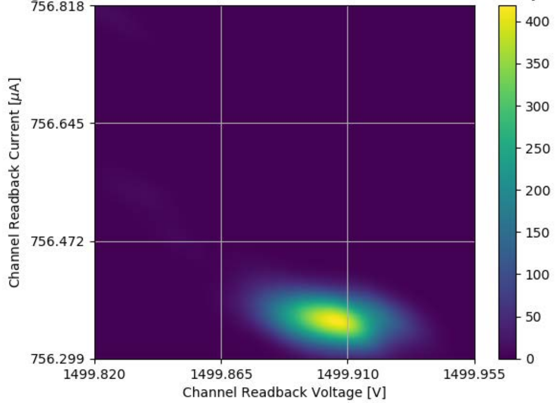
Voltage and Current Readback for Module #302 Channel 18 Stability Test
