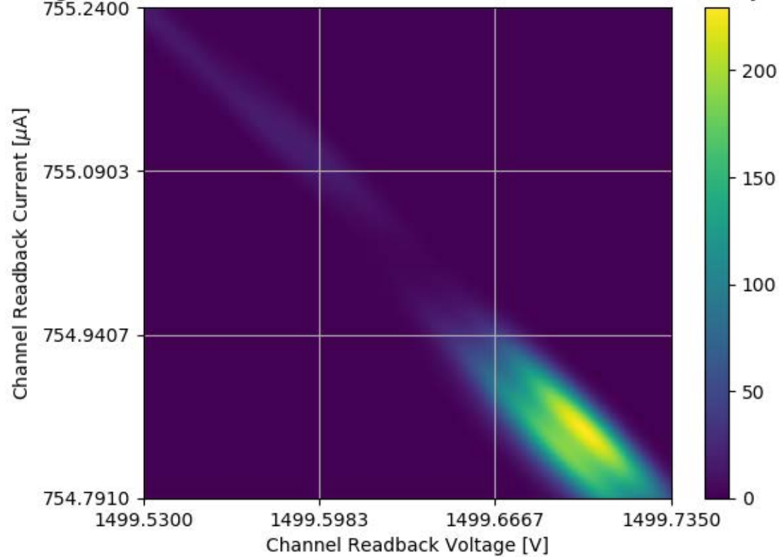
Voltage and Current Readback for Module #302 Channel 30 Stability Test
