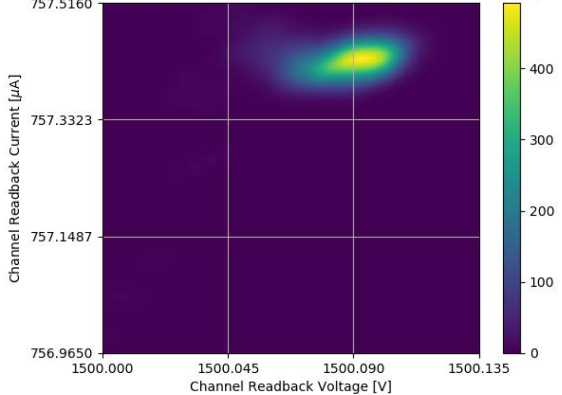
Voltage and Current Readback for Module #302 Channel 29 Stability Test
