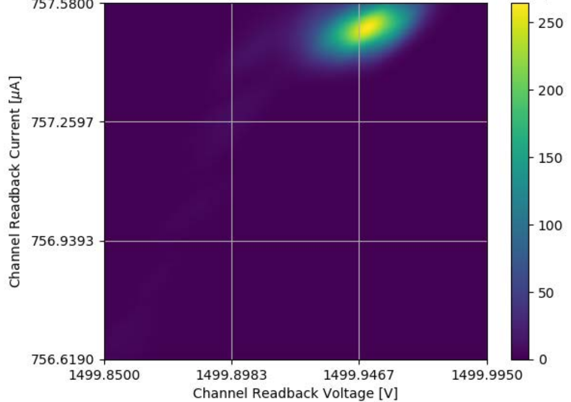
Voltage and Current Readback for Module #302 Channel 26 Stability Test
