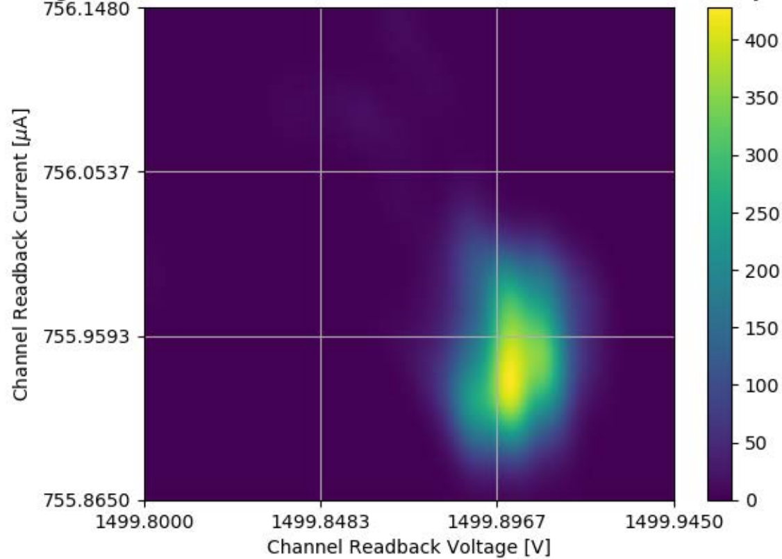
Voltage and Current Readback for Module #304 Channel 14 Stability Test
