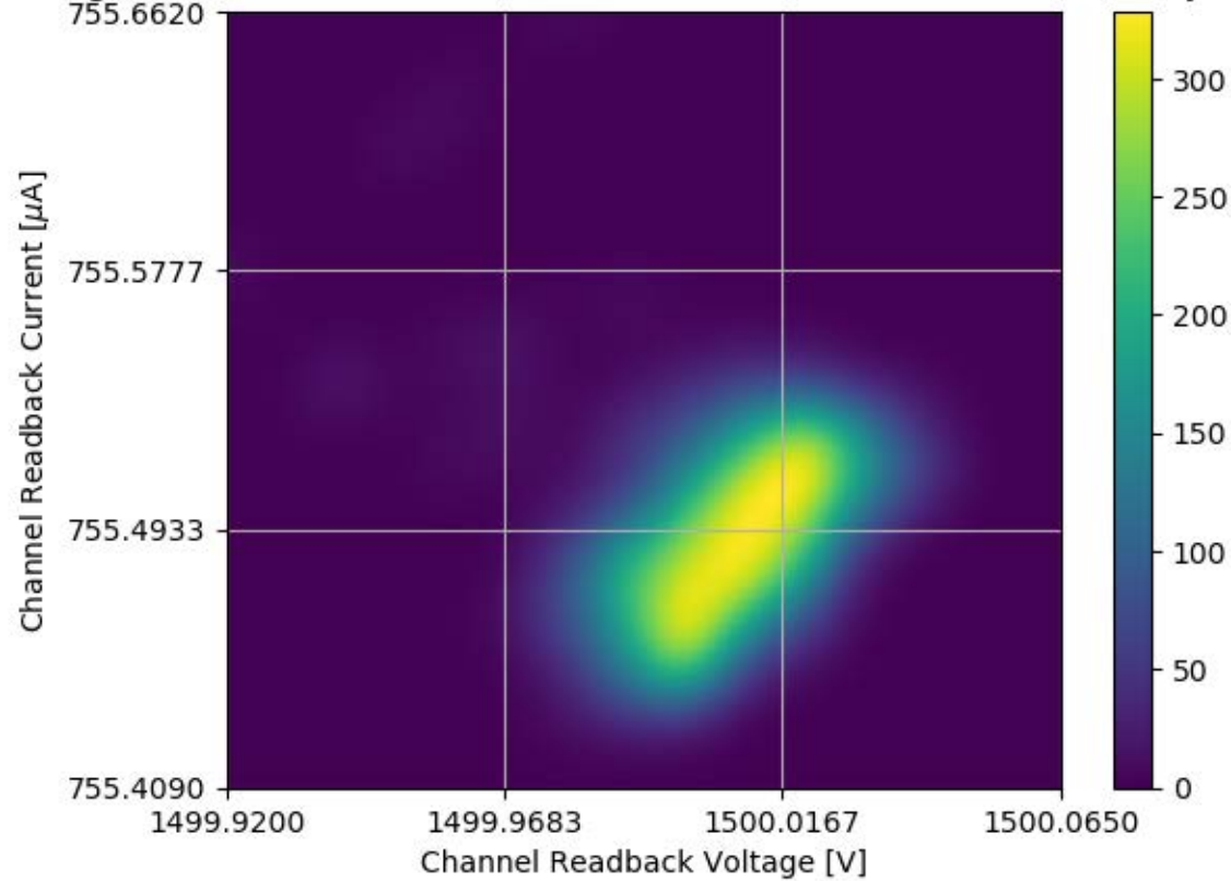
Voltage and Current Readback for Module #304 Channel 15 Stability Test
