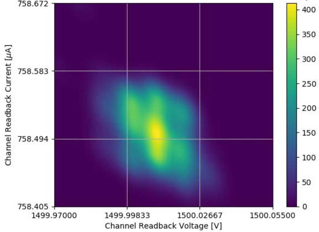
Voltage and Current Readback for Module #304 Channel 35 Stability Test
