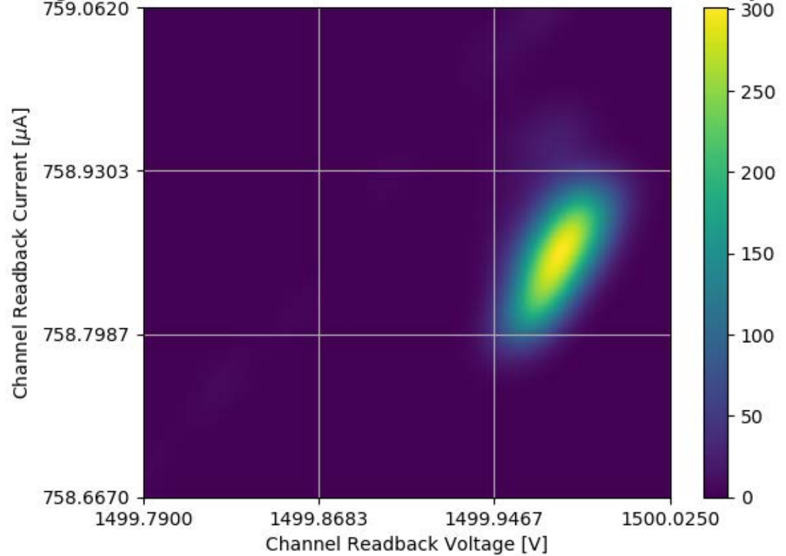
Voltage and Current Readback for Module #304 Channel 12 Stability Test
