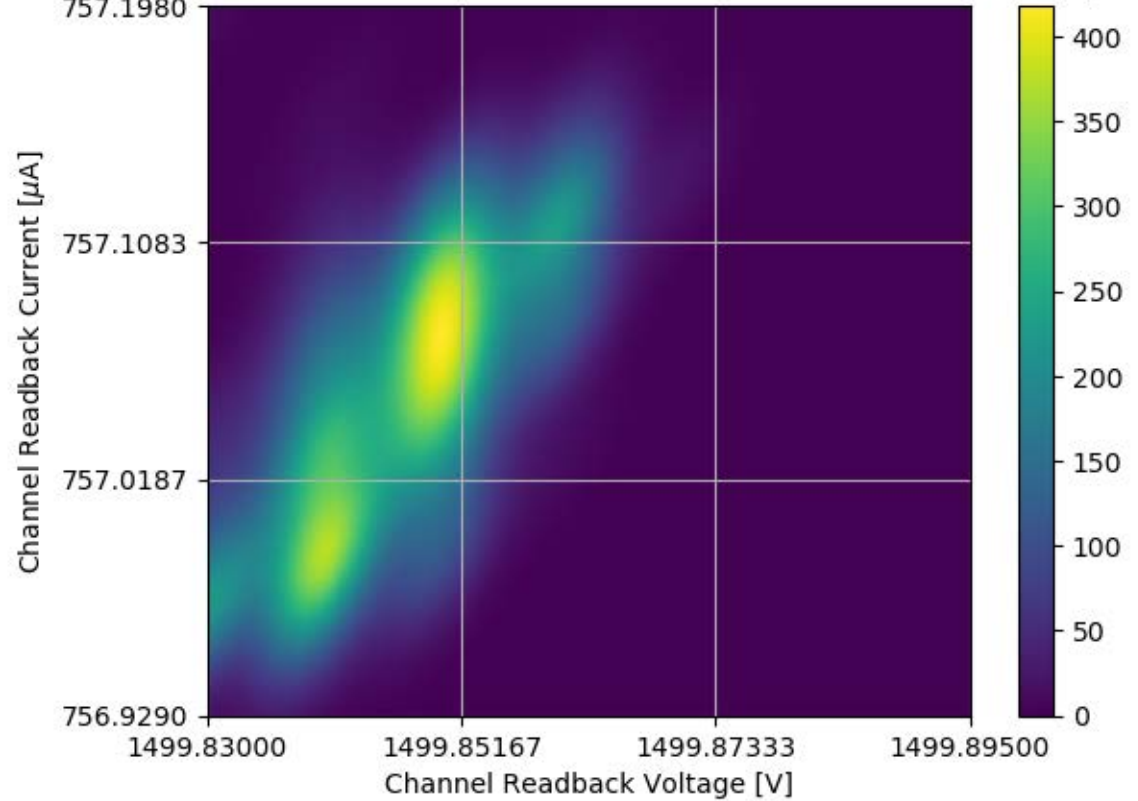
Voltage and Current Readback for Module #304 Channel 23 Stability Test
