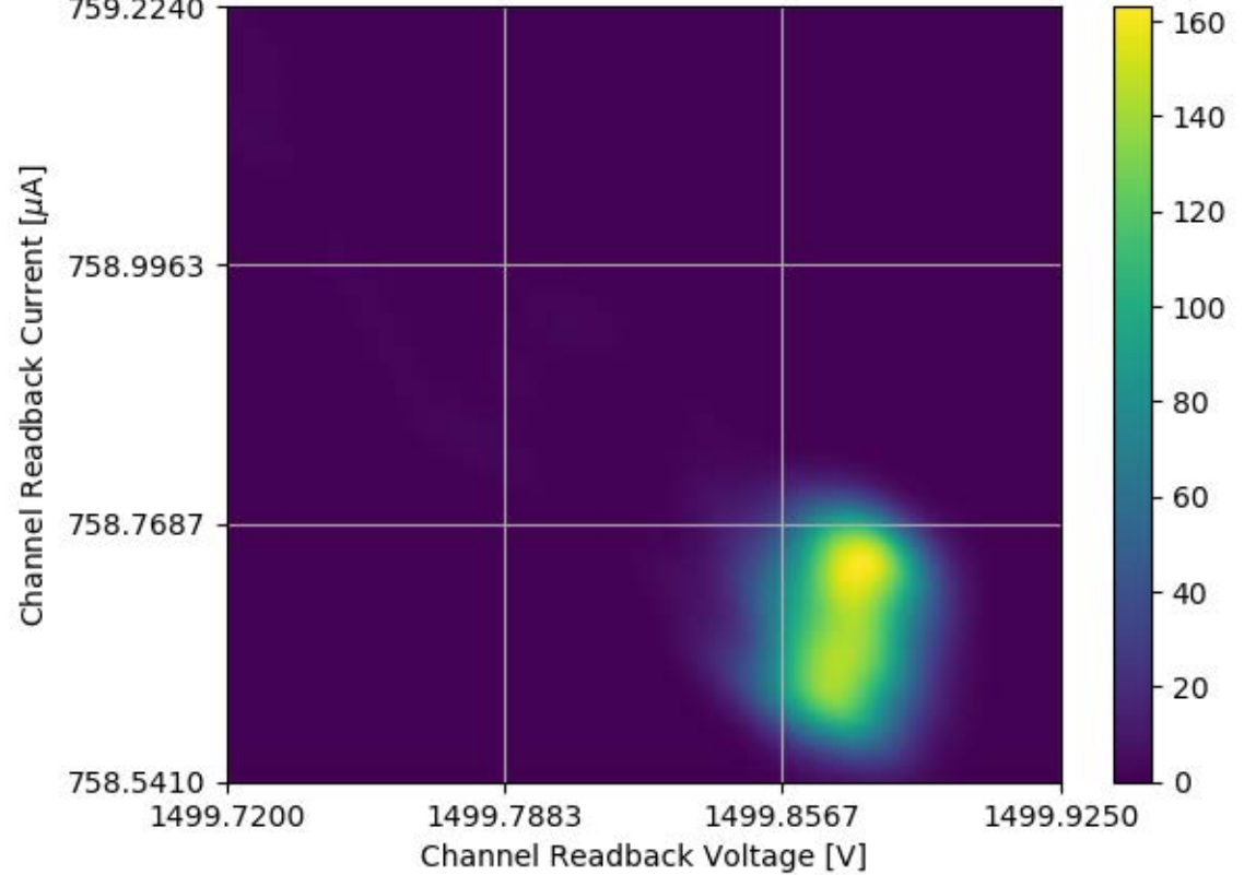
Voltage and Current Readback for Module #304 Channel 22 Stability Test
