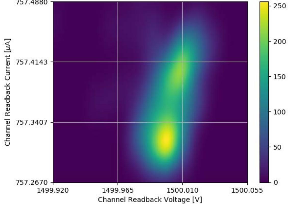
Voltage and Current Readback for Module #304 Channel 27 Stability Test
