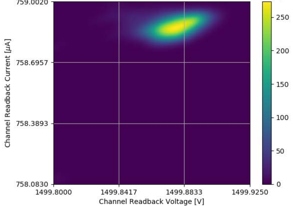
Voltage and Current Readback for Module #304 Channel 10 Stability Test
