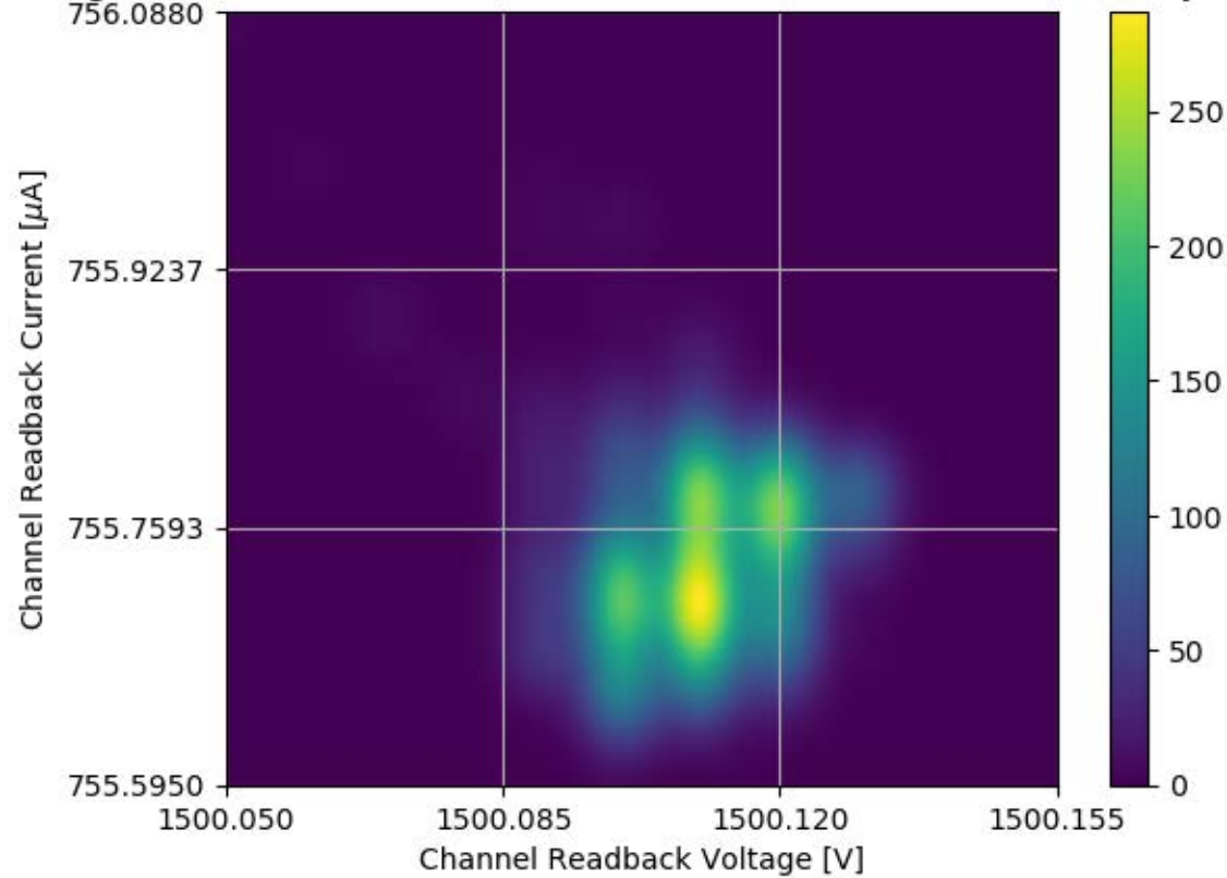
Voltage and Current Readback for Module #304 Channel 28 Stability Test
