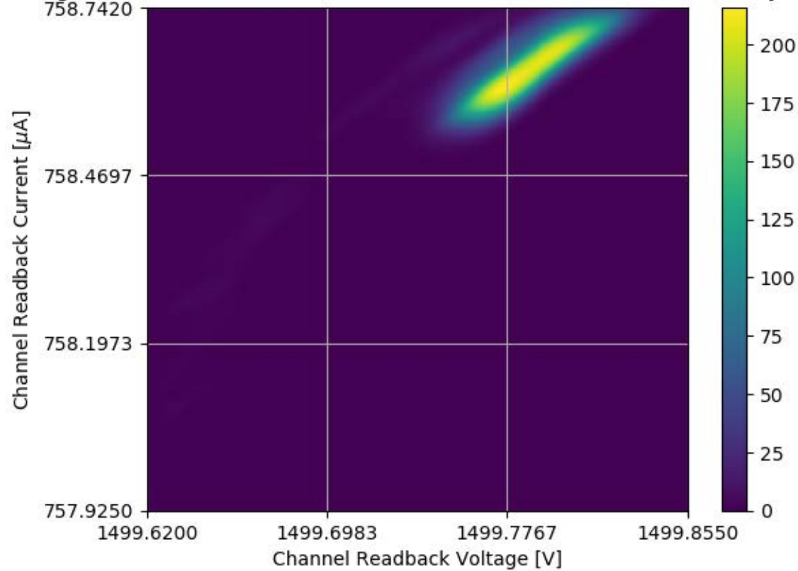
Voltage and Current Readback for Module #304 Channel 24 Stability Test
