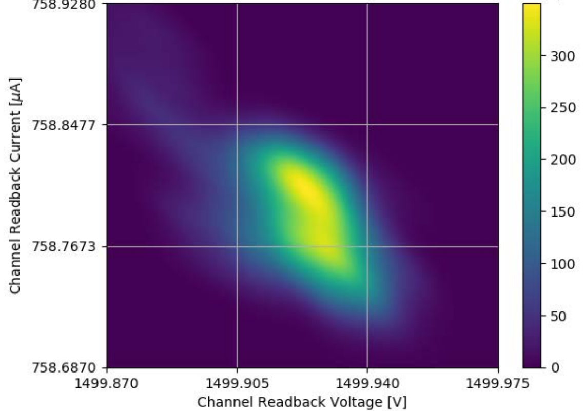
Voltage and Current Readback for Module #304 Channel 19 Stability Test
