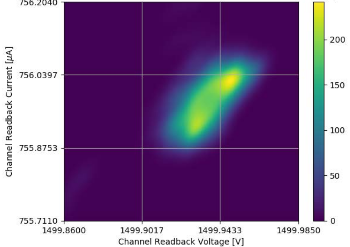
Voltage and Current Readback for Module #304 Channel 31 Stability Test
