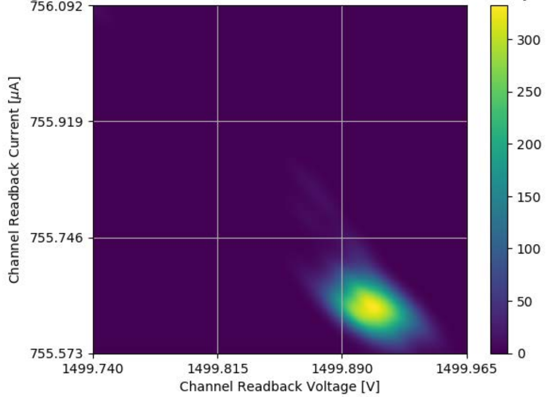
Voltage and Current Readback for Module #304 Channel 01 Stability Test
