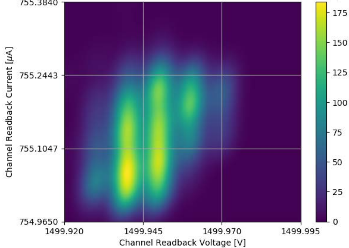
Voltage and Current Readback for Module #304 Channel 17 Stability Test
