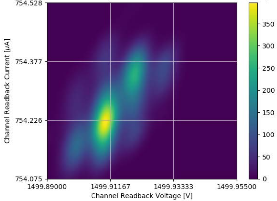
Voltage and Current Readback for Module #304 Channel 30 Stability Test
