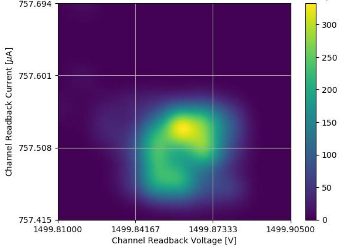
Voltage and Current Readback for Module #304 Channel 21 Stability Test
