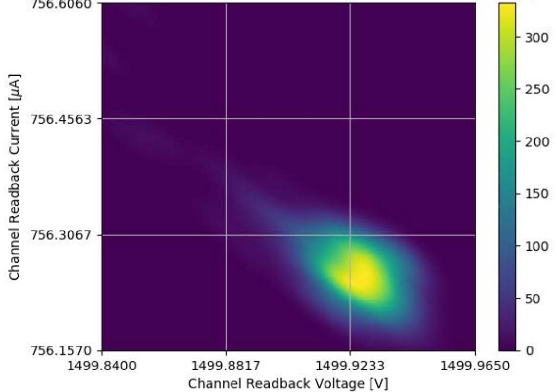
Voltage and Current Readback for Module #304 Channel 18 Stability Test
