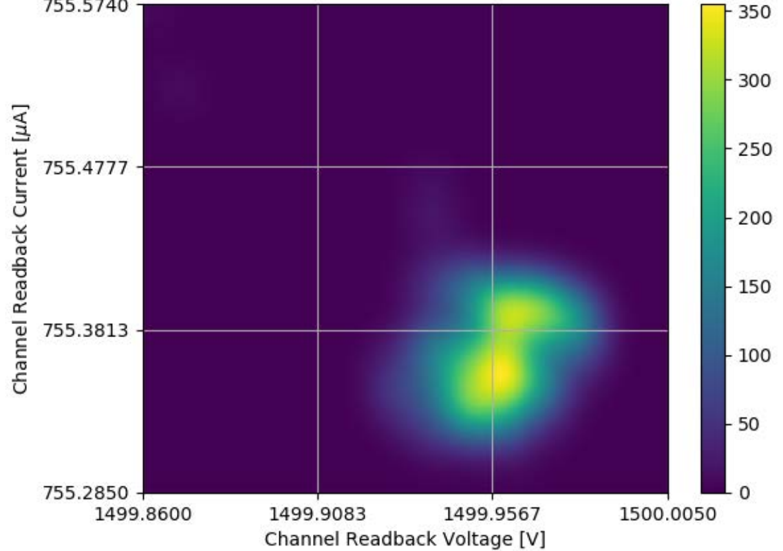
Voltage and Current Readback for Module #304 Channel 00 Stability Test
