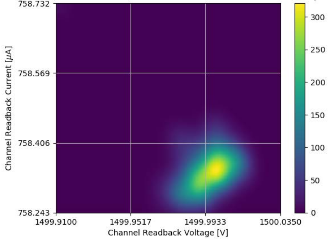
Voltage and Current Readback for Module #304 Channel 05 Stability Test
