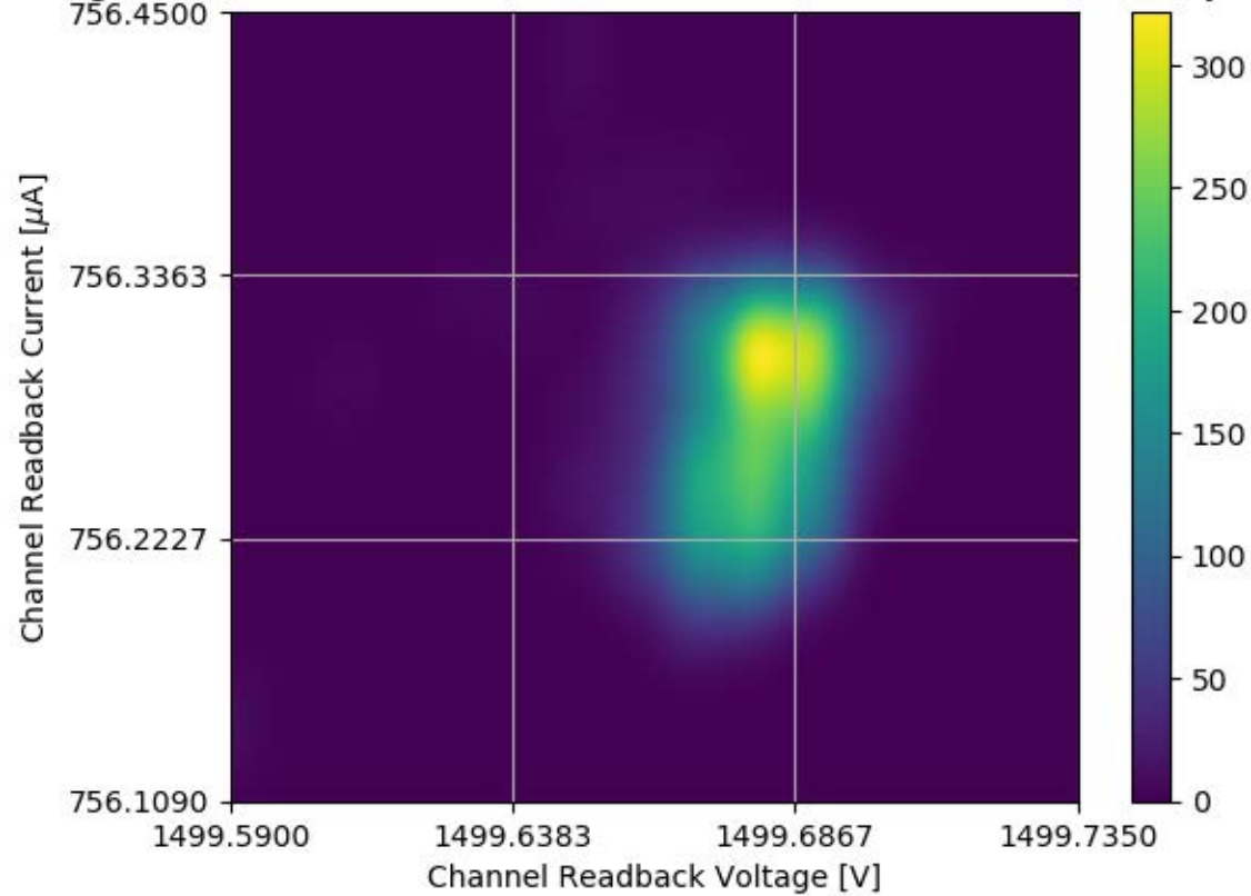
Voltage and Current Readback for Module #304 Channel 11 Stability Test
