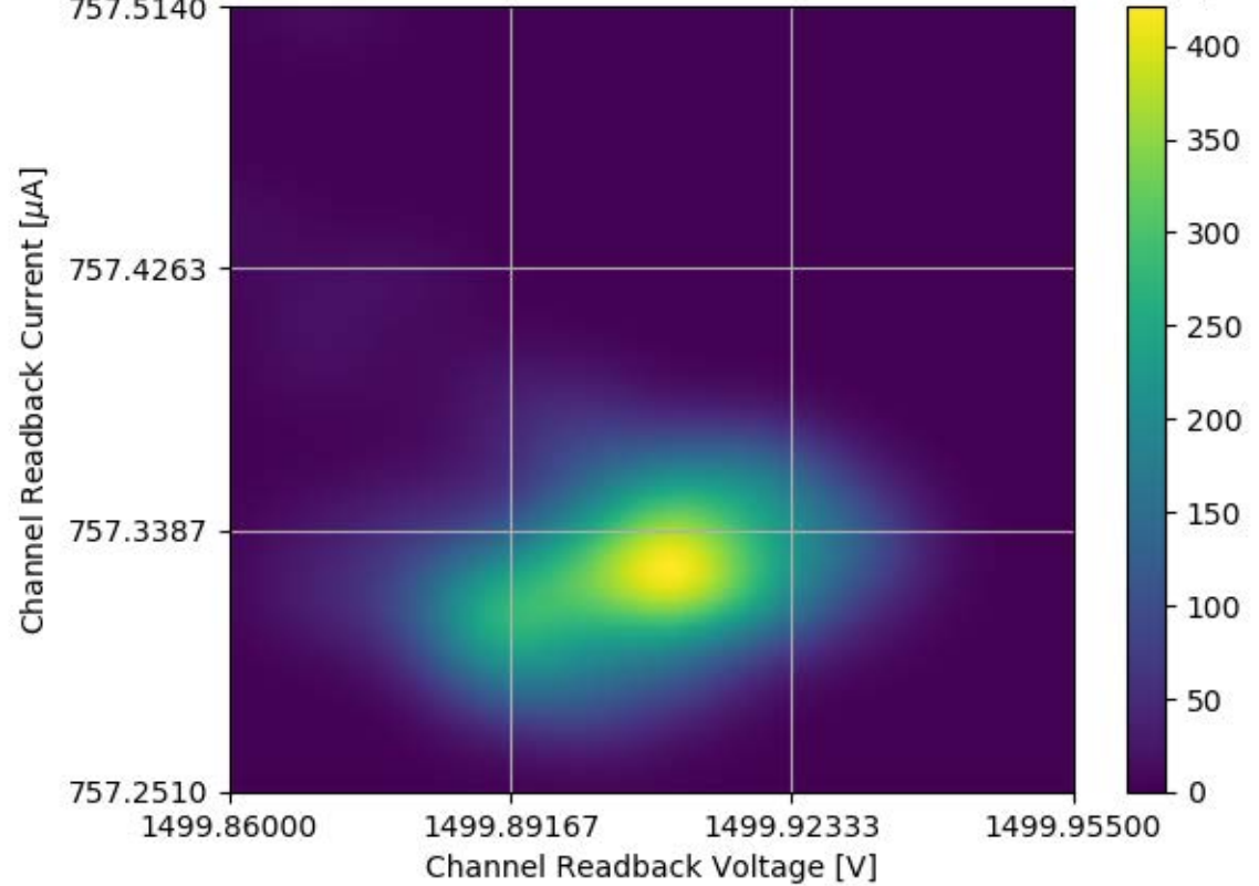
Voltage and Current Readback for Module #304 Channel 07 Stability Test
