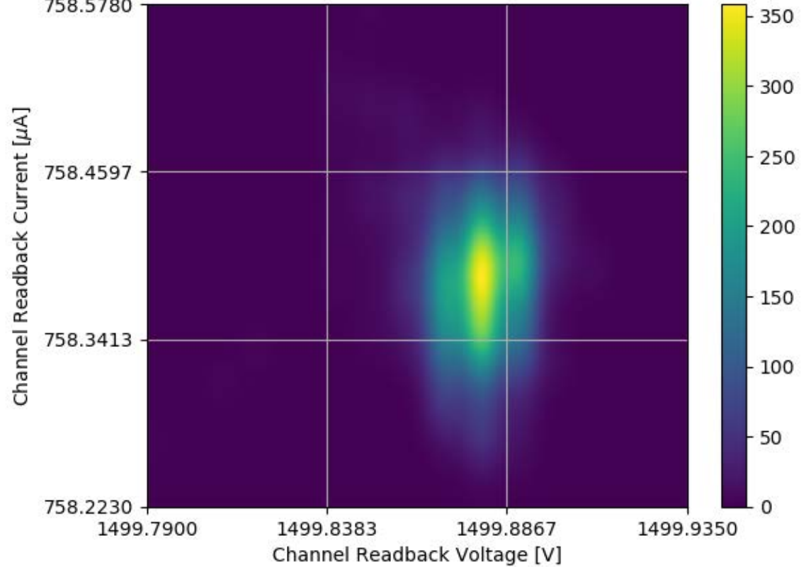
Voltage and Current Readback for Module #304 Channel 04 Stability Test
