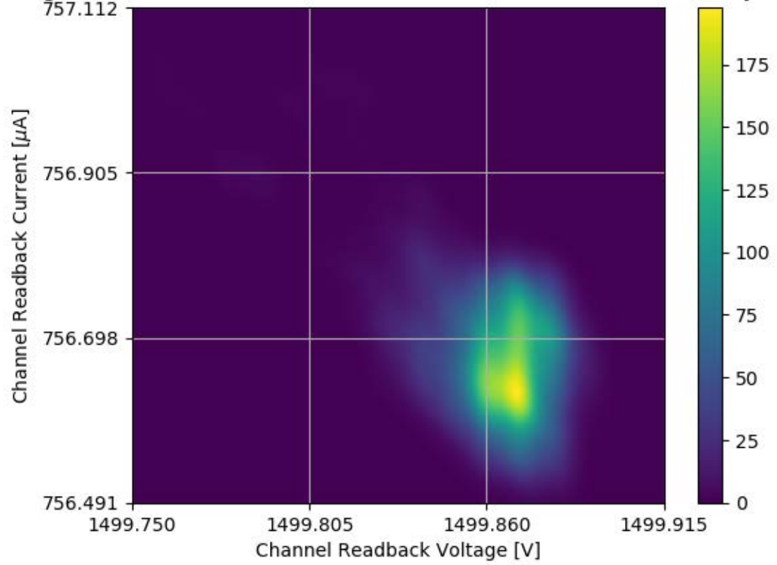
Voltage and Current Readback for Module #304 Channel 29 Stability Test
