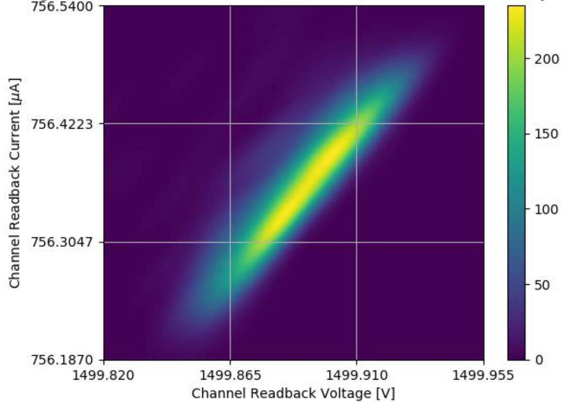
Voltage and Current Readback for Module #304 Channel 20 Stability Test
