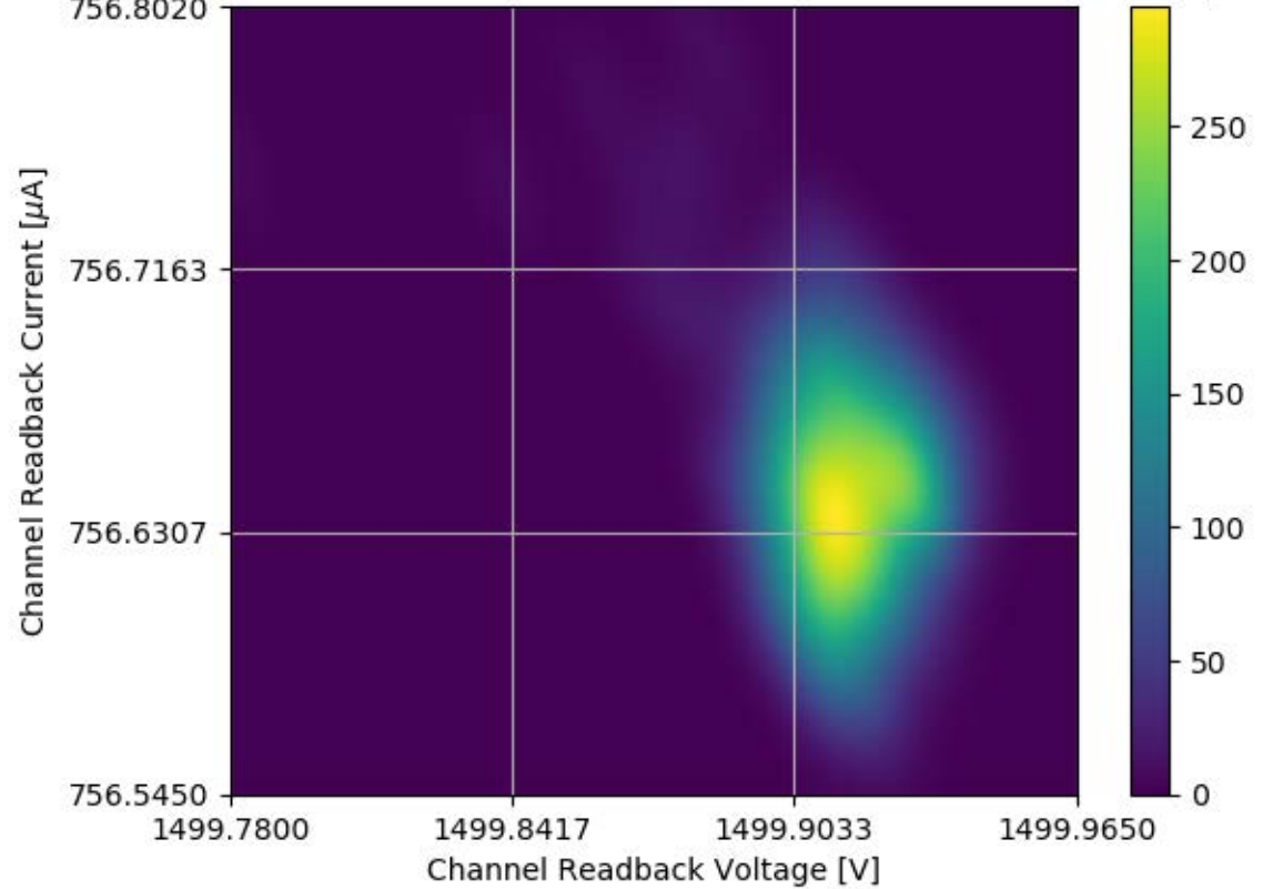
Voltage and Current Readback for Module #304 Channel 02 Stability Test
