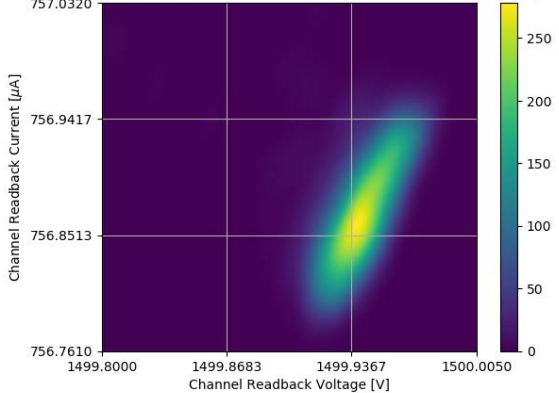
Voltage and Current Readback for Module #304 Channel 32 Stability Test
