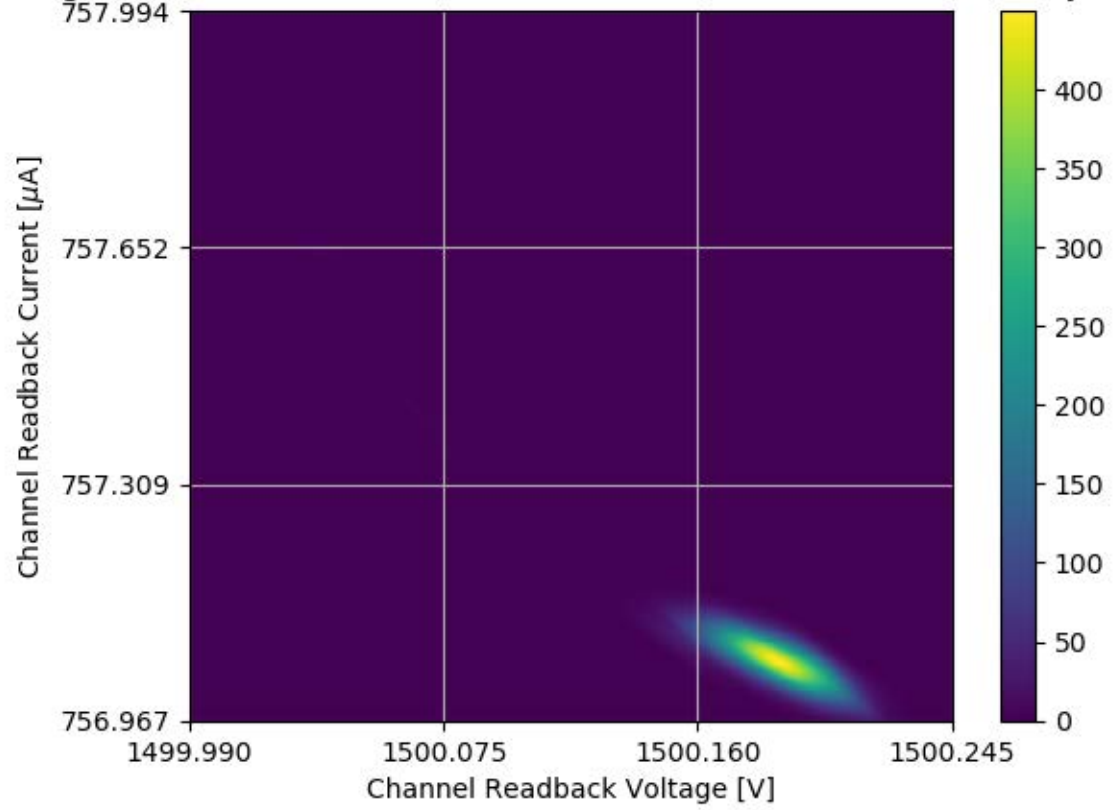
Voltage and Current Readback for Module #309 Channel 19 Stability Test
