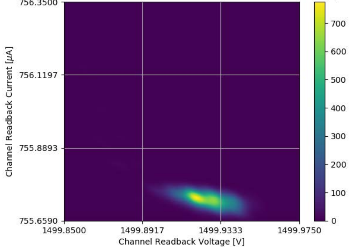
Voltage and Current Readback for Module #309 Channel 01 Stability Test
