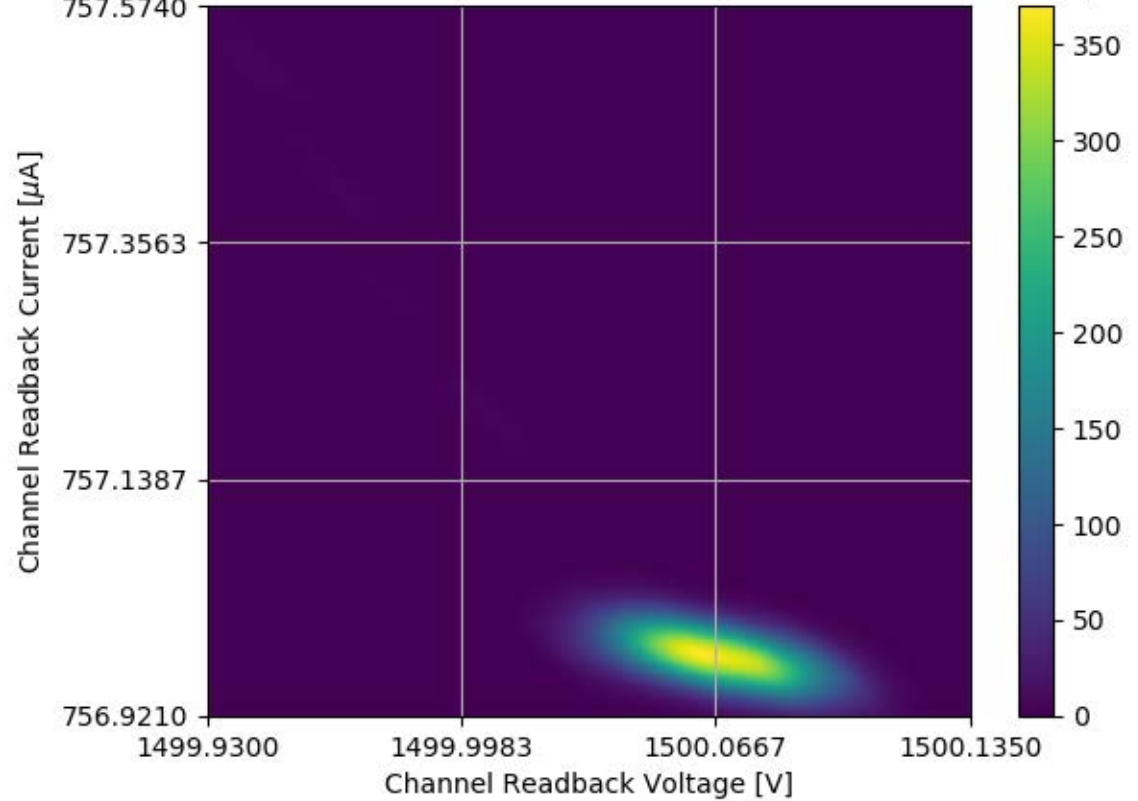
Voltage and Current Readback for Module #309 Channel 29 Stability Test
