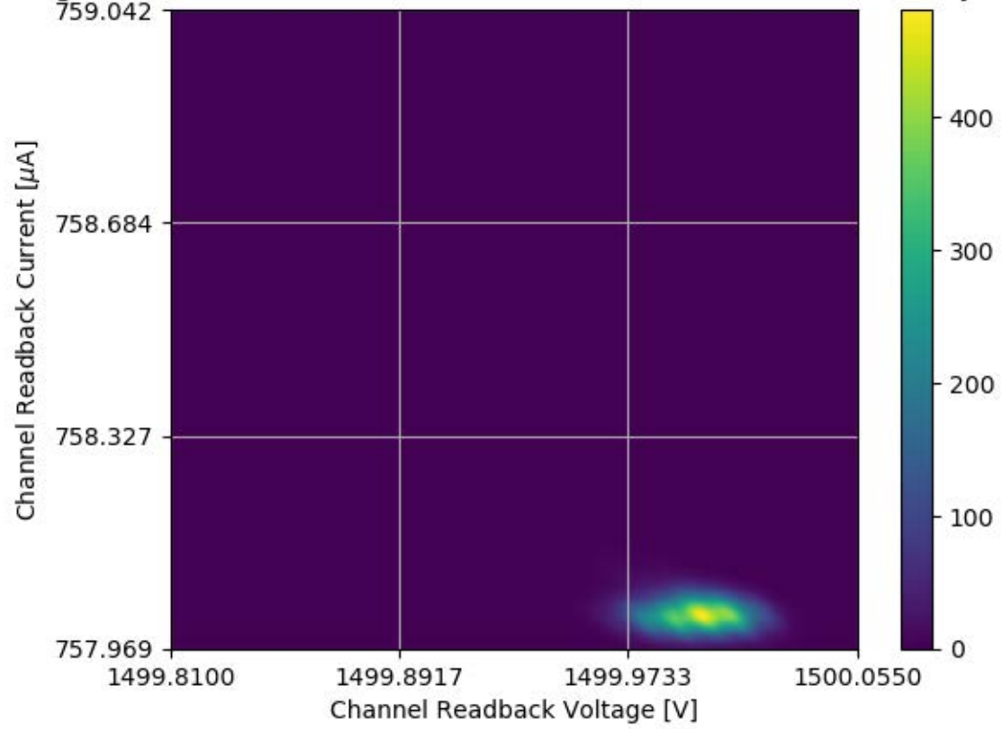
Voltage and Current Readback for Module #309 Channel 05 Stability Test
