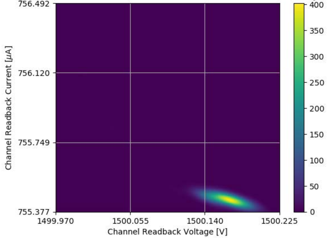
Voltage and Current Readback for Module #309 Channel 03 Stability Test
