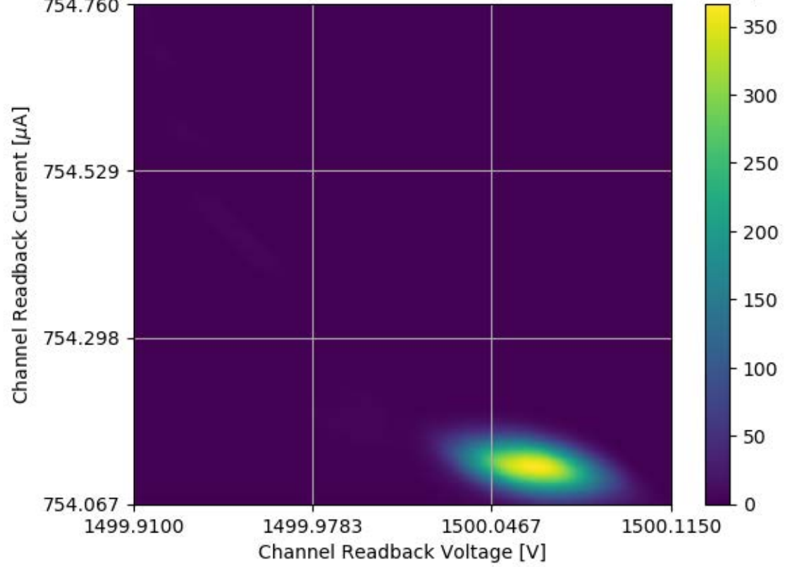
Voltage and Current Readback for Module #309 Channel 00 Stability Test
