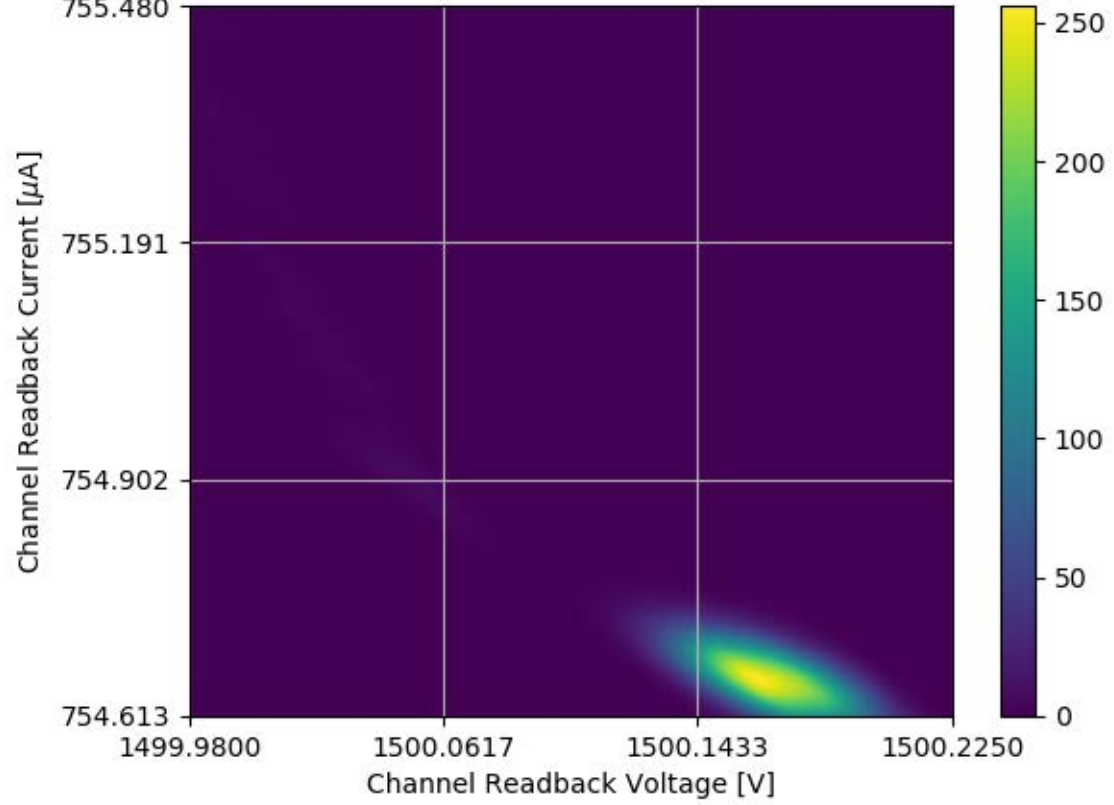
Voltage and Current Readback for Module #309 Channel 13 Stability Test
