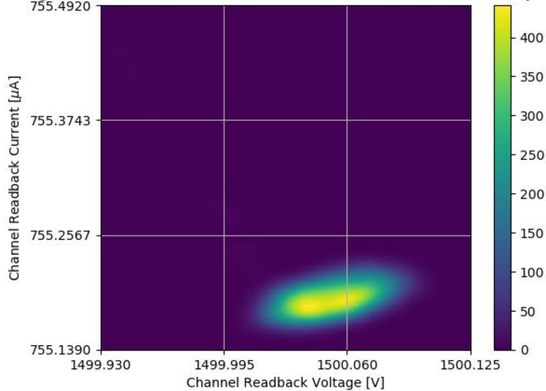
Voltage and Current Readback for Module #309 Channel 30 Stability Test
