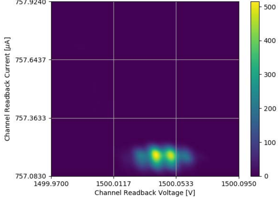
Voltage and Current Readback for Module #309 Channel 23 Stability Test
