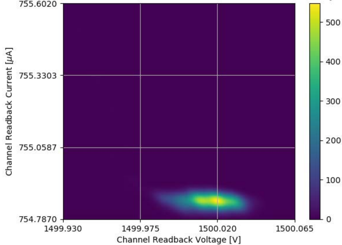
Voltage and Current Readback for Module #309 Channel 14 Stability Test
