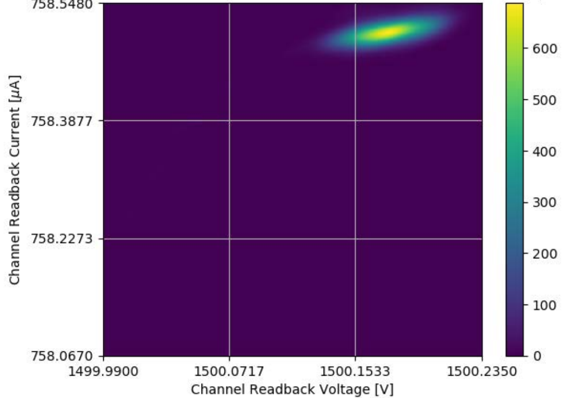
Voltage and Current Readback for Module #309 Channel 08 Stability Test
