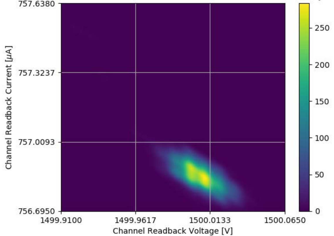
Voltage and Current Readback for Module #309 Channel 20 Stability Test
