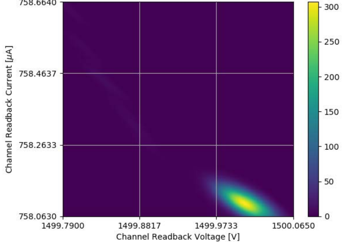
Voltage and Current Readback for Module #309 Channel 04 Stability Test
