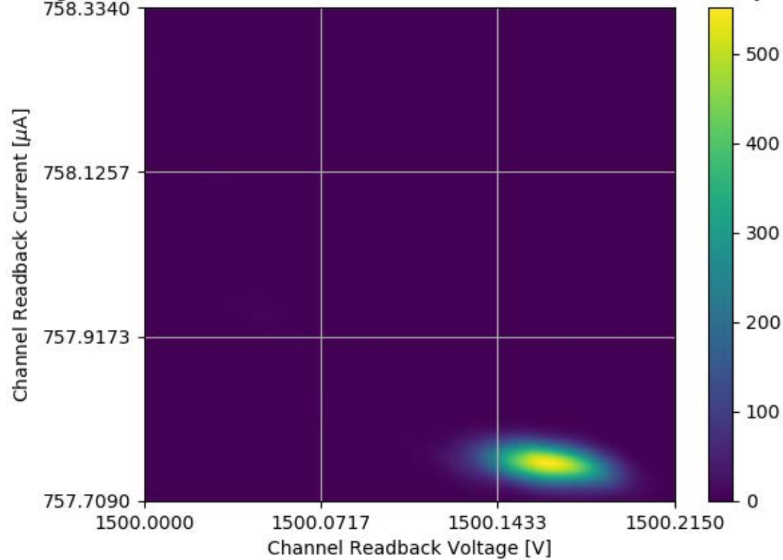
Voltage and Current Readback for Module #309 Channel 06 Stability Test
