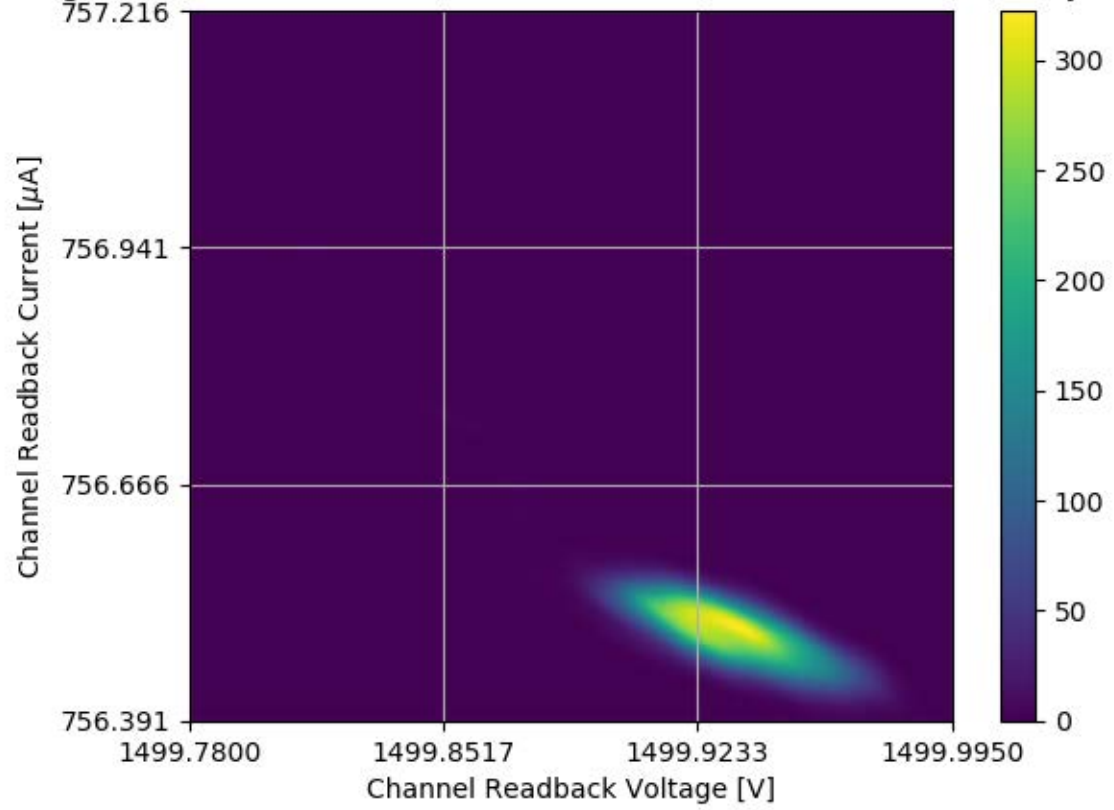
Voltage and Current Readback for Module #309 Channel 27 Stability Test
