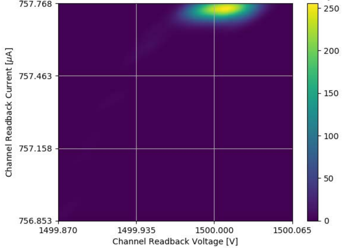
Voltage and Current Readback for Module #309 Channel 26 Stability Test
