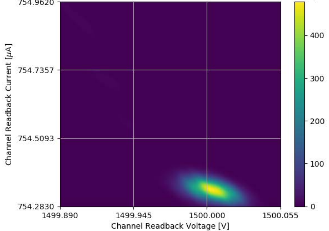
Voltage and Current Readback for Module #309 Channel 33 Stability Test
