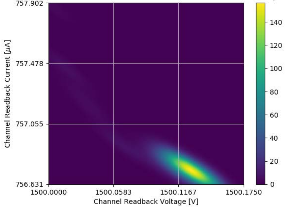
Voltage and Current Readback for Module #313 Channel 18 Stability Test
