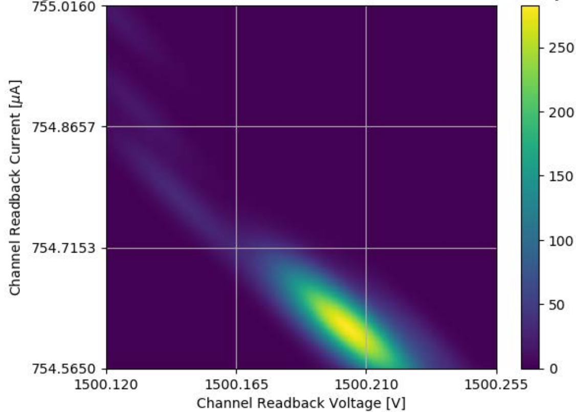
Voltage and Current Readback for Module #313 Channel 00 Stability Test
