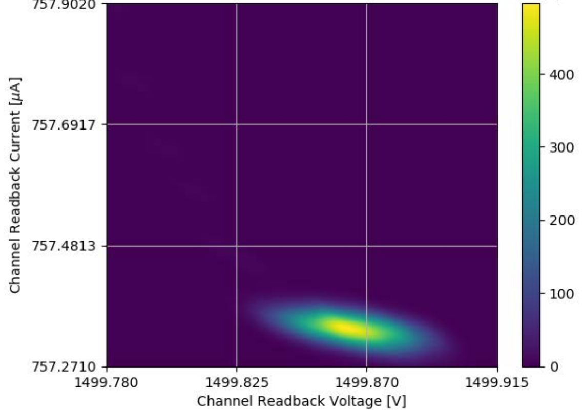
Voltage and Current Readback for Module #313 Channel 16 Stability Test
