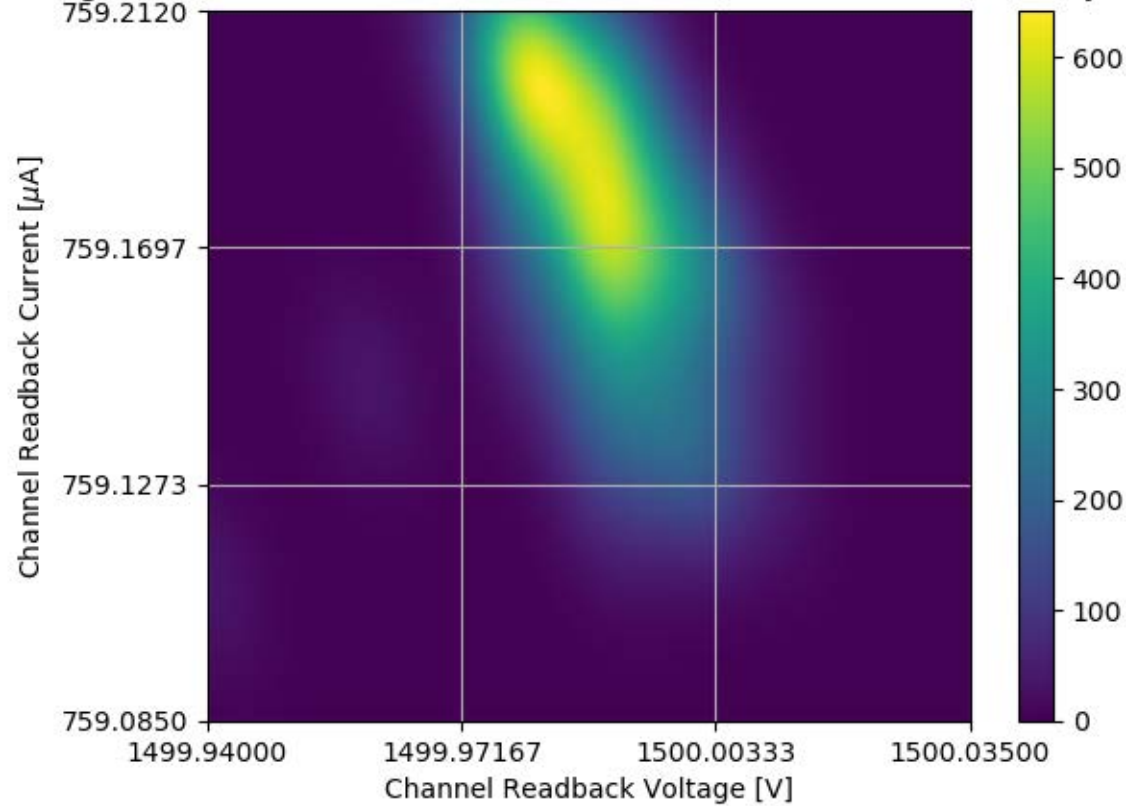
Voltage and Current Readback for Module #313 Channel 25 Stability Test
