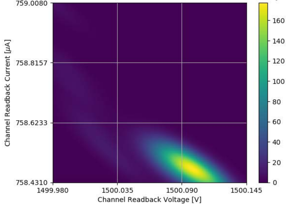
Voltage and Current Readback for Module #313 Channel 05 Stability Test
