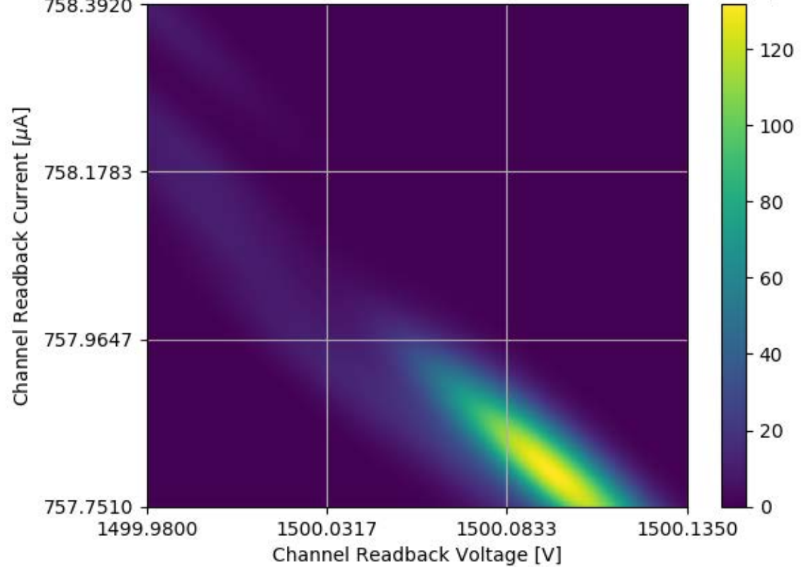
Voltage and Current Readback for Module #313 Channel 06 Stability Test
