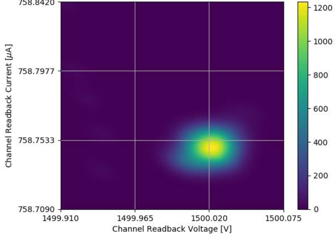
Voltage and Current Readback for Module #313 Channel 12 Stability Test
