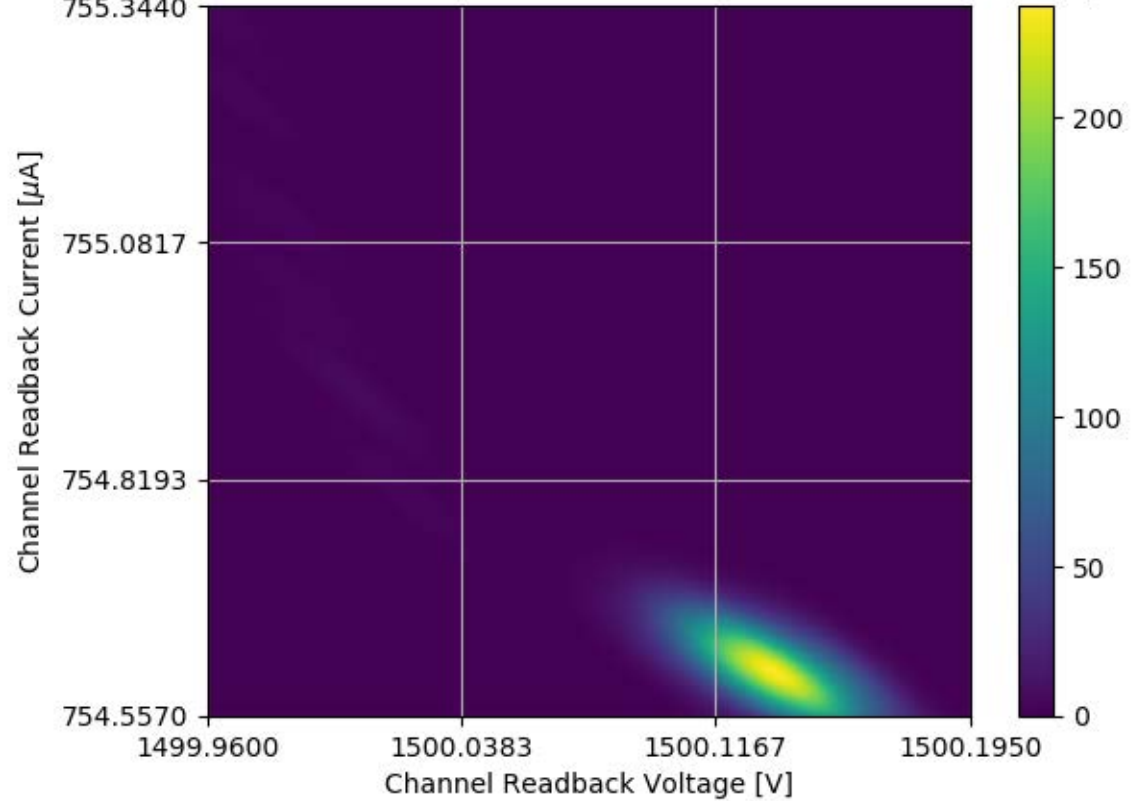
Voltage and Current Readback for Module #313 Channel 13 Stability Test
