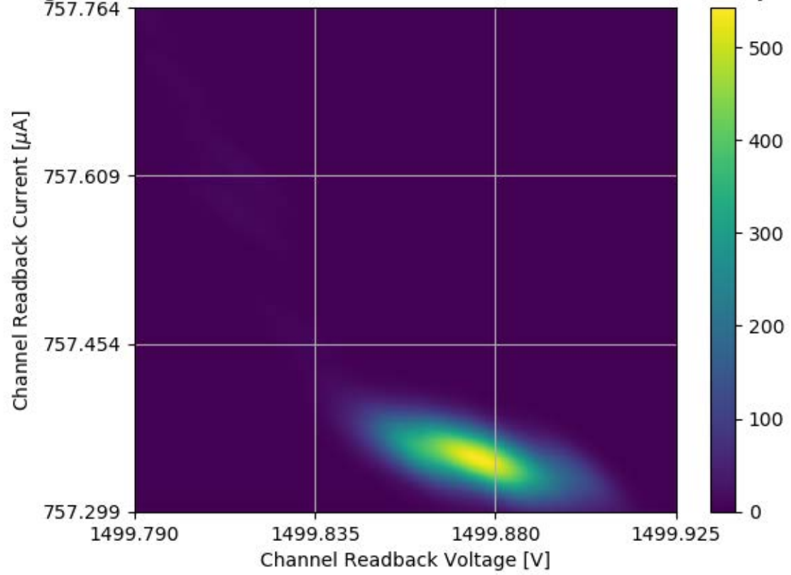
Voltage and Current Readback for Module #313 Channel 35 Stability Test
