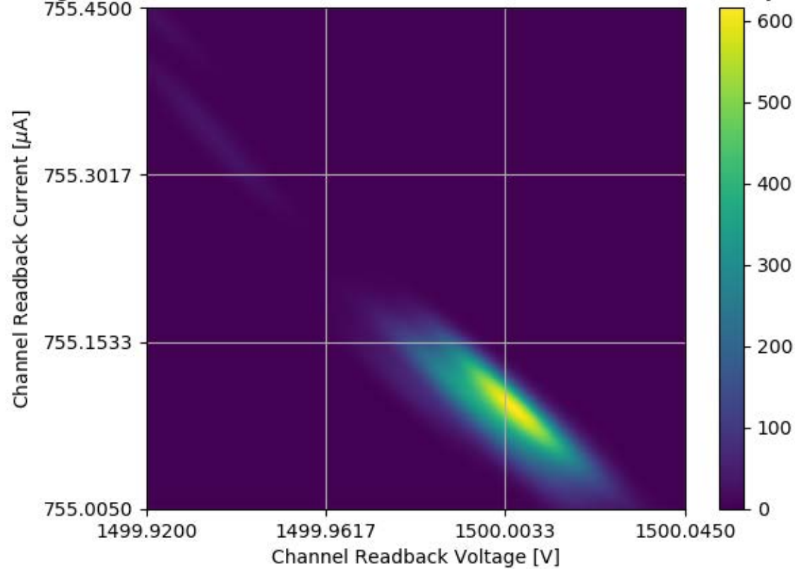
Voltage and Current Readback for Module #313 Channel 30 Stability Test
