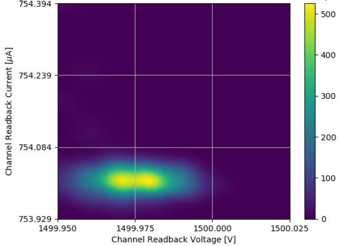
Voltage and Current Readback for Module #313 Channel 33 Stability Test
