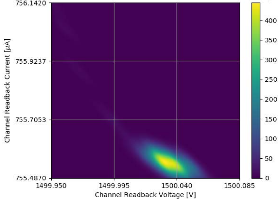
Voltage and Current Readback for Module #313 Channel 17 Stability Test
