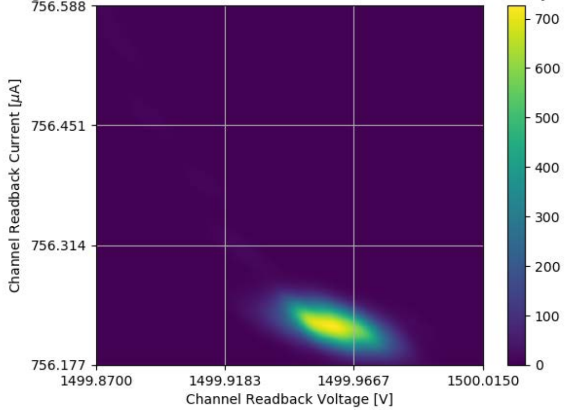
Voltage and Current Readback for Module #313 Channel 23 Stability Test
