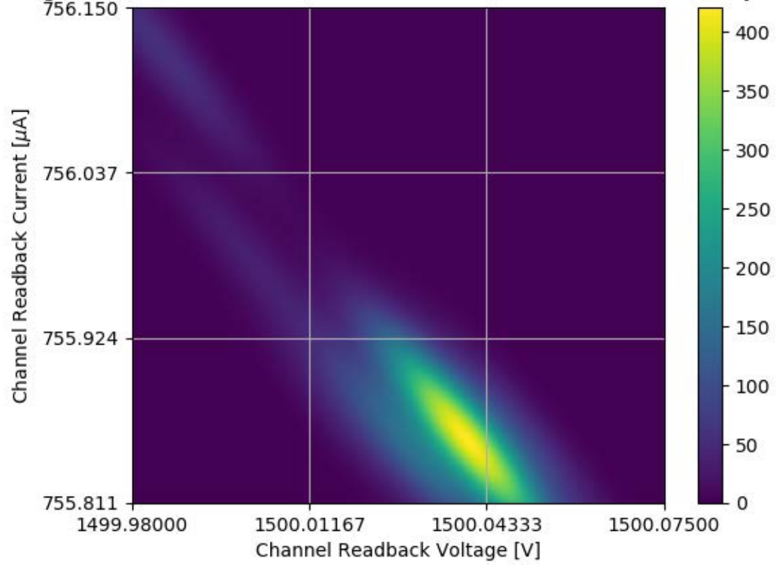
Voltage and Current Readback for Module #313 Channel 15 Stability Test
