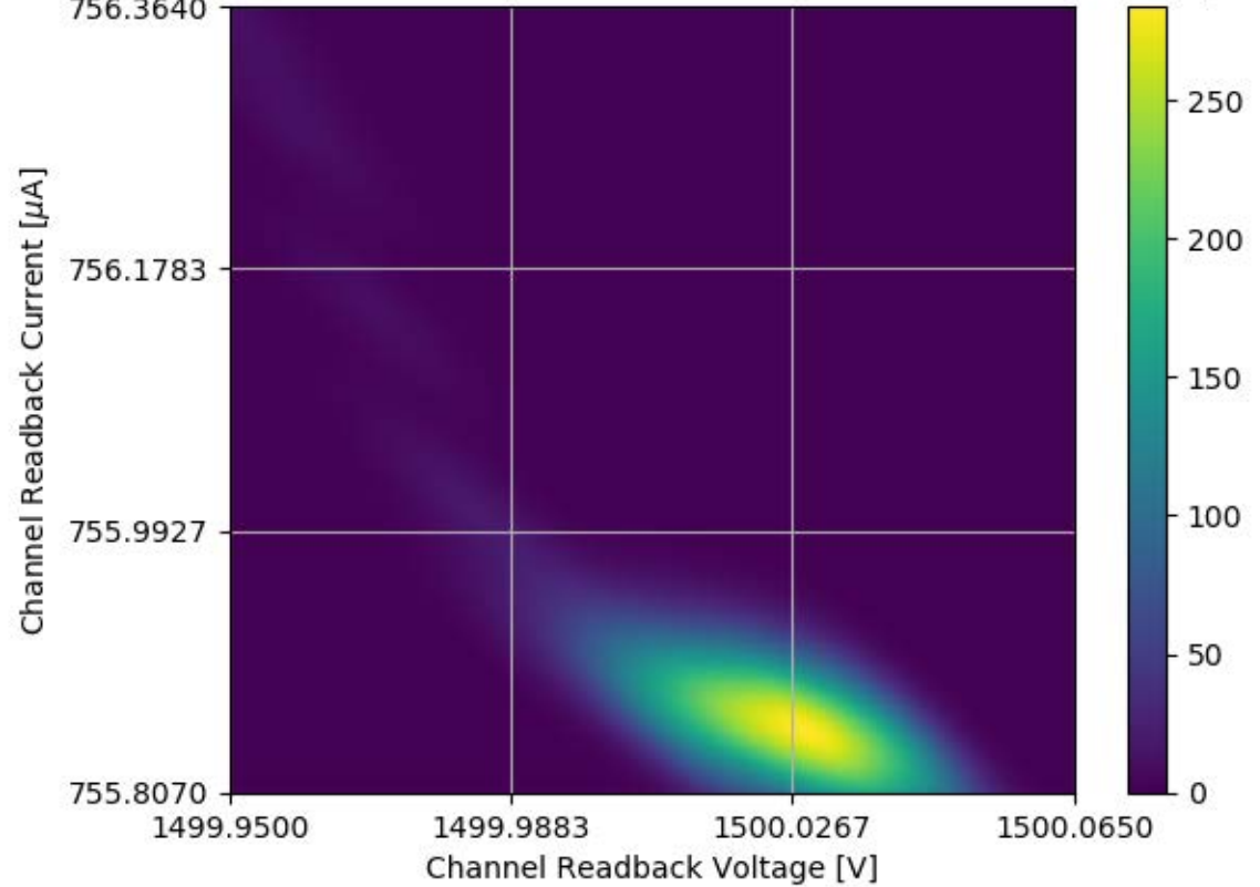
Voltage and Current Readback for Module #313 Channel 31 Stability Test
