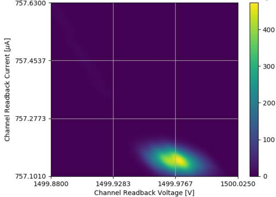
Voltage and Current Readback for Module #313 Channel 21 Stability Test
