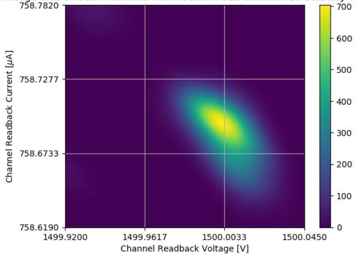
Voltage and Current Readback for Module #313 Channel 10 Stability Test
