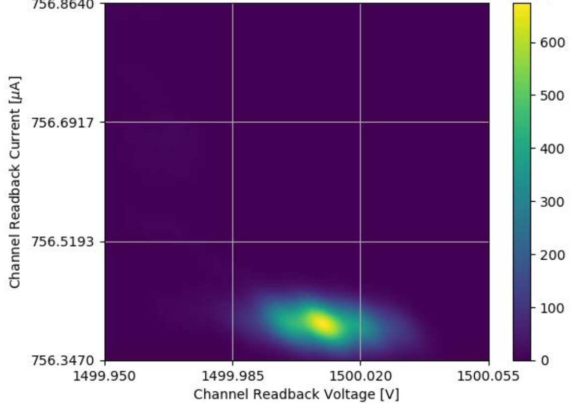
Voltage and Current Readback for Module #313 Channel 27 Stability Test
