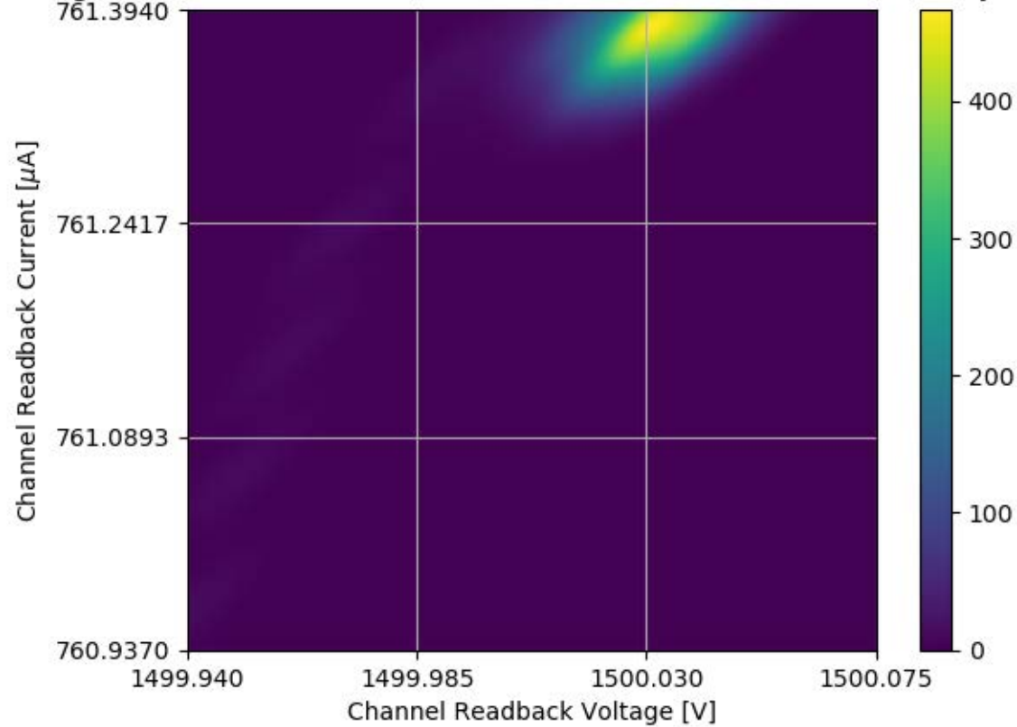
Voltage and Current Readback for Module #313 Channel 09 Stability Test
