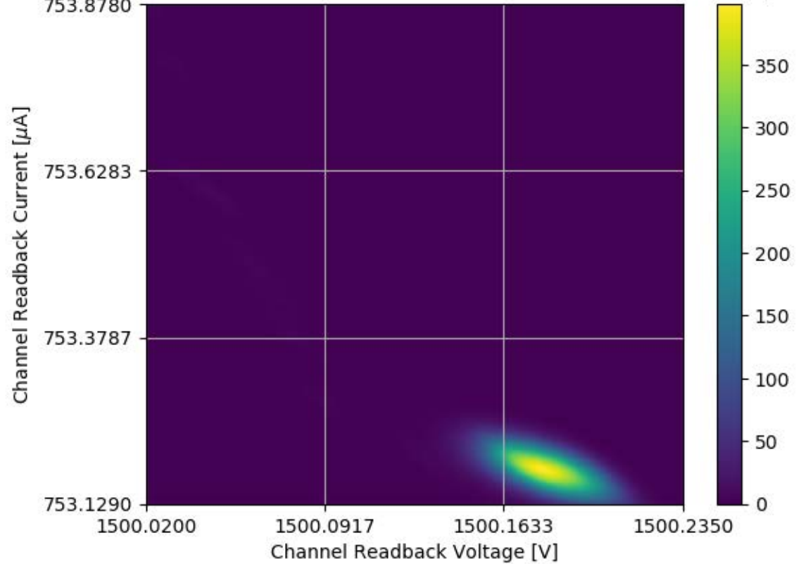
Voltage and Current Readback for Module #313 Channel 11 Stability Test
