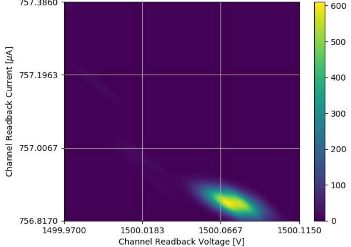
Voltage and Current Readback for Module #313 Channel 19 Stability Test
