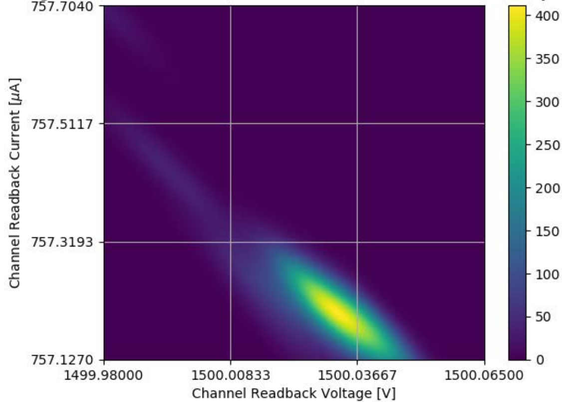
Voltage and Current Readback for Module #313 Channel 20 Stability Test
