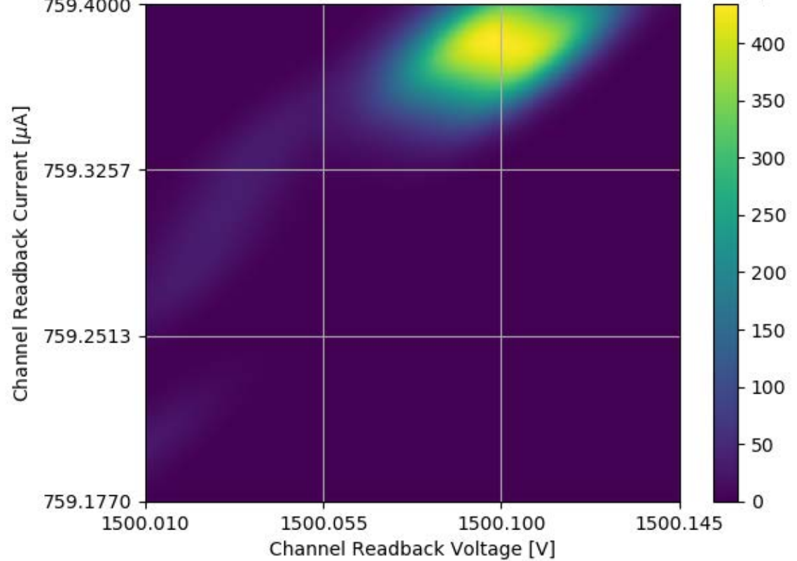
Voltage and Current Readback for Module #313 Channel 24 Stability Test
